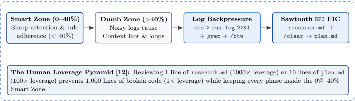
Figure 4: Context Window Physics: keeping utilization inside the 0%–40% Smart Zone via output-redirection backpressure, Sawtooth RPI Intentional Compaction, and the Human Leverage Pyramid [12, 18].
