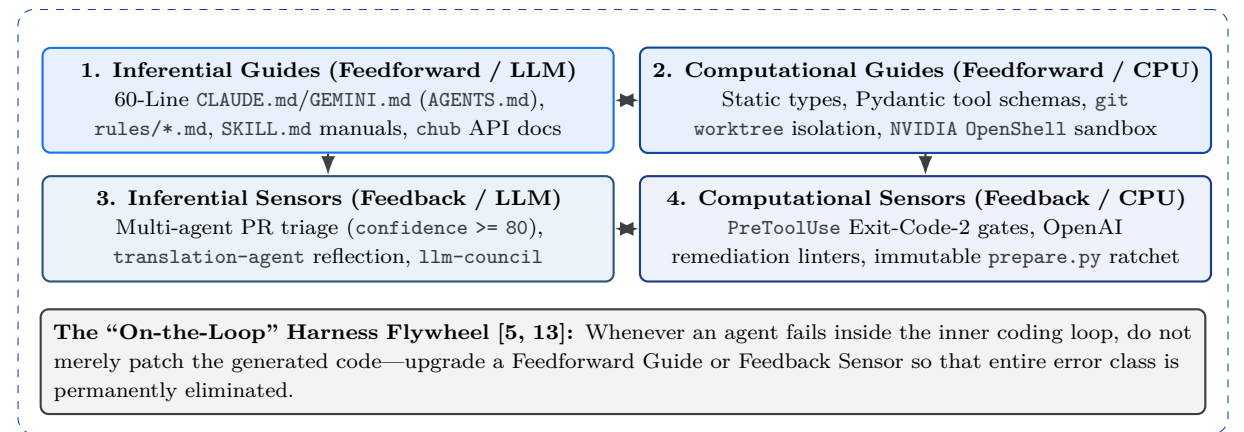
Figure 5: The 2×2 Cybernetic Control Matrix mapping Feedforward Guides and Feedback Sensors across deterministic CPU checks and semantic LLM reasoning [13].
