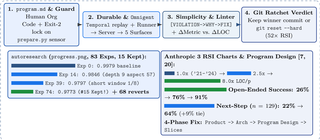
Figure 10: Layer 4 Autonomous Loops & Meta-Harnesses: the autoresearch 83-experiment step-down ratchet (0.9979 → 0.9773 [18]), Databricks Omnigent [20], and Anthropic’s 3 RSI charts (8.0× quarterly LOC/person, 26%→91% open-ended success, and 64% next-step win rate [7]).
