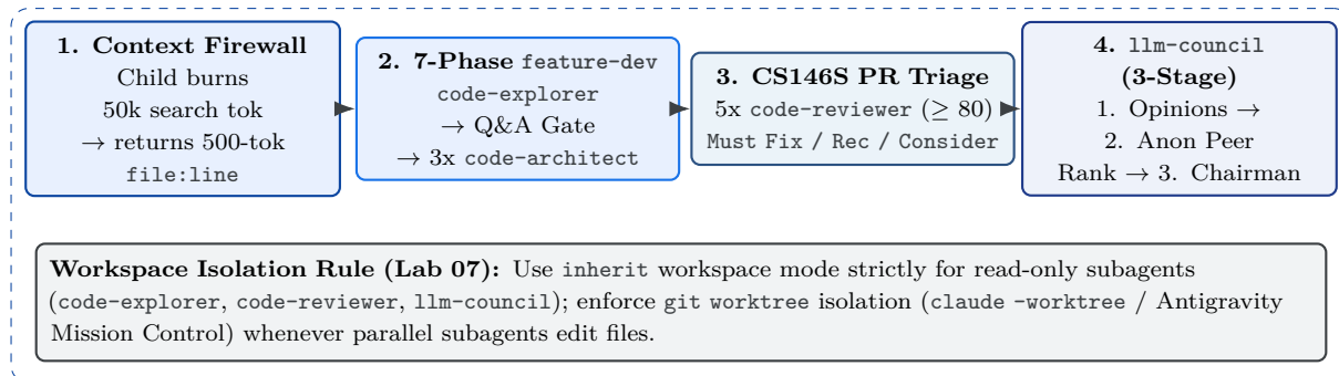
Figure 5.1 Blueprint: Subagent Firewalls, PR Triage &amp; llm-council
