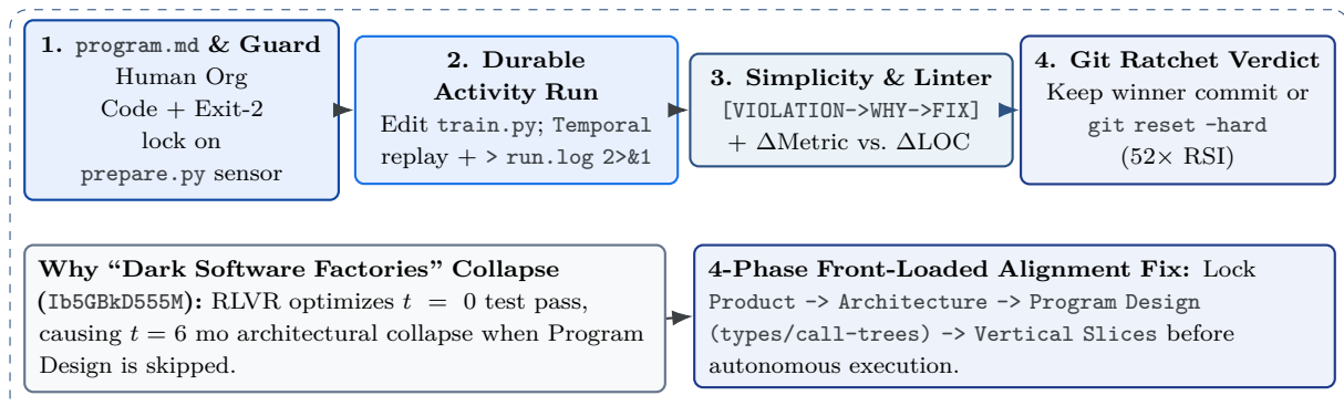
Figure 5.2 Blueprint: Autoresearch Ratchet, Governance & Program Design
