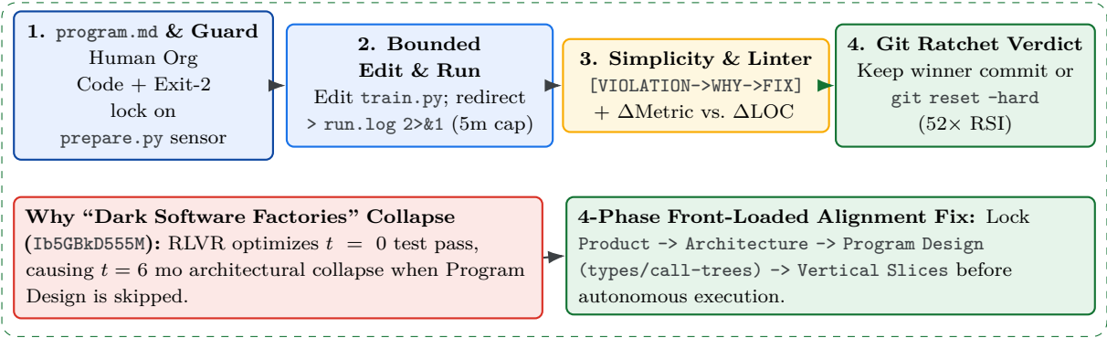
Figure 10: Layer 4 Autonomous Loops & Governance: Karpathy’s autoresearch (program.md) keep-or-revert ratchet, OpenAI remediation linters, and Horthy’s 4-Phase Front-Loaded Program Design preventing “Dark Factory” collapse.
