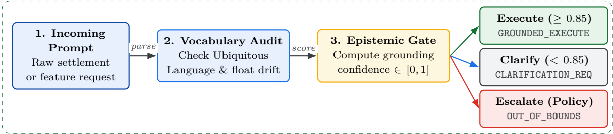
Figure 2: Bounding an agent inside an explicit Engineering Language Game with Ubiquitous Language types and a 3-way Epistemic Confidence Gate (Lab 01).
