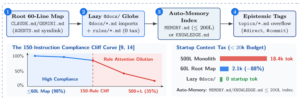
Figure 3.2 Blueprint: 150-Instruction Compliance Cliff Curve, 60-Line Map & Auto-Memory
