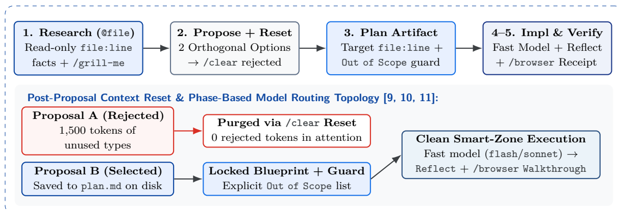
Figure 2.1 Blueprint: The 5-Step RePPIT Workflow & Post-Proposal Context Reset
