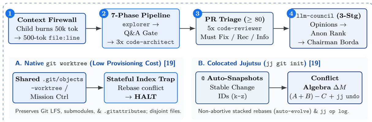
Figure 5.1 Blueprint: Subagent Firewalls, PR Triage, llm-council &amp; git worktree / Jujutsu (jj)
