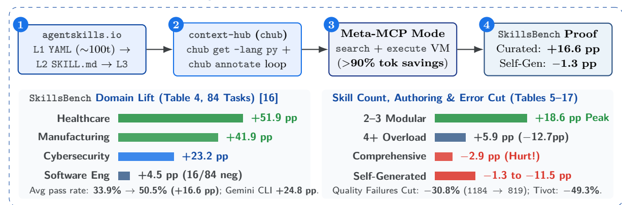
Figure 4.1 Blueprint: 3-Level agentskills.io , chub , Meta-MCP & SkillsBench Charts
