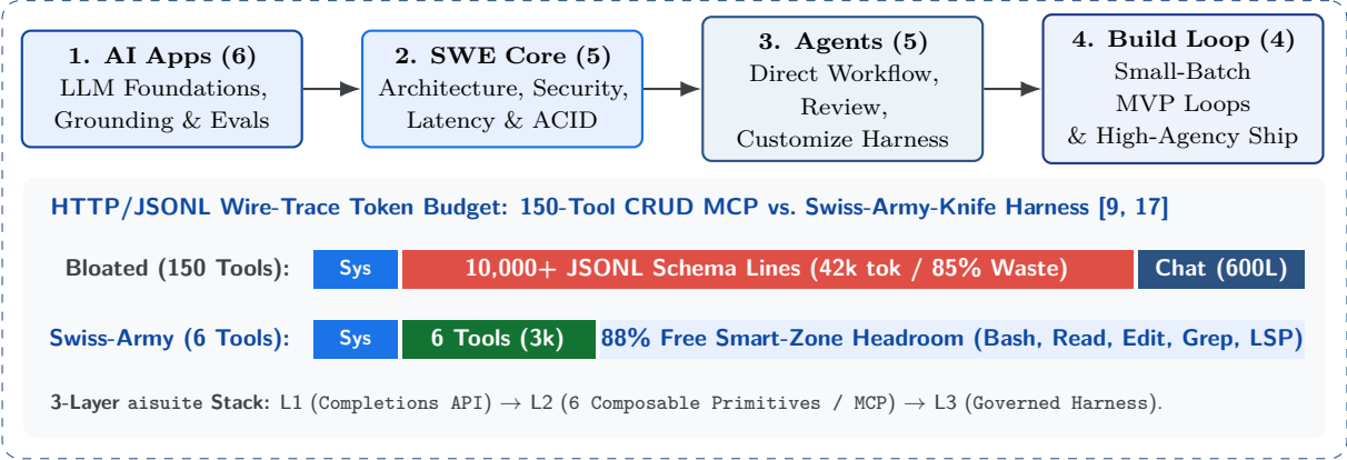
Figure 3: The 4-Pillar AI Engineering Skills Map [5], the aisuite 3-Layer Agent Stack [17], and HTTP/JSONL wire-trace token breakdown contrasting Swiss-Army-Knife primitives against 150-tool schema bloat [9].
