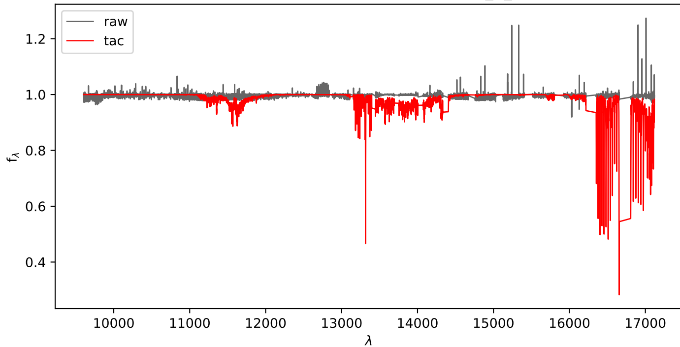
car-20190702T20h55m20s-sci-amap-nir_A_s1d.fits
