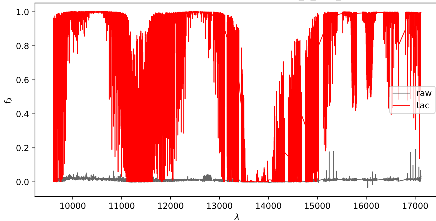
car-20190702T20h55m20s-sci-amap-nir_A_S1D_NIR.fits
