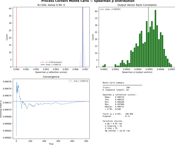
Fig. 1. Process-corners Monte Carlo histogram ( N = 500 ) showing Spearman \rho distribution. Mean \rho = 0.996724 , minimum \rho = 0.996289 , zero trials below 0.99.
