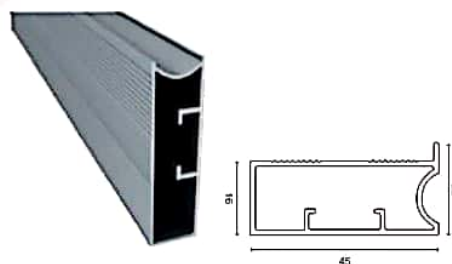
45mm U Framelass Profile
