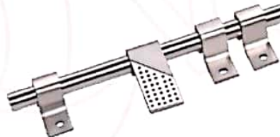
3 mm 20/20 Latch - 12mm Rod
