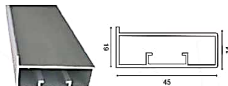
45mm Framelass Profile
