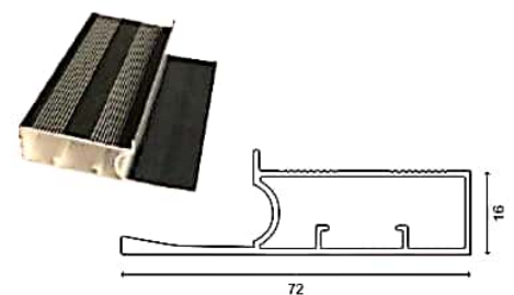
72mm U Handle Framelass Profile
