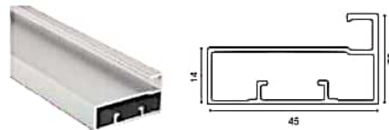
45mm Frame Profile
