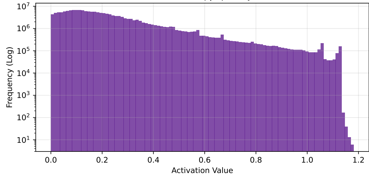
conv3 - Global Freq | Sparsity: 50.0%
