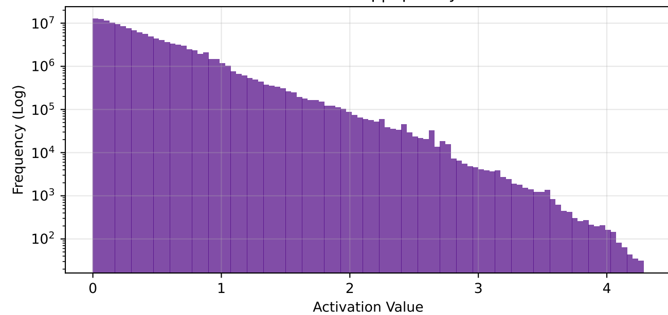
conv3 - Global Freq | Sparsity: 89.0%
