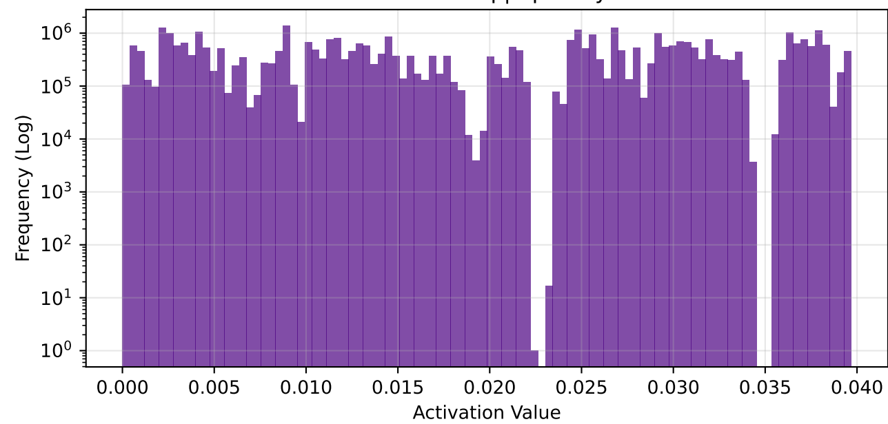
fc1 - Global Freq | Sparsity: 58.6%
