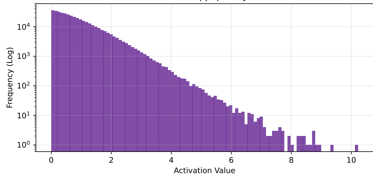
fc1 - Global Freq | Sparsity: 68.7%
