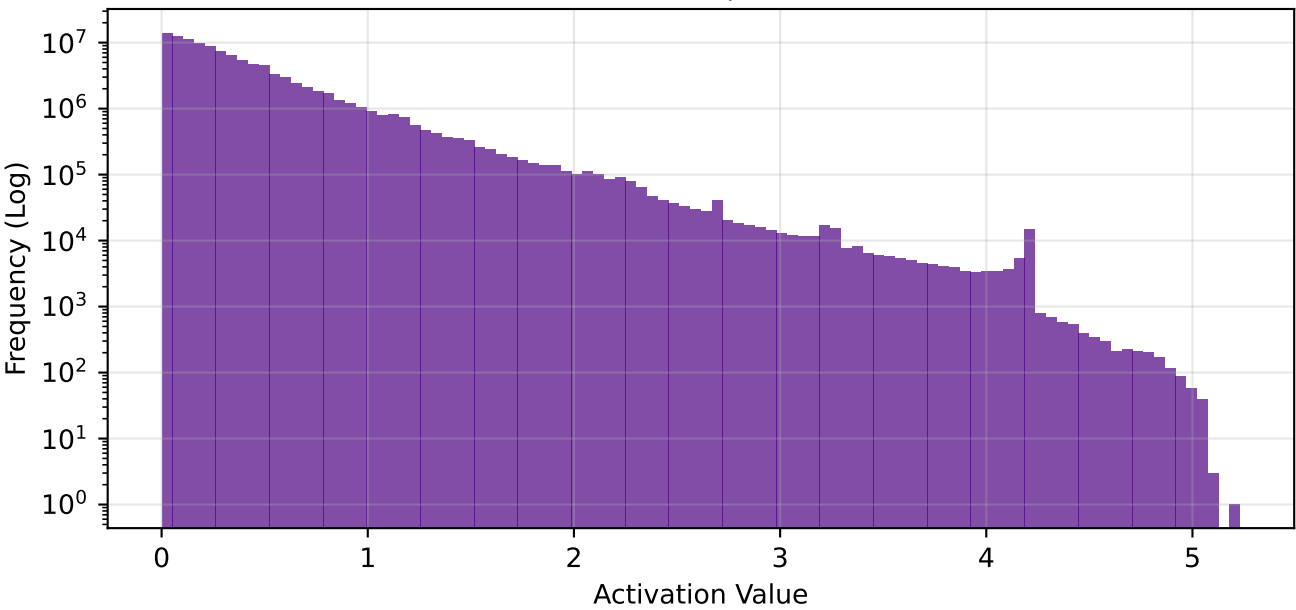
conv3 - Global Freq | Sparsity: 91.4%
