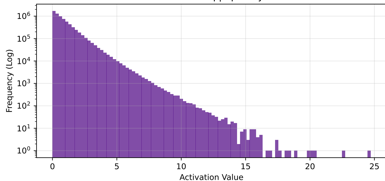
fc1 - Global Freq | Sparsity: 69.9%
