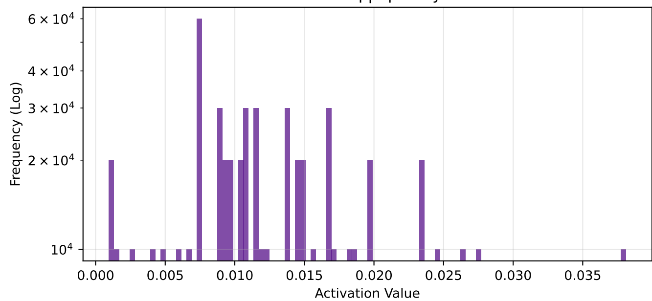
fc1 - Global Freq | Sparsity: 58.6%
