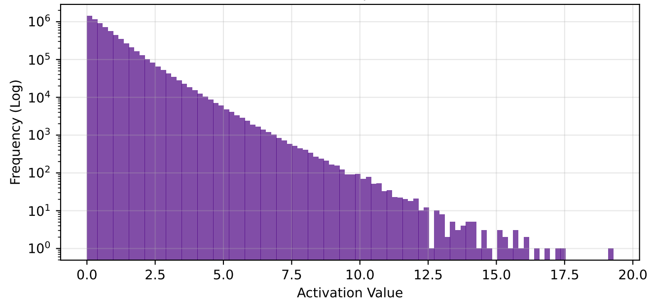
fc1 - Global Freq | Sparsity: 70.4%
