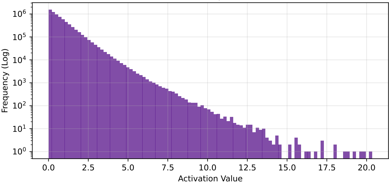
fc1 - Global Freq | Sparsity: 61.3%
