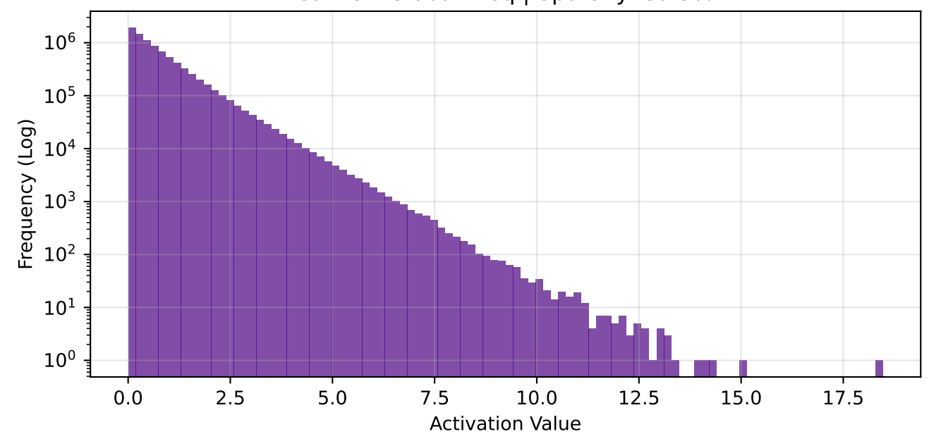
fc1 - Global Freq | Sparsity: 62.3%
