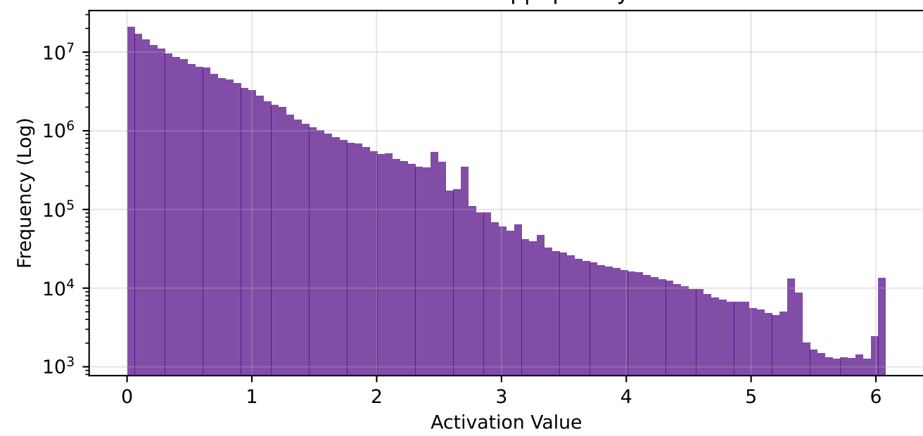
conv3 - Global Freq | Sparsity: 87.1%
