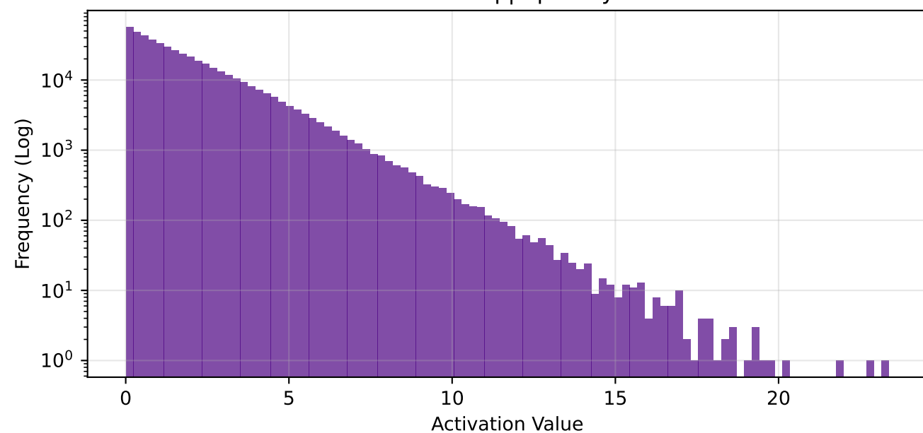
fc1 - Global Freq | Sparsity: 62.1%
