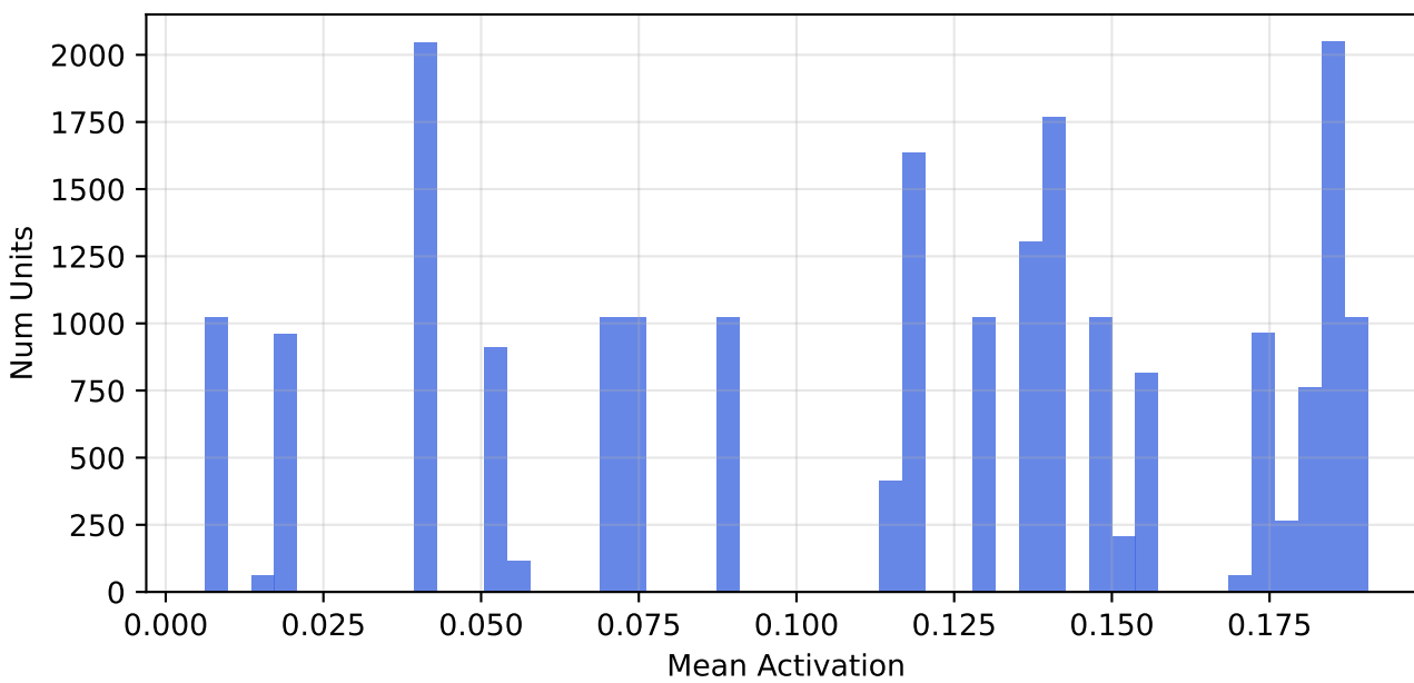
conv3 - Mean Activation/Unit
