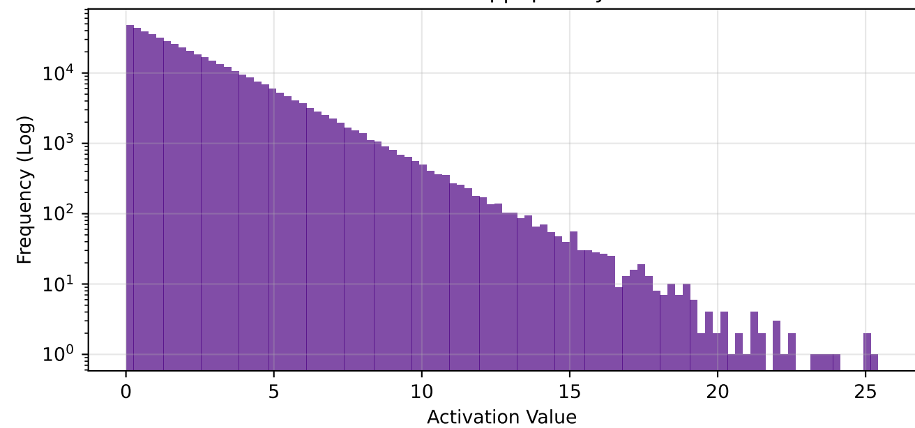
fc1 - Global Freq | Sparsity: 63.9%
