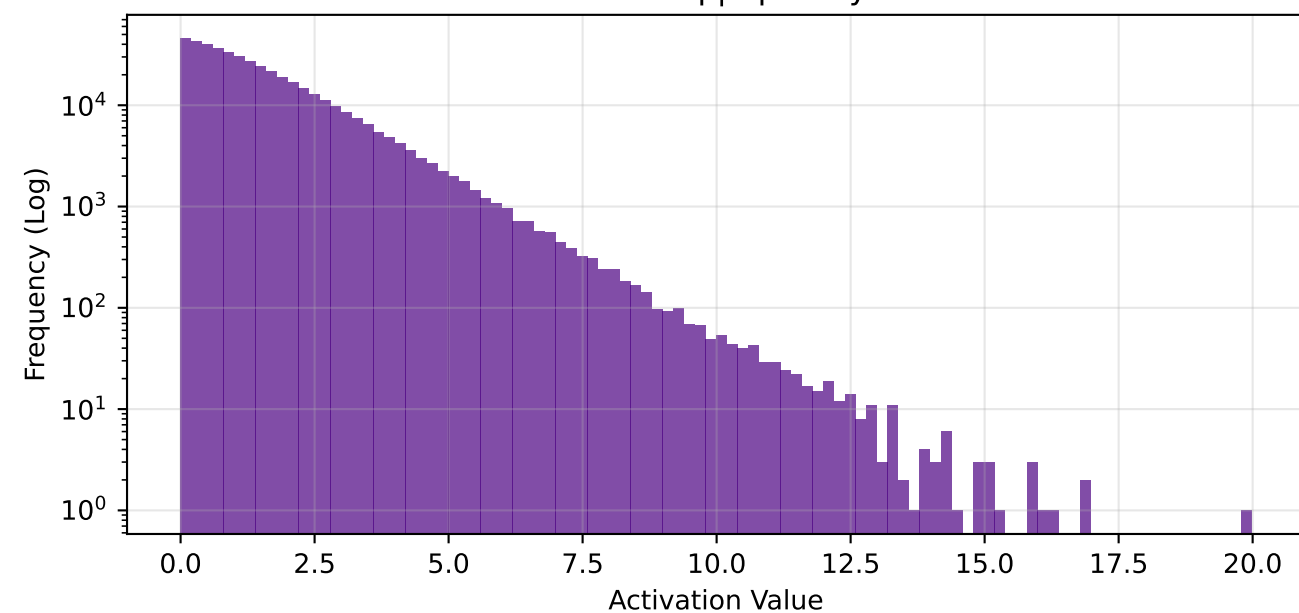
fc1 - Global Freq | Sparsity: 64.9%
