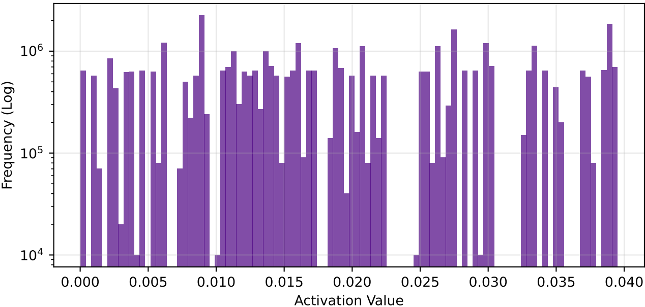
conv3 - Global Freq | Sparsity: 49.2%
