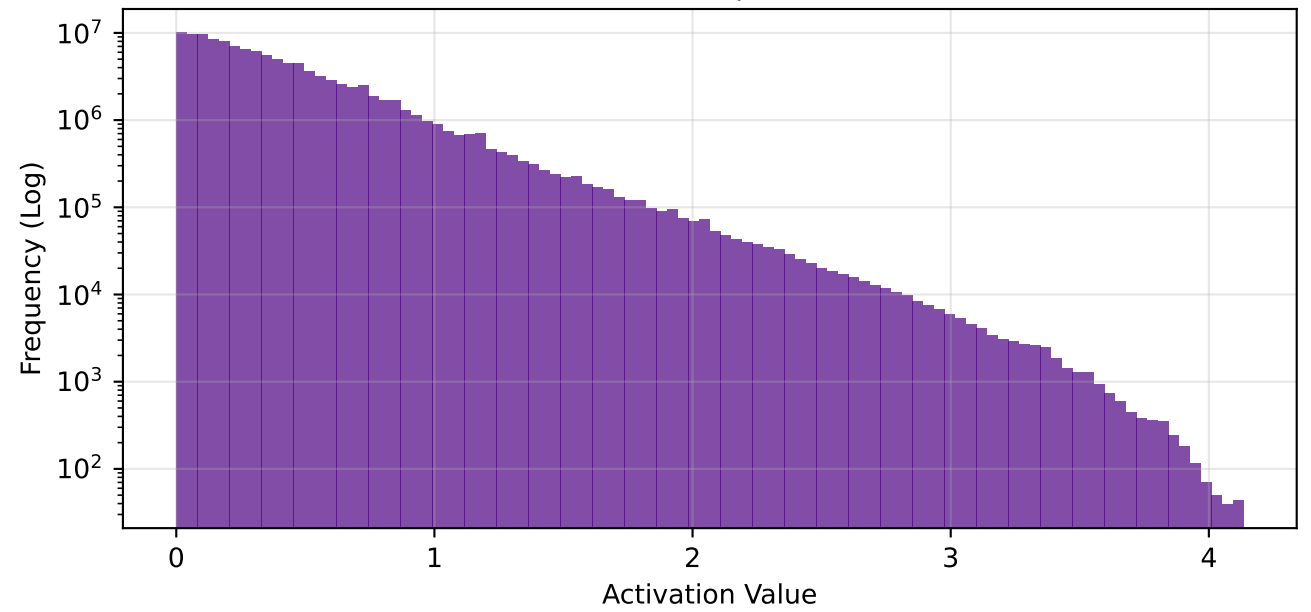
conv3 - Global Freq | Sparsity: 91.7%
