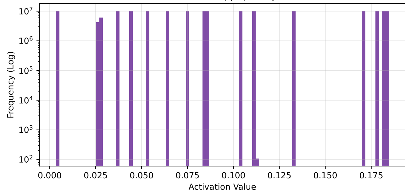
conv3 - Global Freq | Sparsity: 51.6%
