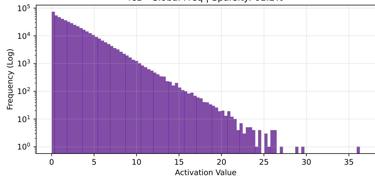
fc1 - Global Freq | Sparsity: 61.2%
