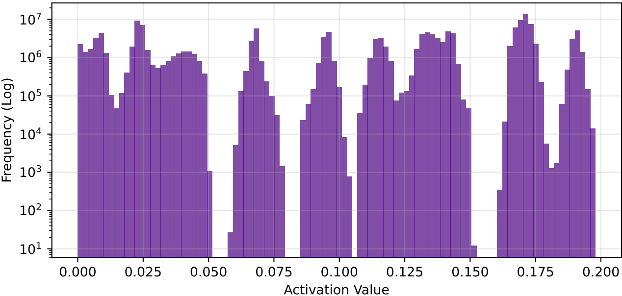
conv1 - Global Freq | Sparsity: 51.9%
