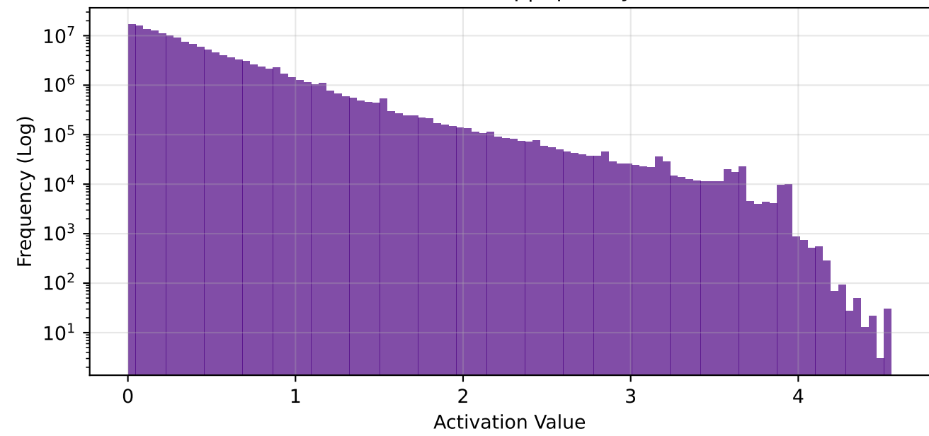
conv3 - Global Freq | Sparsity: 87.5%
