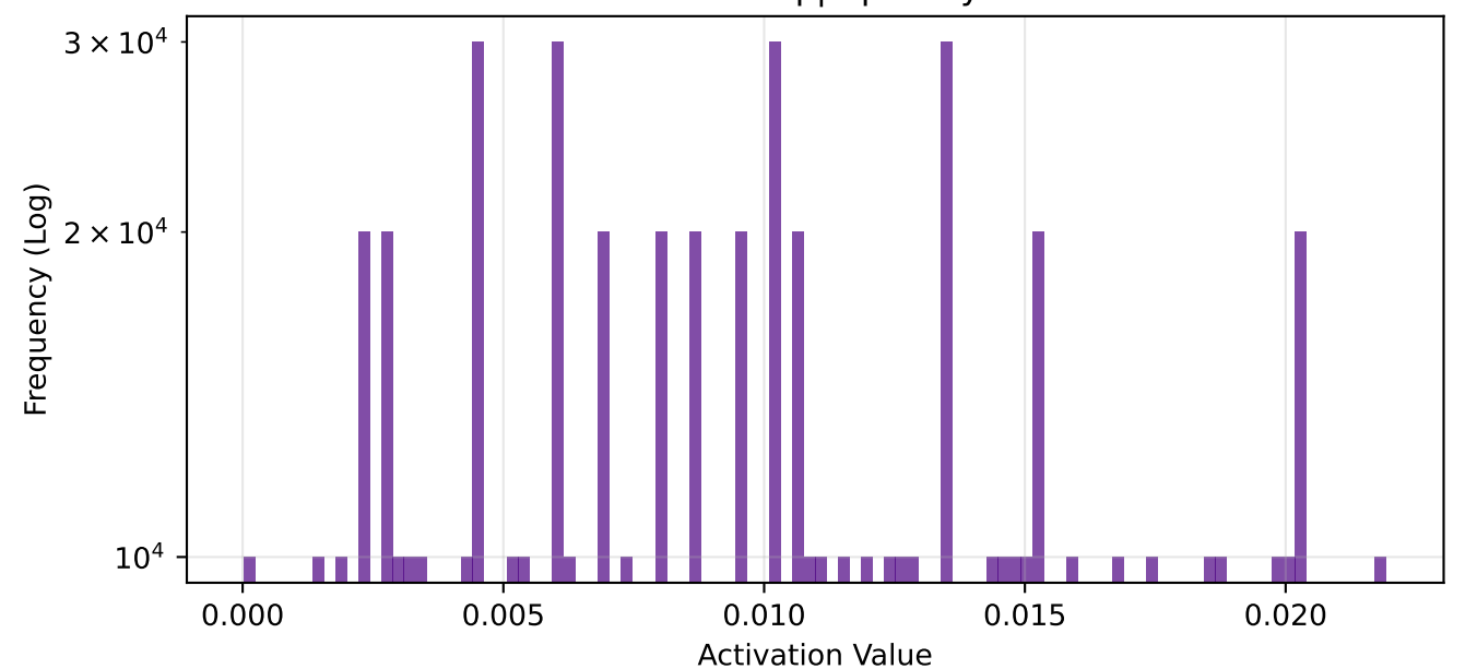
fc1 - Global Freq | Sparsity: 53.1%
