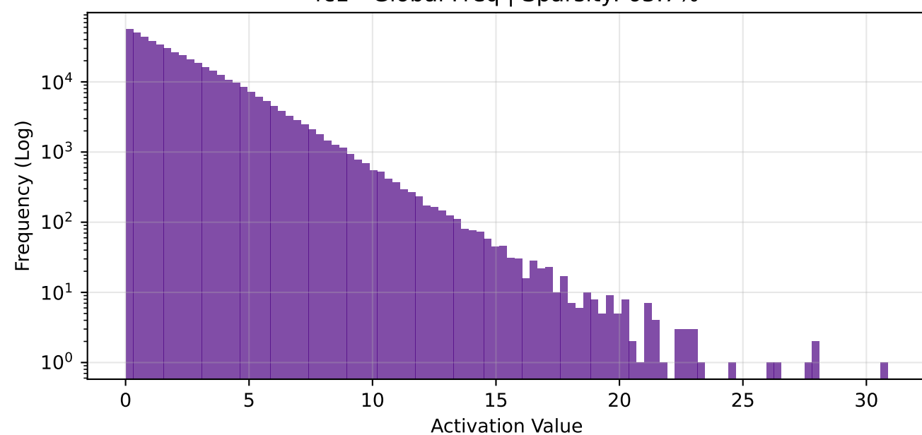
fc1 - Global Freq | Sparsity: 63.7%
