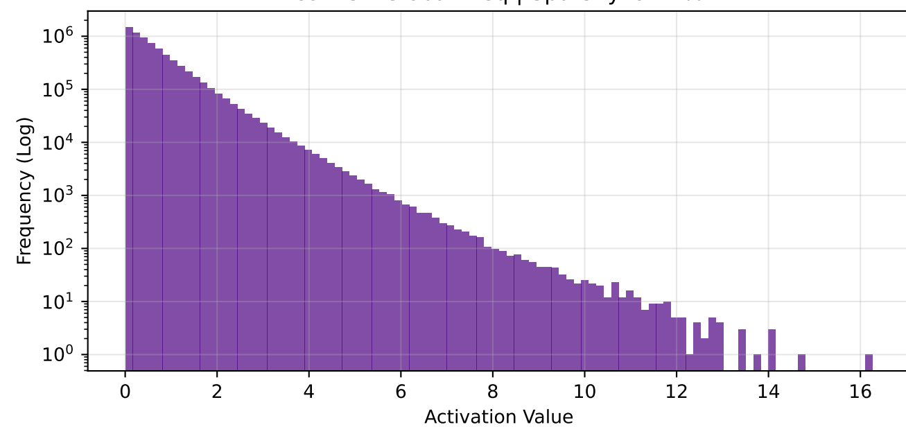
fc1 - Global Freq | Sparsity: 70.5%
