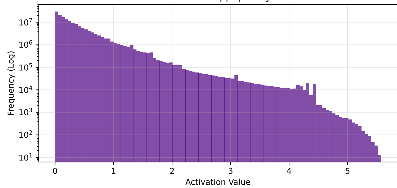
conv3 - Global Freq | Sparsity: 74.7%
