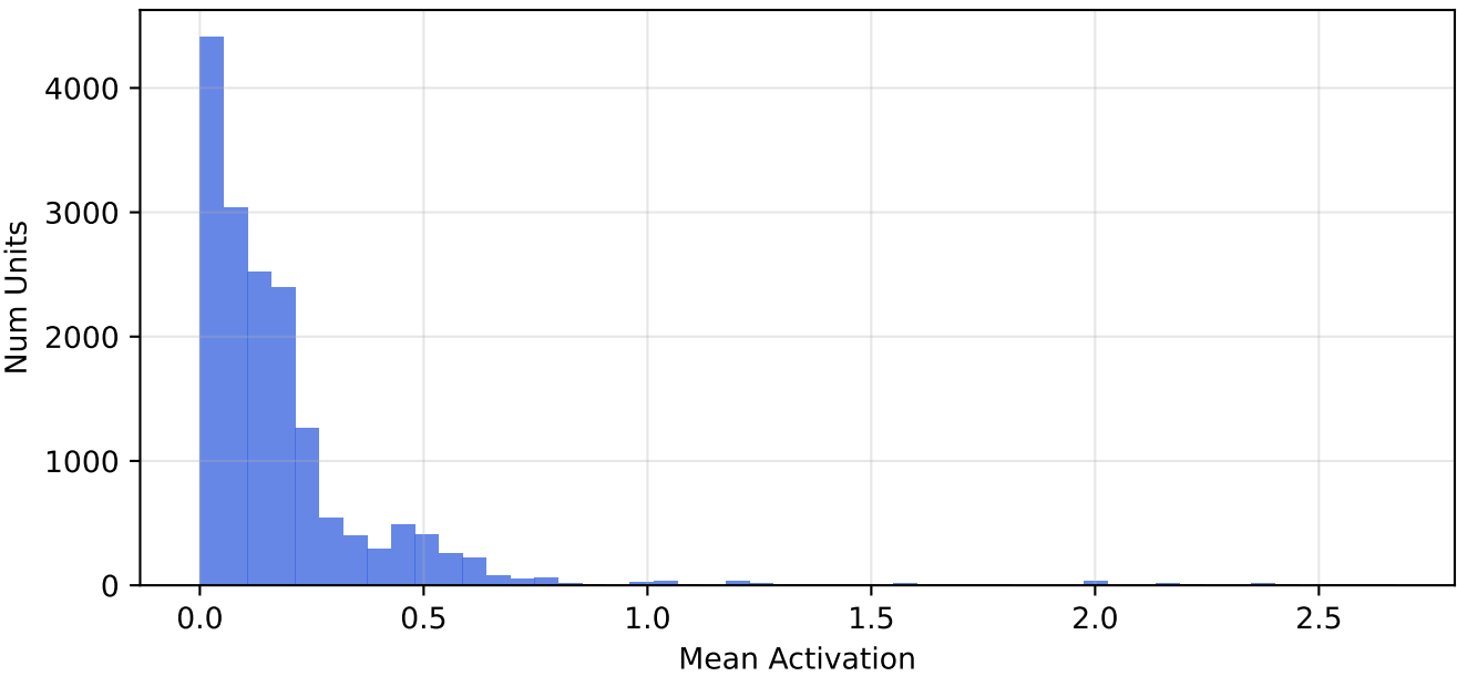
conv1 - Mean Activation/Unit
