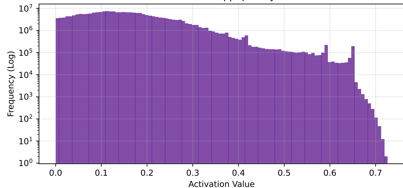
conv3 - Global Freq | Sparsity: 51.9%
