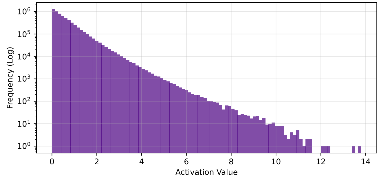
fc1 - Global Freq | Sparsity: 68.8%
