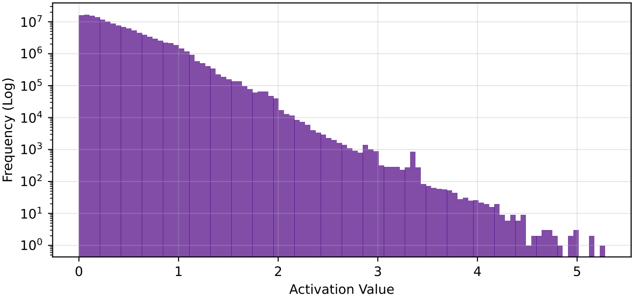
conv3 - Global Freq | Sparsity: 65.8%
