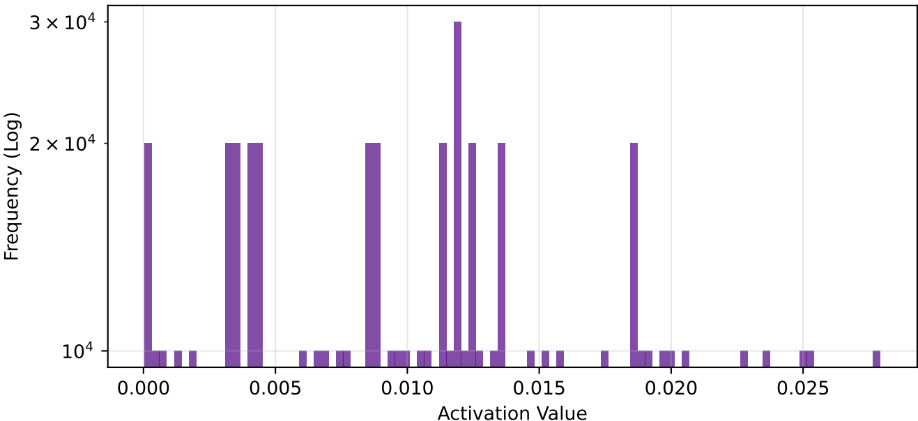
fc1 - Global Freq | Sparsity: 55.5%
