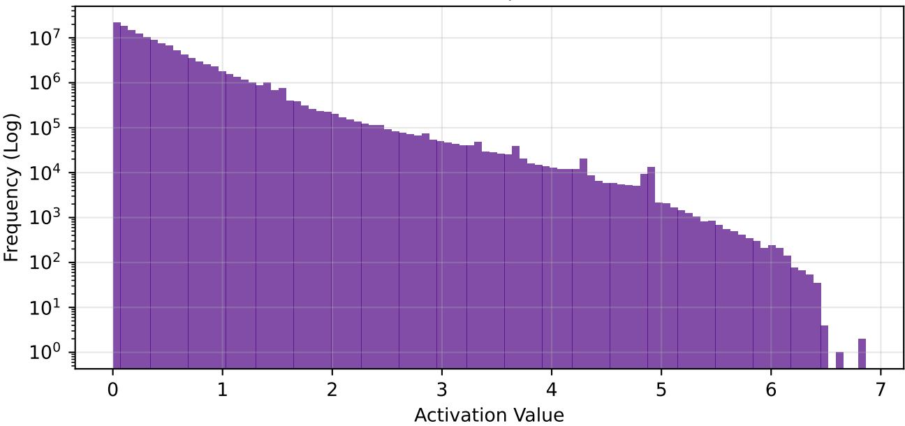
conv1 - Global Freq | Sparsity: 58.4%
