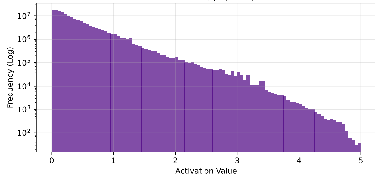
conv3 - Global Freq | Sparsity: 87.0%
