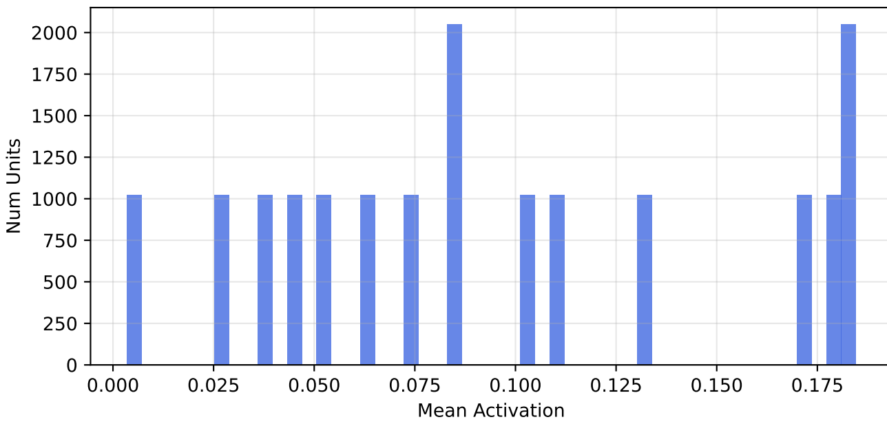
conv3 - Mean Activation/Unit
