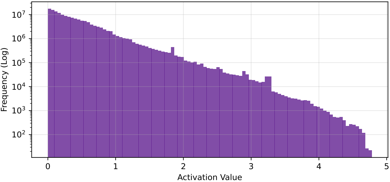
conv3 - Global Freq | Sparsity: 87.2%
