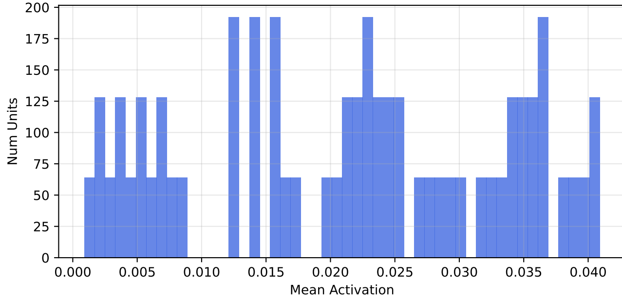
fc1 - Mean Activation/Unit
