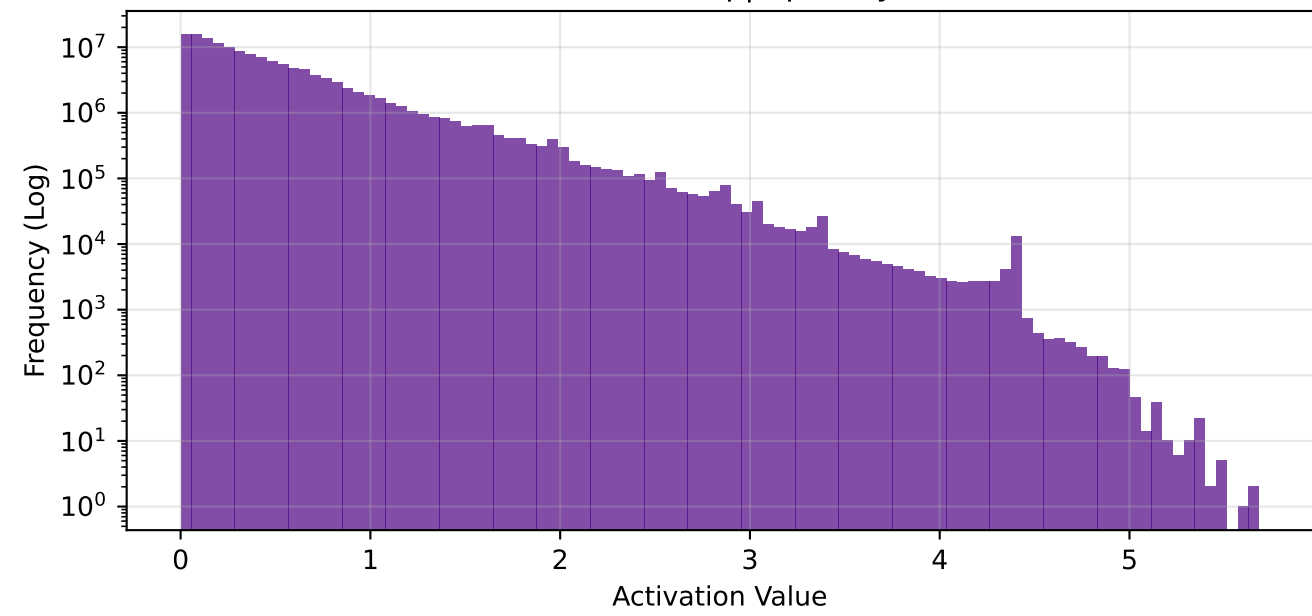
conv3 - Global Freq | Sparsity: 89.8%
