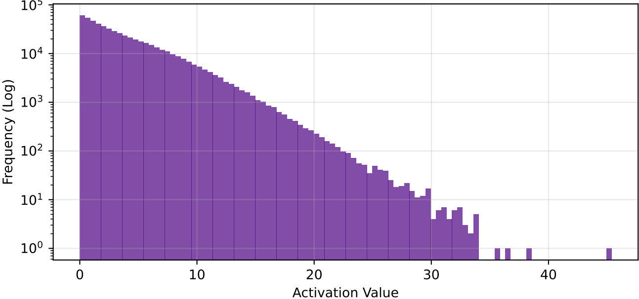
fc1 - Global Freq | Sparsity: 56.7%
