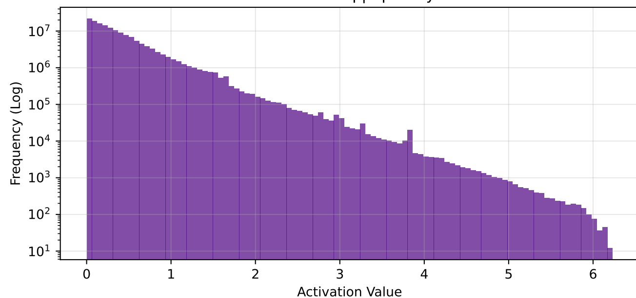
conv3 - Global Freq | Sparsity: 88.5%
