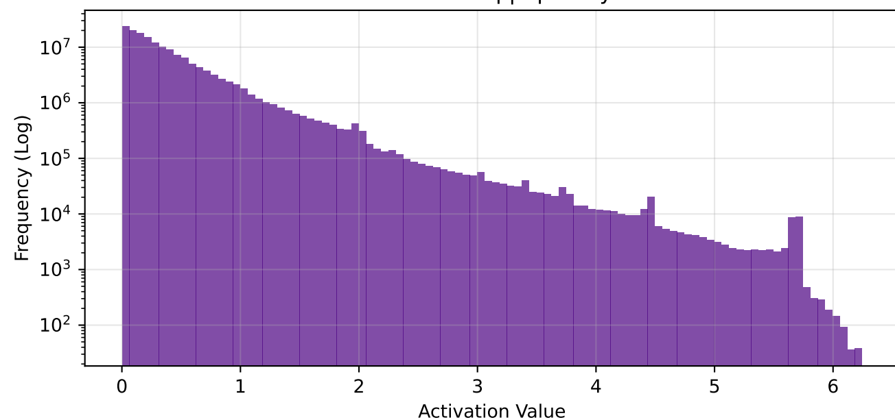
conv3 - Global Freq | Sparsity: 88.0%
