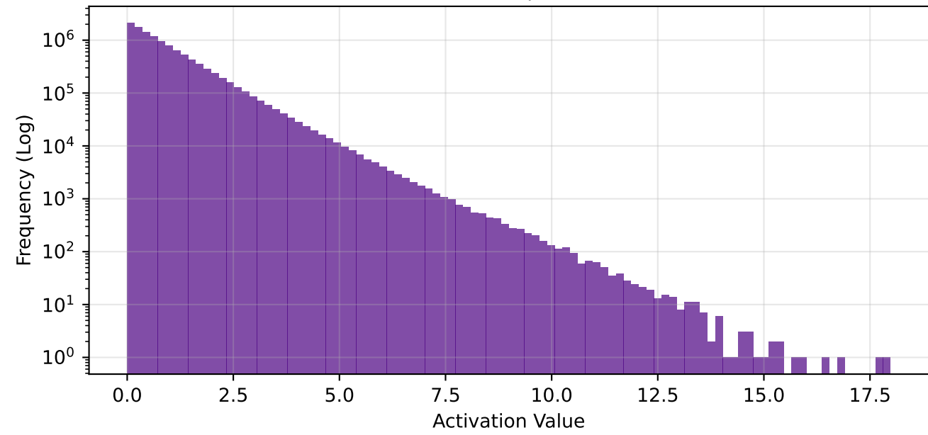
fc1 - Global Freq | Sparsity: 63.4%
