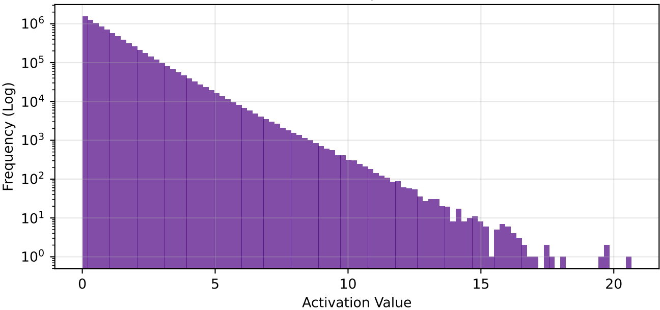
conv3 - Global Freq | Sparsity: 89.5%
