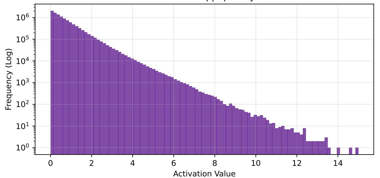
fc1 - Global Freq | Sparsity: 64.3%
