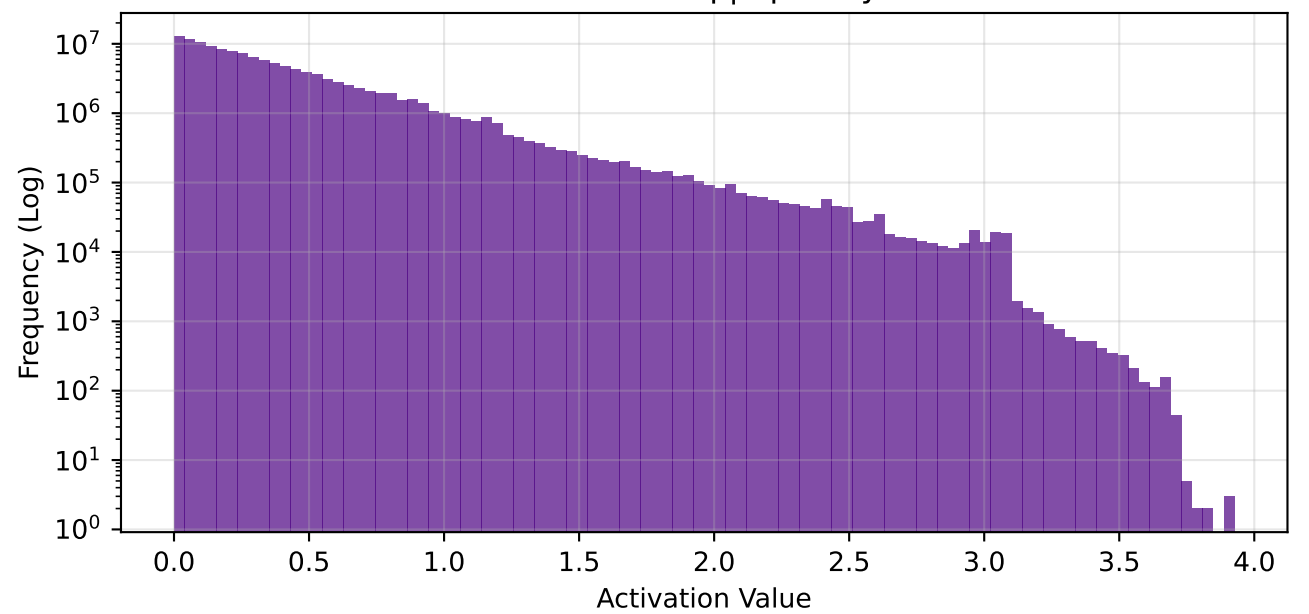
conv3 - Global Freq | Sparsity: 86.5%
