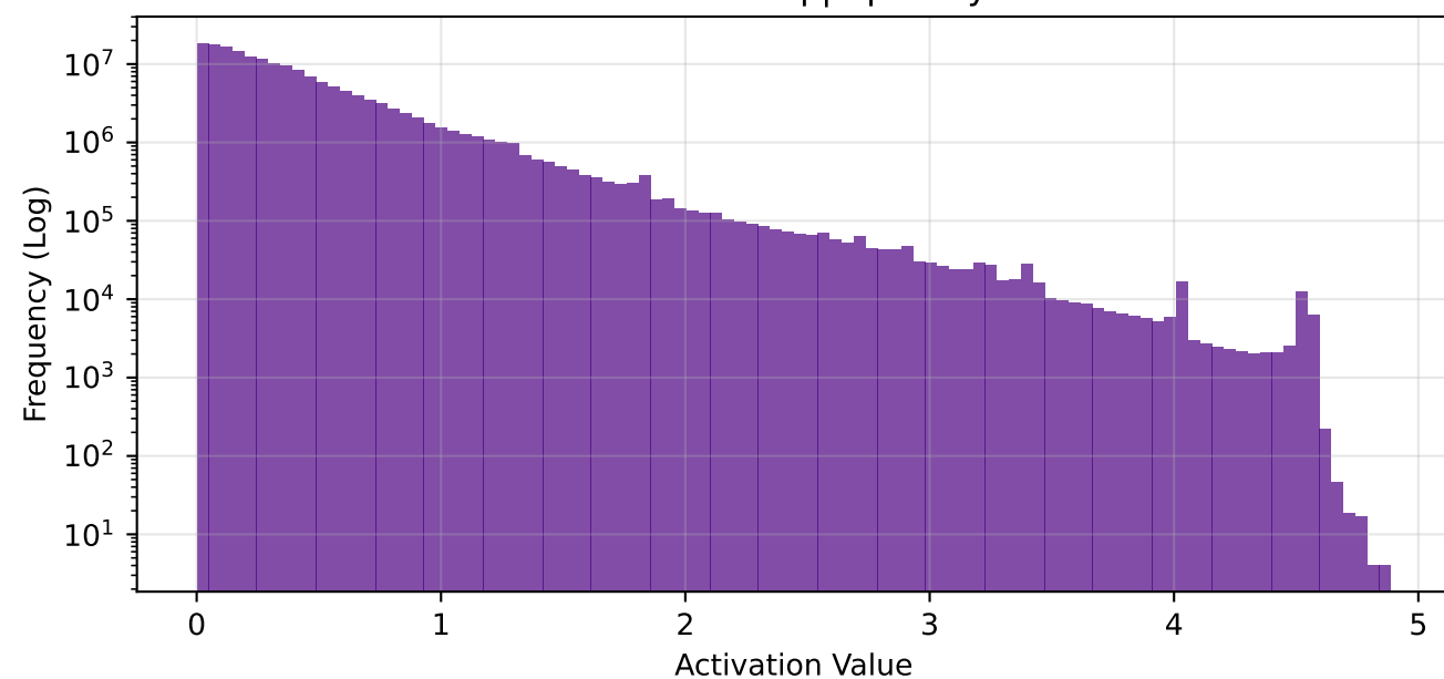
conv3 - Global Freq | Sparsity: 88.1%
