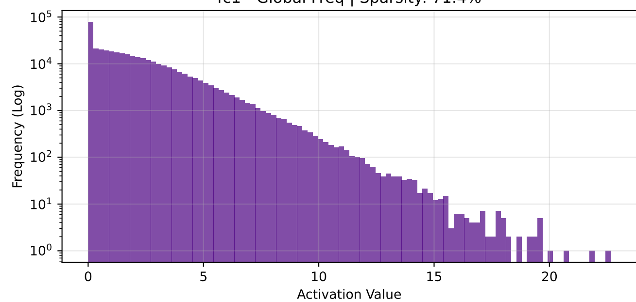
fc1 - Global Freq | Sparsity: 71.4%
