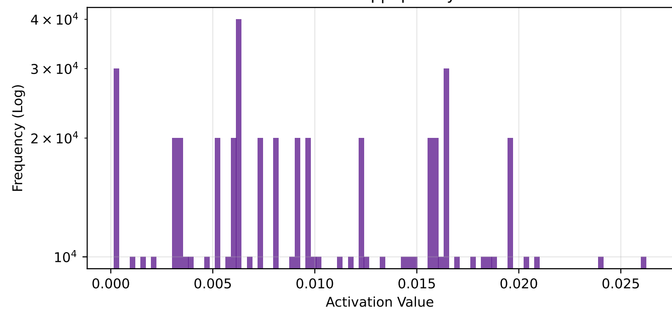
fc1 - Global Freq | Sparsity: 51.6%
