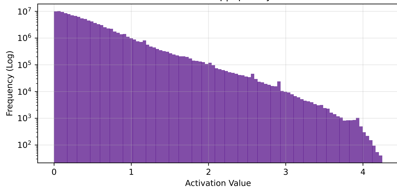
conv3 - Global Freq | Sparsity: 91.3%
