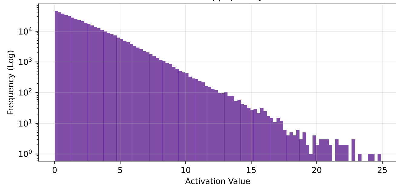
fc1 - Global Freq | Sparsity: 63.8%
