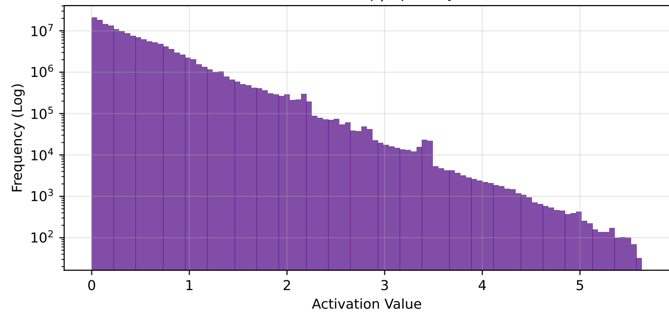
conv3 - Global Freq | Sparsity: 85.6%
