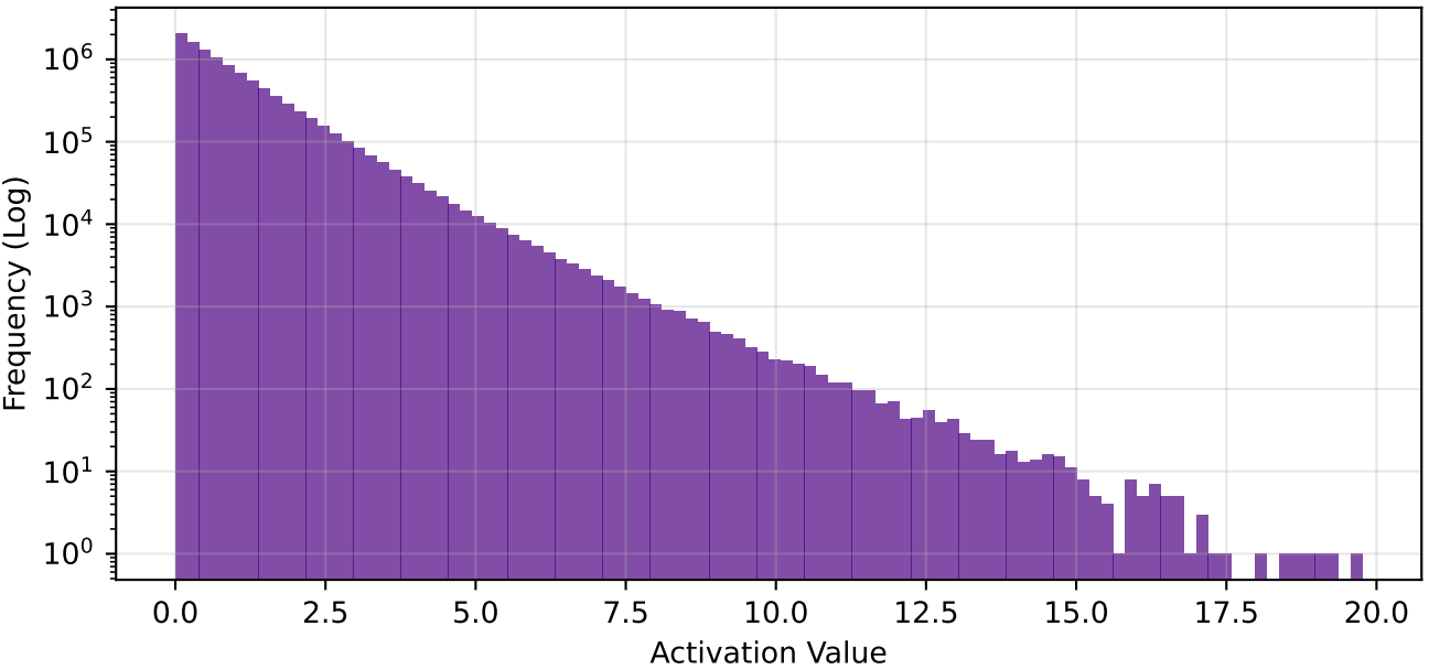
fc1 - Global Freq | Sparsity: 61.4%
