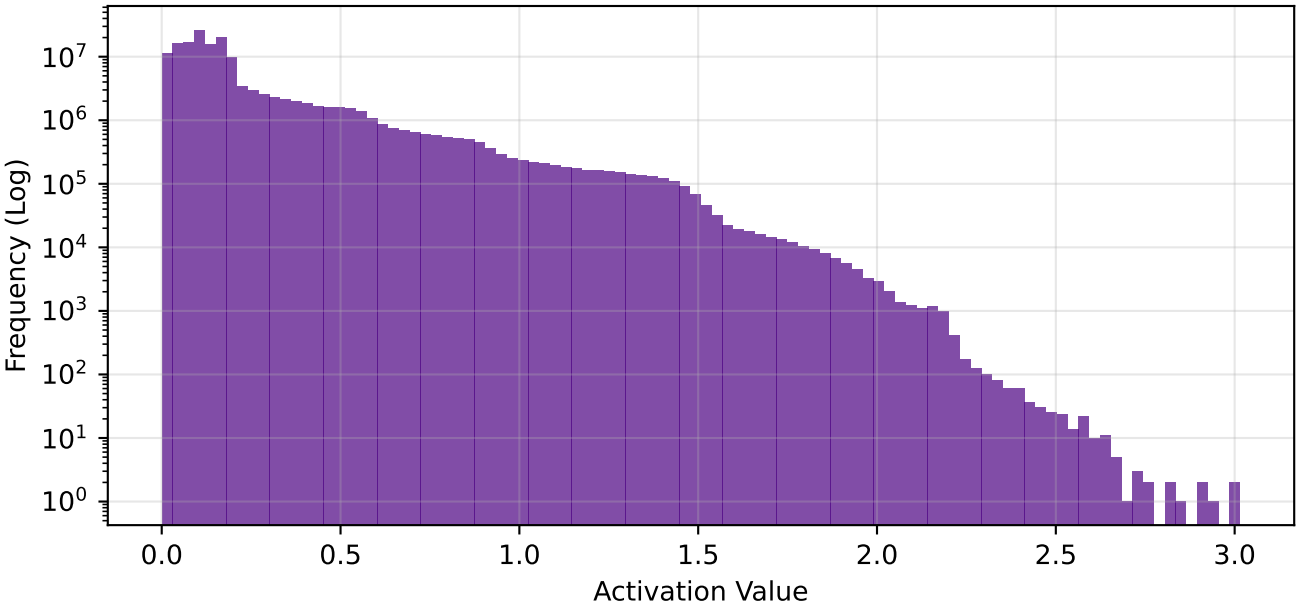
conv3 - Global Freq | Sparsity: 51.3%
