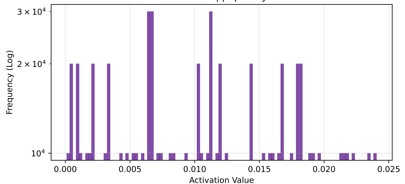
fc1 - Global Freq | Sparsity: 51.6%
