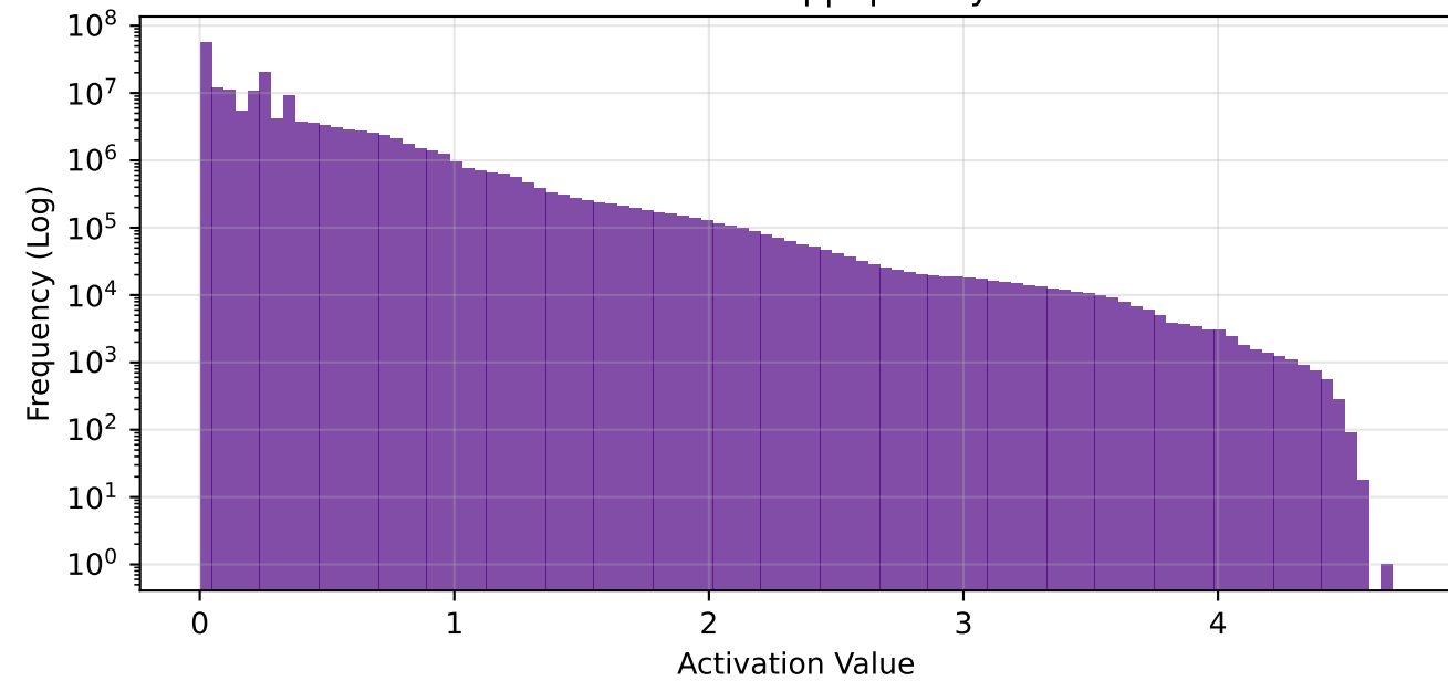
conv3 - Global Freq | Sparsity: 86.1%
