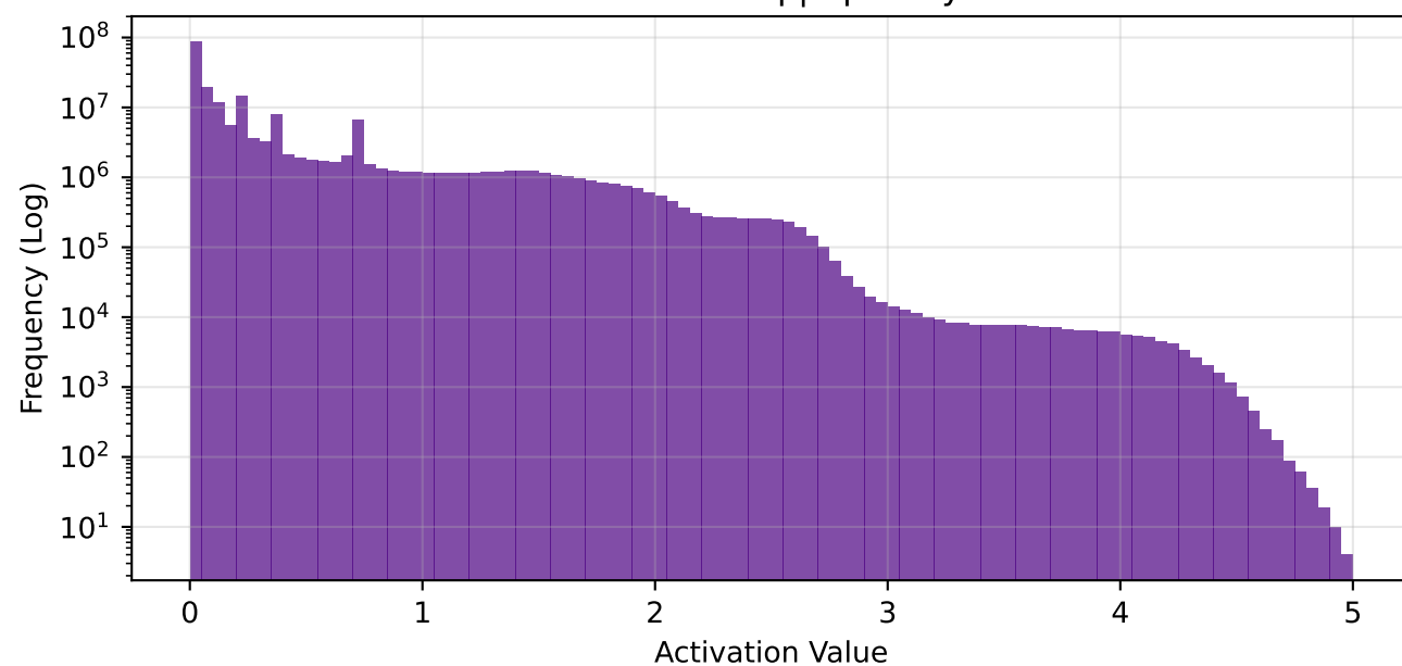
conv3 - Global Freq | Sparsity: 65.6%
