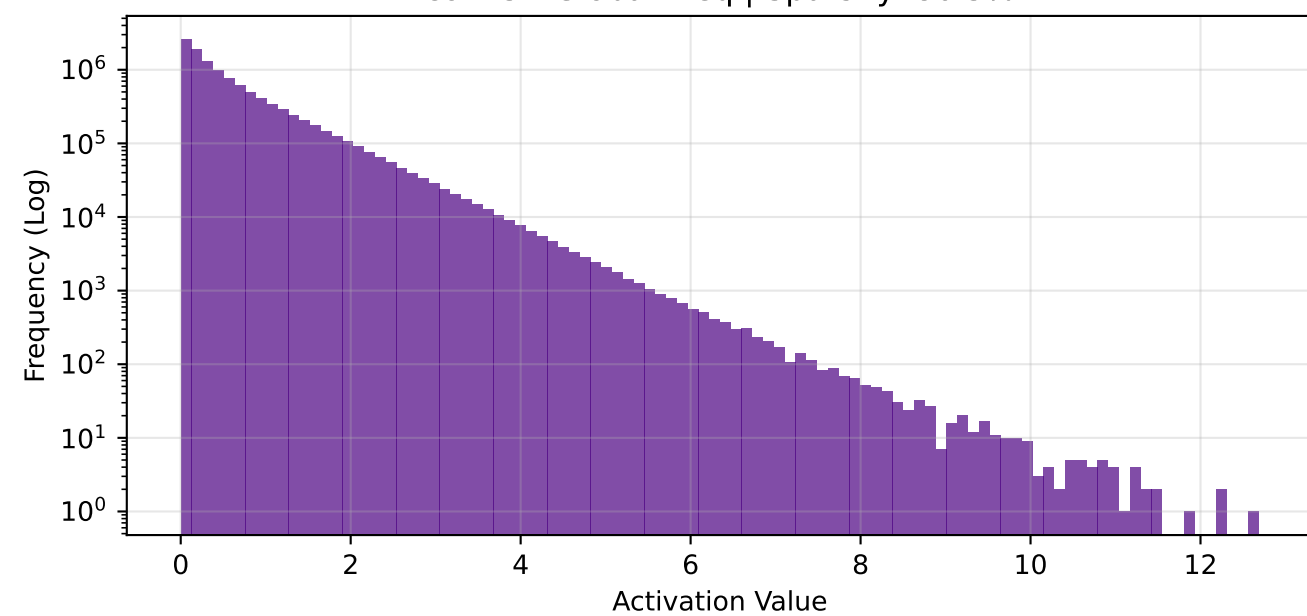
fc1 - Global Freq | Sparsity: 77.0%
