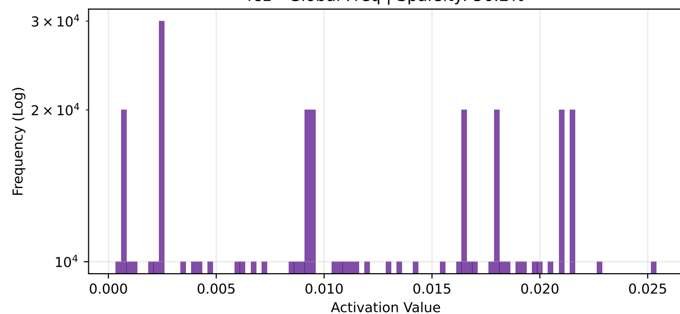
fc1 - Global Freq | Sparsity: 56.2%
