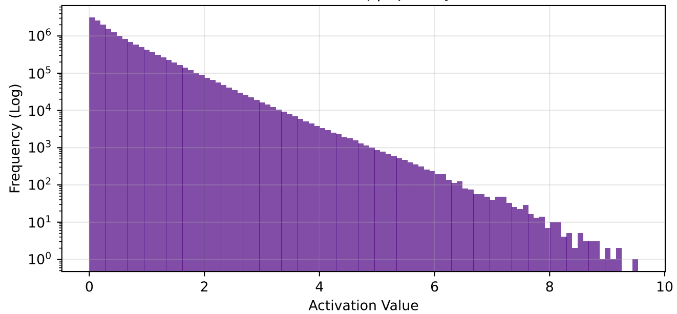
fc1 - Global Freq | Sparsity: 68.6%
