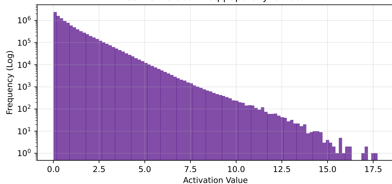
fc1 - Global Freq | Sparsity: 74.6%
