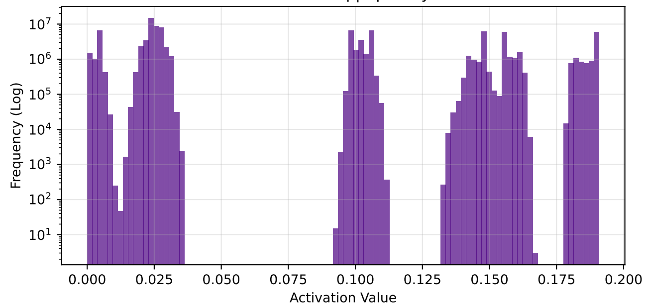
conv3 - Global Freq | Sparsity: 51.6%
