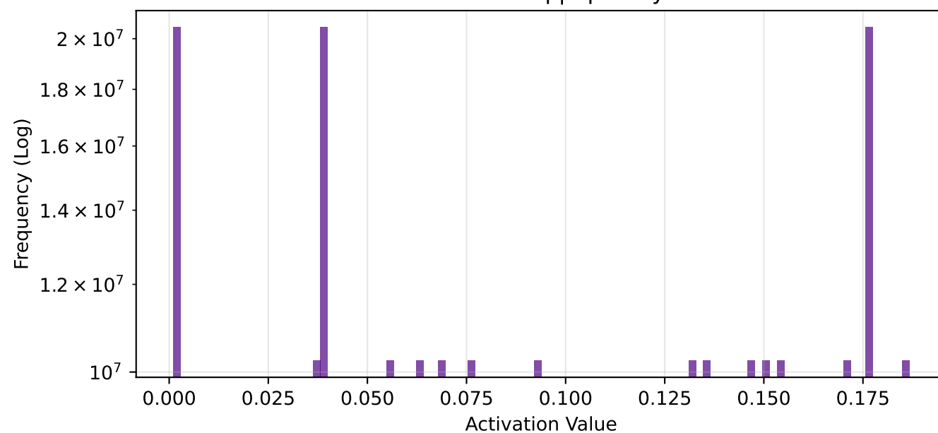
conv3 - Global Freq | Sparsity: 50.0%
