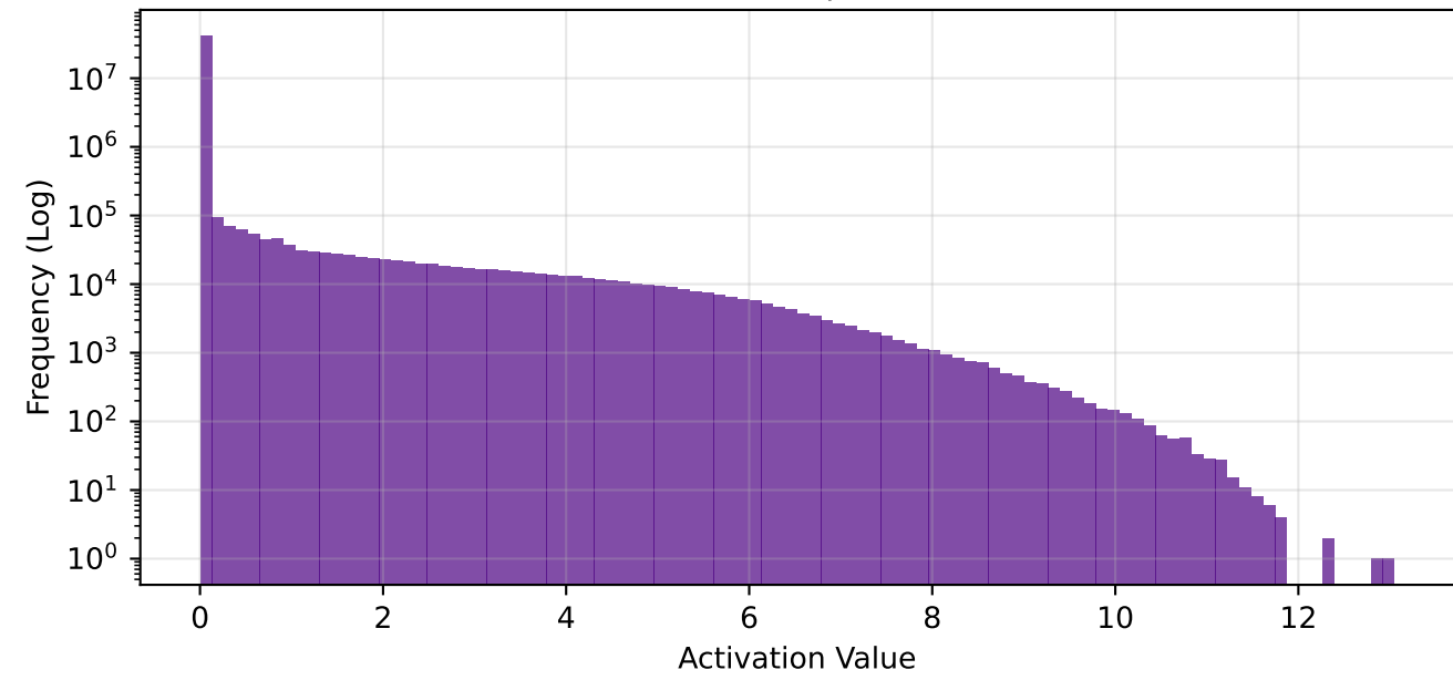
fc1 - Global Freq | Sparsity: 50.8%
