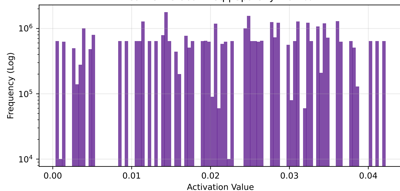
fc1 - Global Freq | Sparsity: 51.6%
