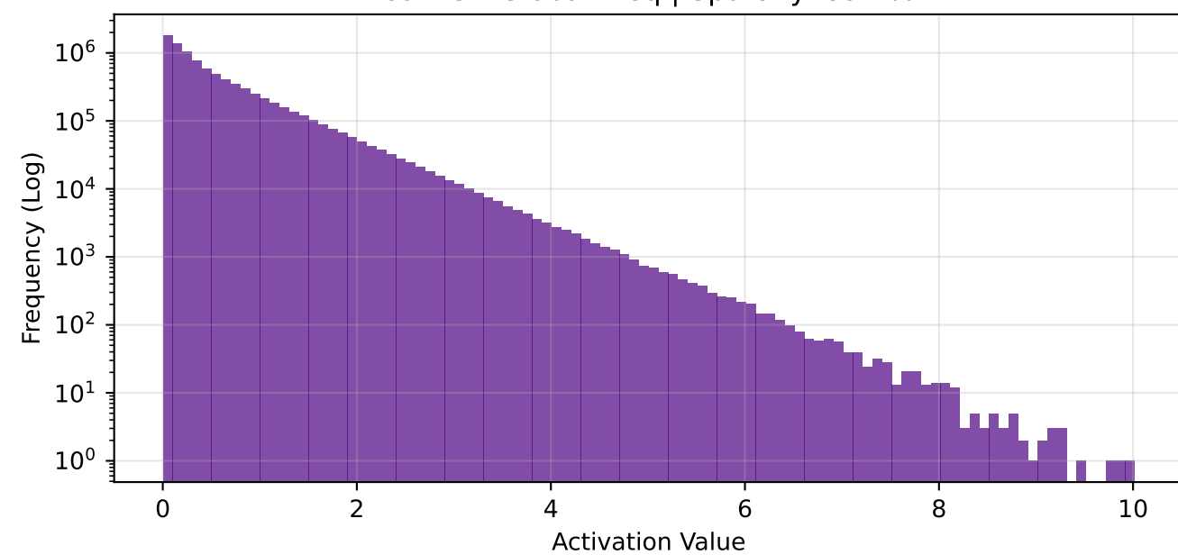
fc1 - Global Freq | Sparsity: 75.4%
