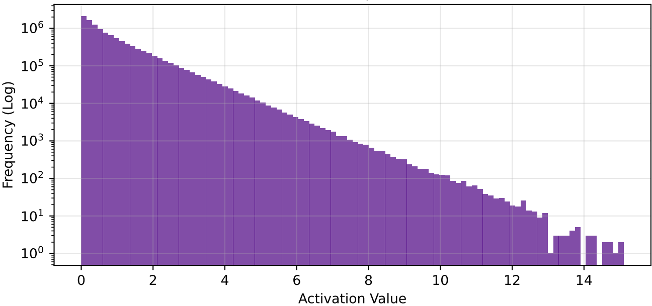
fc1 - Global Freq | Sparsity: 75.0%
