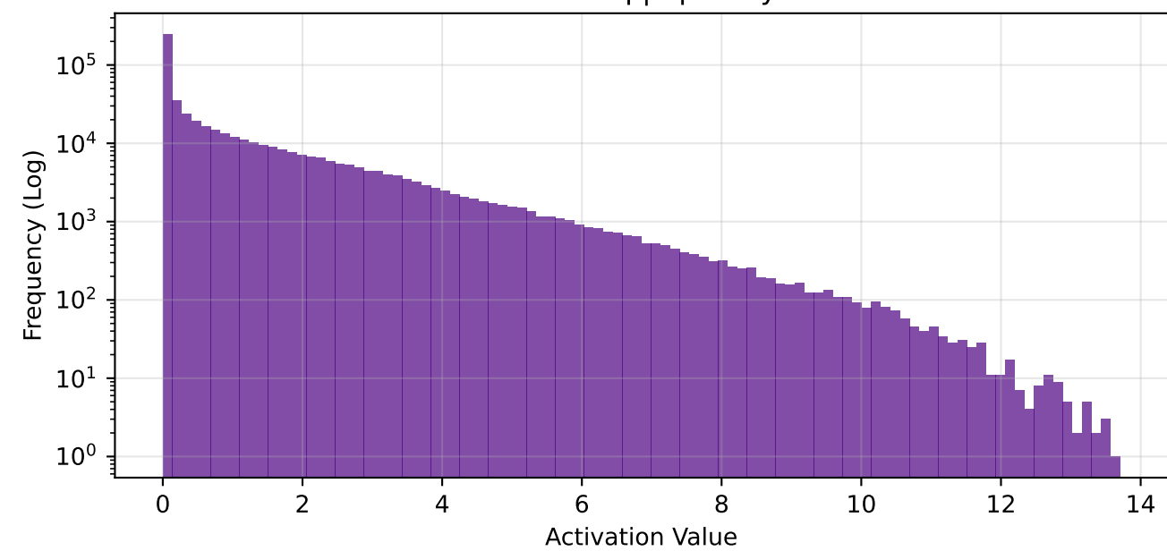
fc1 - Global Freq | Sparsity: 57.6%
