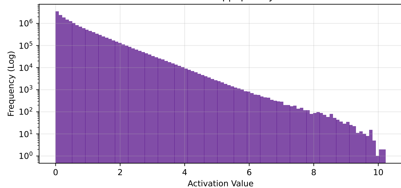
fc1 - Global Freq | Sparsity: 60.2%
