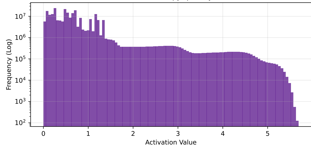
conv3 - Global Freq | Sparsity: 61.6%
