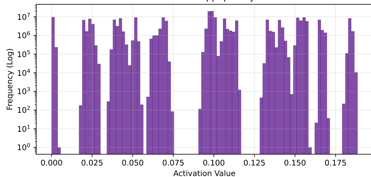
conv3 - Global Freq | Sparsity: 54.4%
