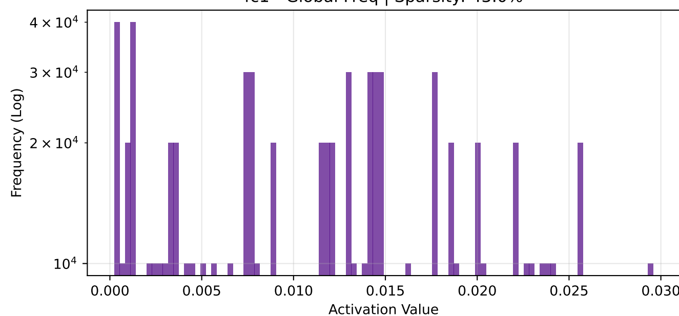
fc1 - Global Freq | Sparsity: 43.0%
