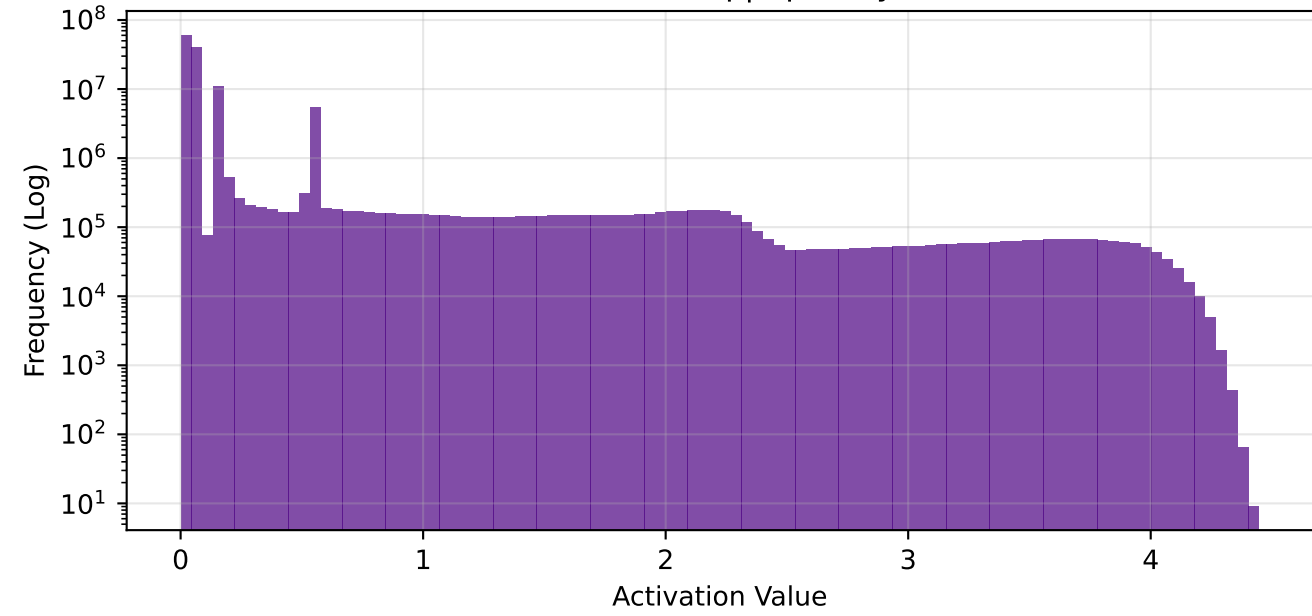
conv3 - Global Freq | Sparsity: 48.4%
