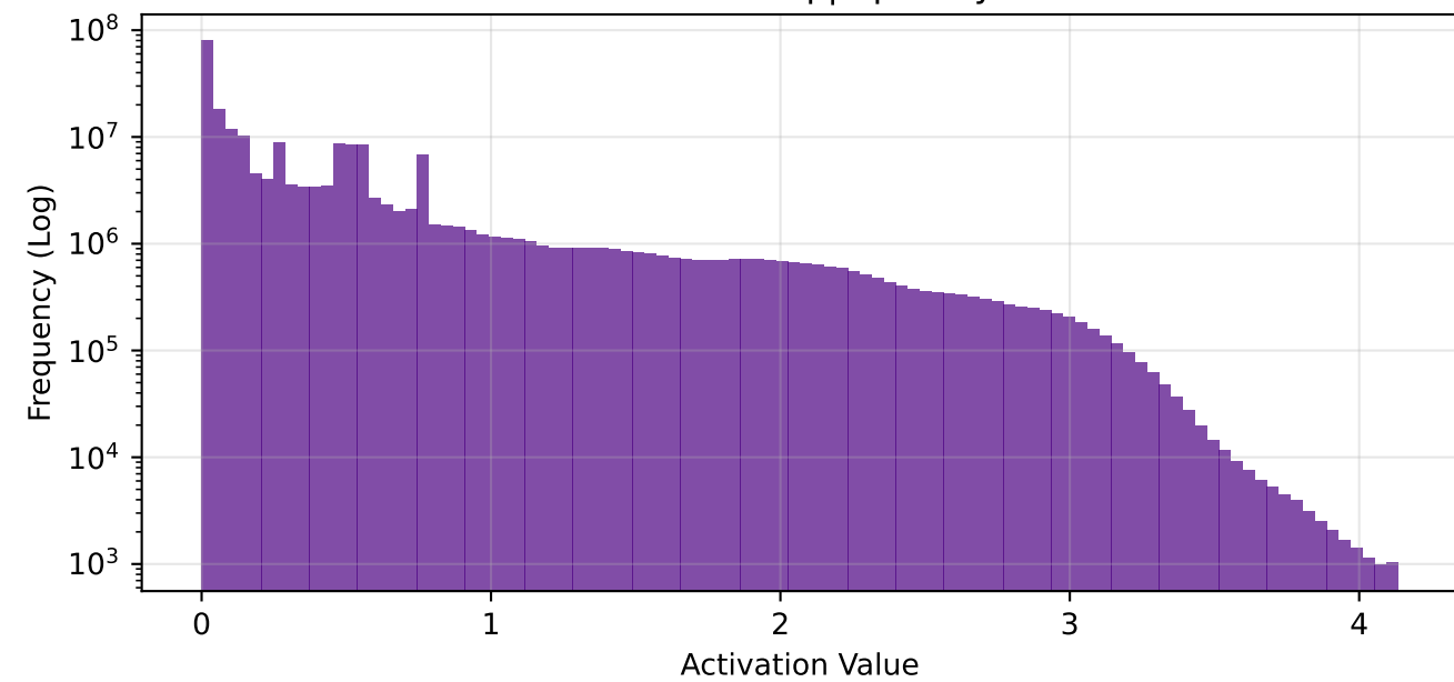
conv3 - Global Freq | Sparsity: 78.3%
