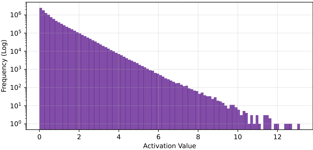
fc1 - Global Freq | Sparsity: 75.0%
