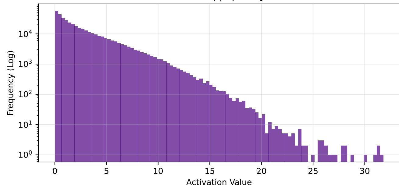
fc1 - Global Freq | Sparsity: 69.6%
