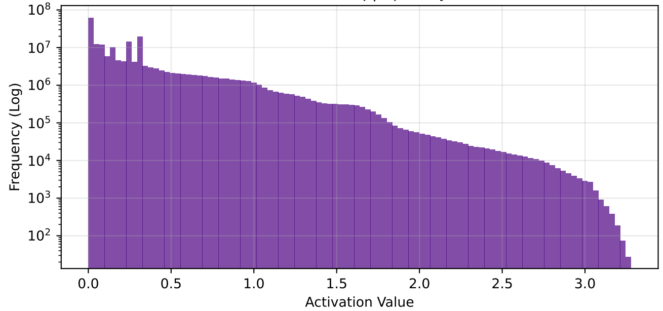
conv3 - Global Freq | Sparsity: 79.4%
