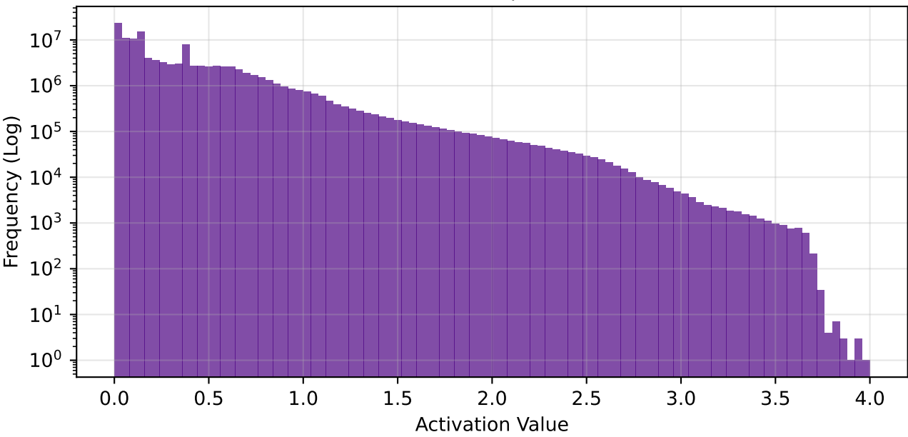
conv3 - Global Freq | Sparsity: 87.0%
