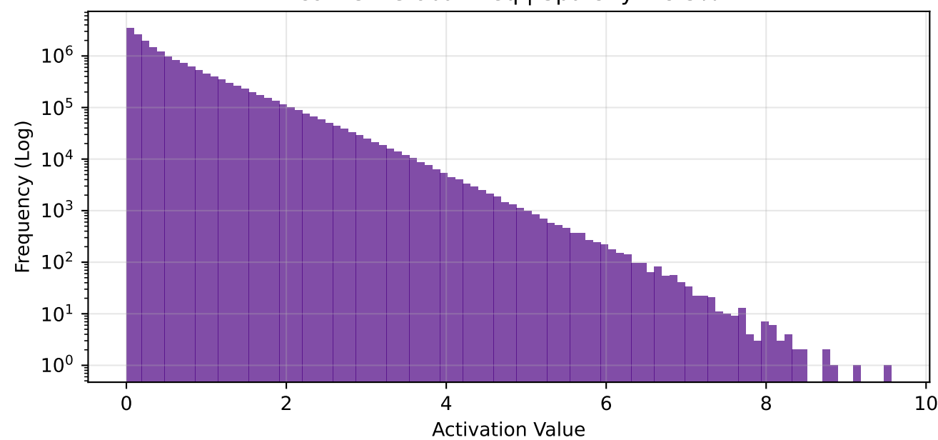
fc1 - Global Freq | Sparsity: 70.6%
