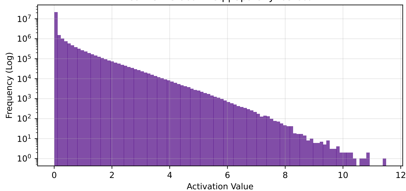
fc1 - Global Freq | Sparsity: 62.4%
