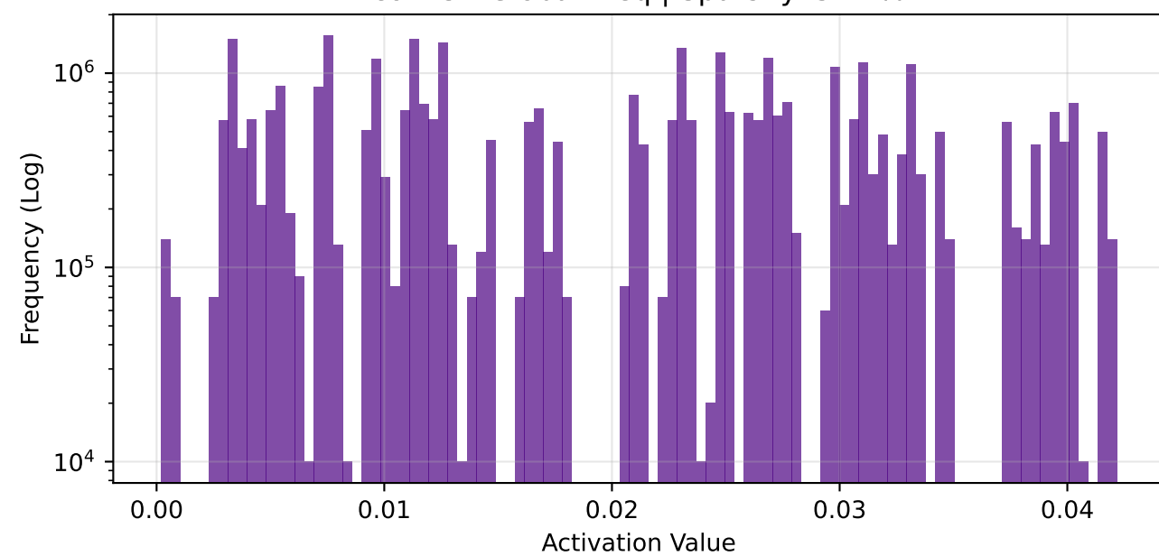
fc1 - Global Freq | Sparsity: 56.2%
