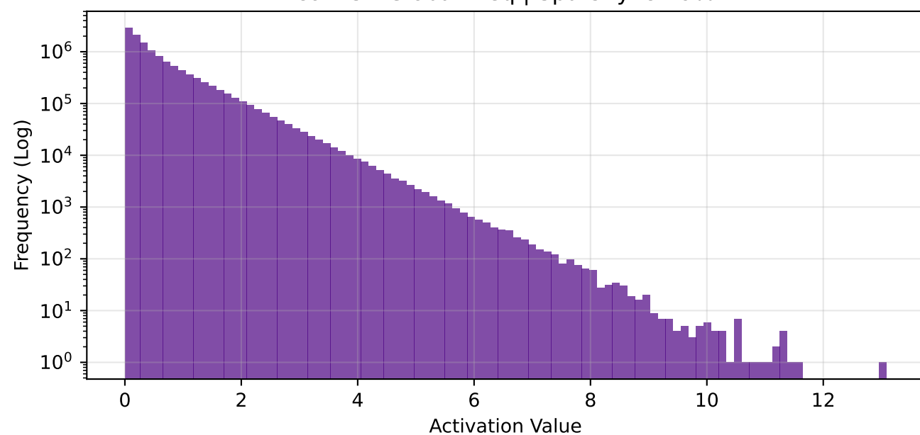
fc1 - Global Freq | Sparsity: 74.9%
