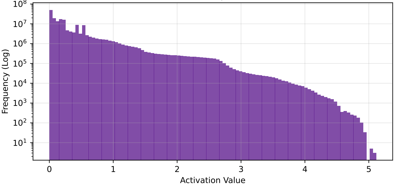
conv3 - Global Freq | Sparsity: 83.7%
