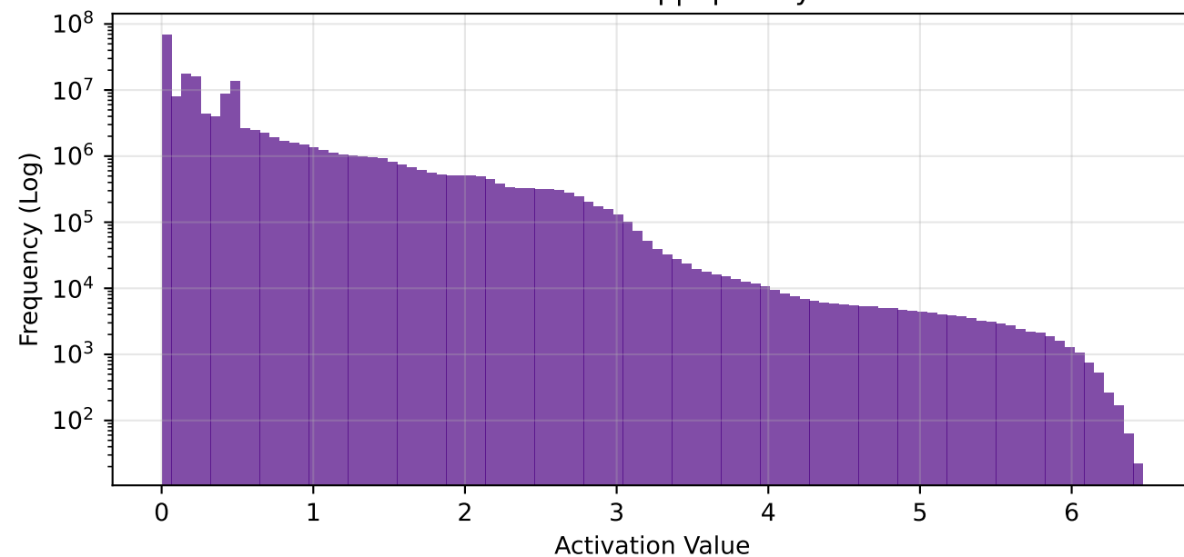
conv3 - Global Freq | Sparsity: 80.0%
