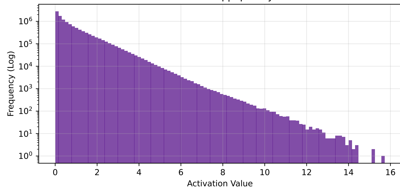
fc1 - Global Freq | Sparsity: 73.4%
