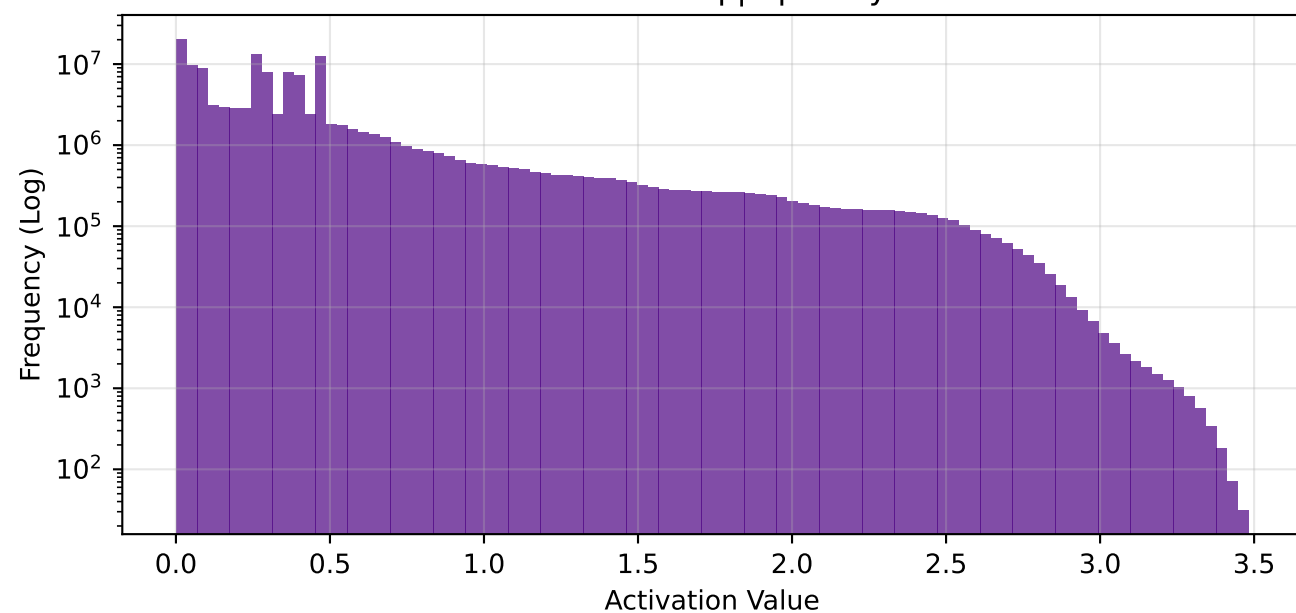
conv3 - Global Freq | Sparsity: 84.9%
