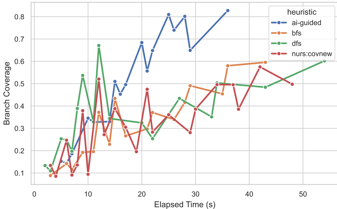
Average Branch Coverage Over Time
