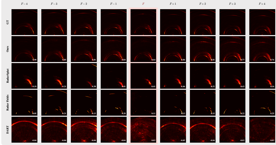
Figure 3: Per-frame |RA| comparison, scene S0 F135. Columns: 8 training frames ( F \pm 1 \dots \pm 4 , black headers) and 1 held-out test frame ( F , red header). Rows: GT, mm3DGS (Ours), RadarSplat, Radar Fields, DART. Per-cell CC overlaid.
