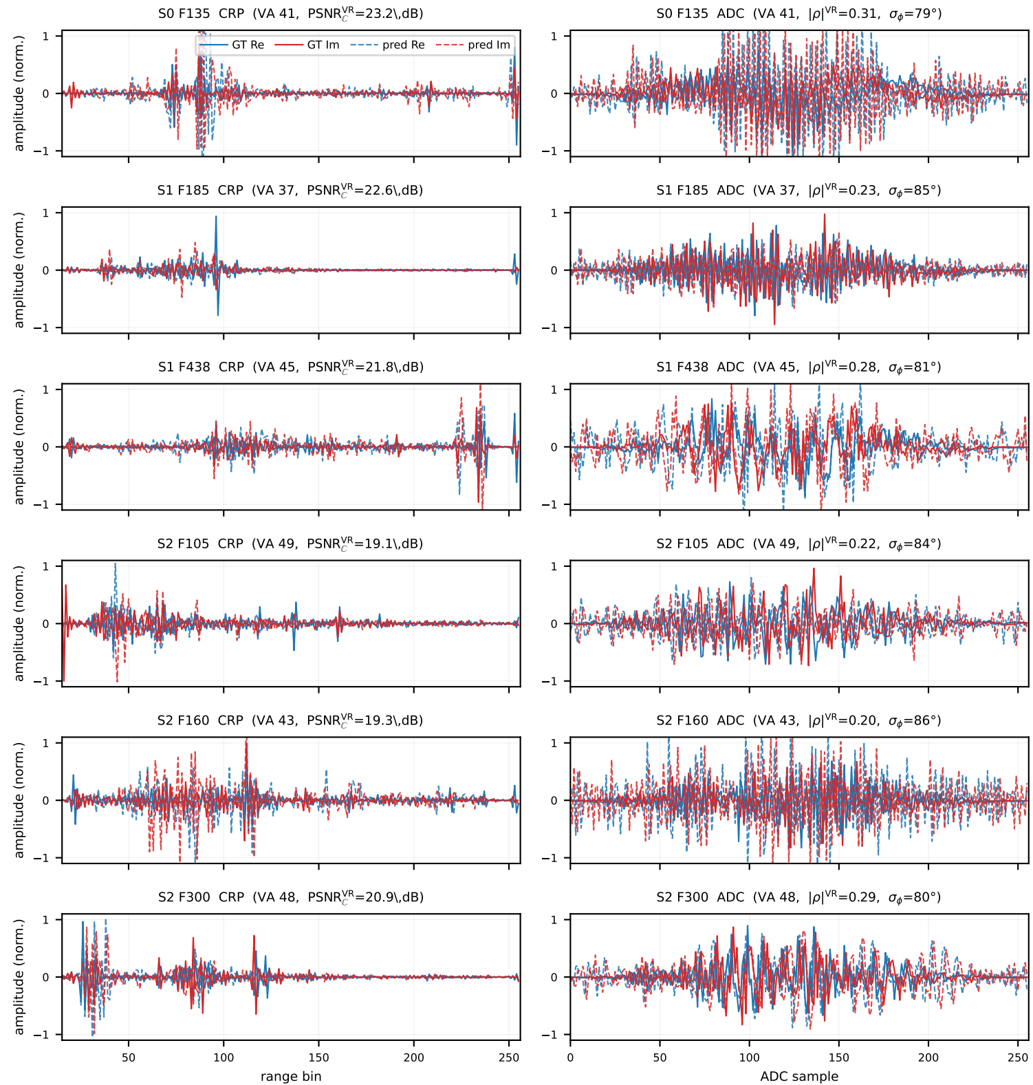
Phase-corrected I/Q traces: GT (solid) vs prediction (dashed) at the highest-energy virtual antenna per scene.
