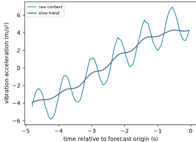
Raw context mixes drift and vibration
