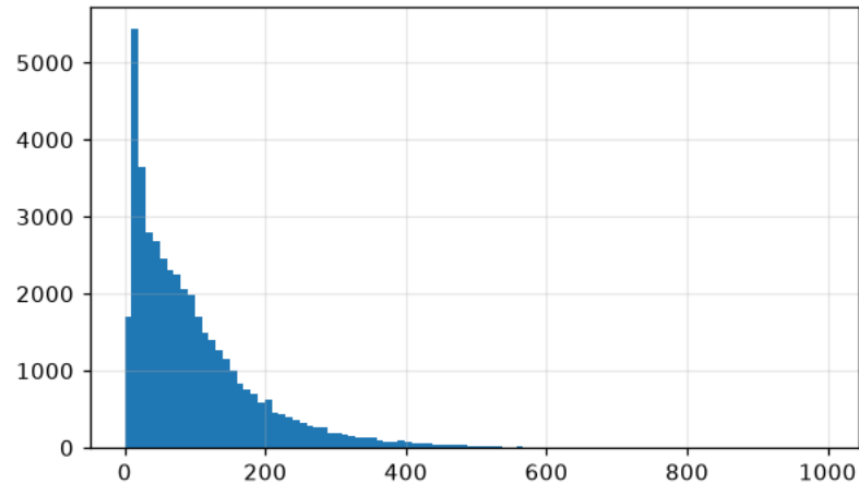
raw values: heavy right tail
