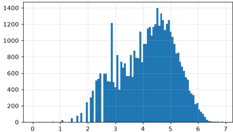
\log_{10}(\text{values}) : close to symmetric
