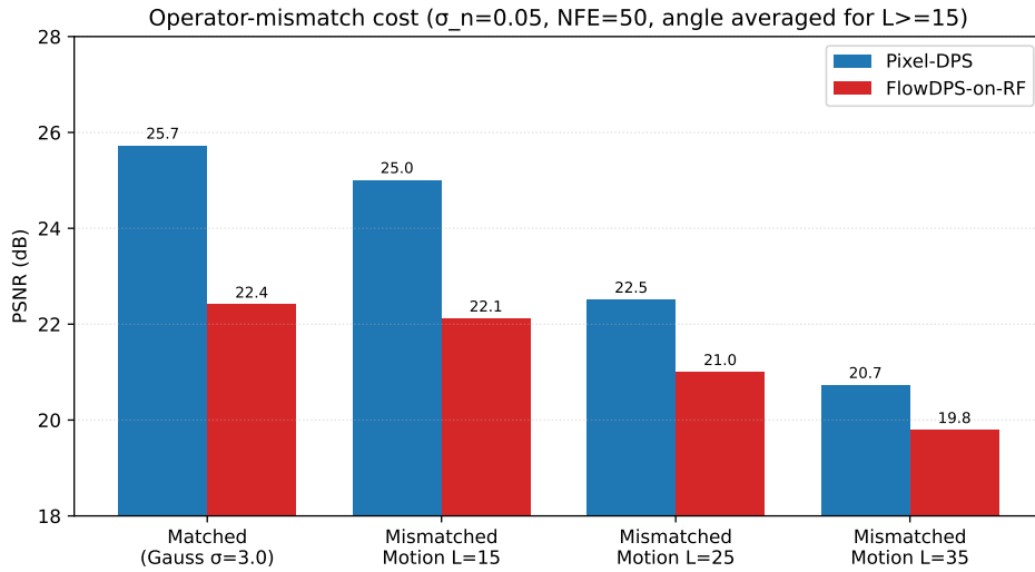
Figure 3: Operator-mismatch cost ( \sigma_n=0.05 , \text{NFE}=50 ). Pixel-DPS drops \sim 5 dB from matched Gaussian to severe motion ( L=35 ); FlowDPS-on-RF drops only \sim 2.5 dB.
