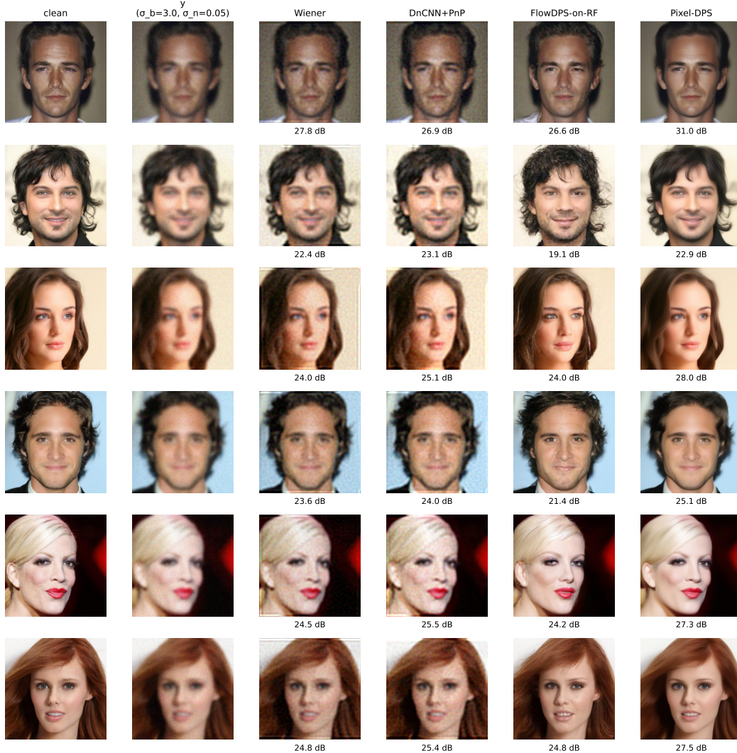
Figure 4: Qualitative comparison on six representative CelebA-HQ-256 test images at \sigma_b=3.0 , \sigma_n=0.05 , NFE=50. Columns: clean ground truth, degraded measurement, Wiener filter, DnCNN+PnP-ADMM, FlowDPS-on-RF, and Pixel-DPS. Numbers below each reconstruction are per-image PSNR (dB). Wiener and DnCNN+PnP are smooth but oversmooth identity-relevant detail; FlowDPS-on-RF sometimes drifts to a plausible-but-wrong face; Pixel-DPS most consistently recovers identity-preserving facial structure.
