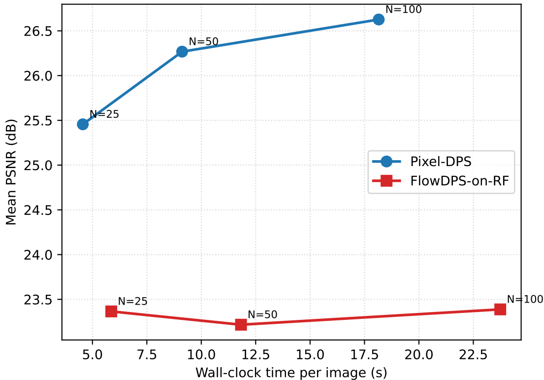
Quality-efficiency frontier (avg across all degradation conditions)
