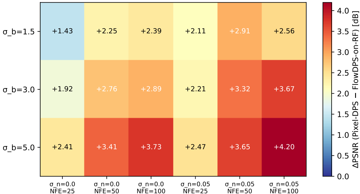
Pixel-DPS advantage over FlowDPS-on-RF in PSNR
