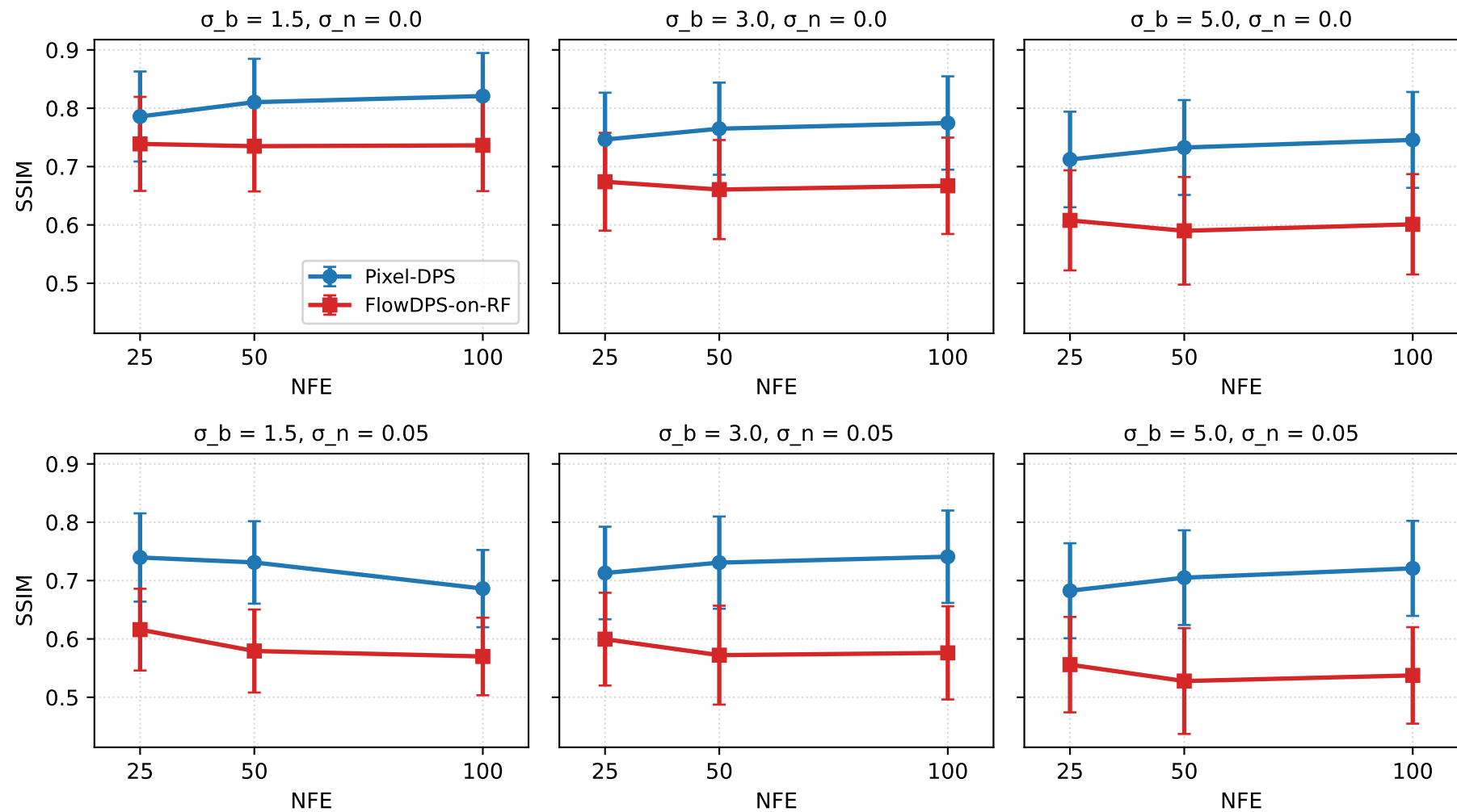
SSIM vs NFE across degradation conditions
