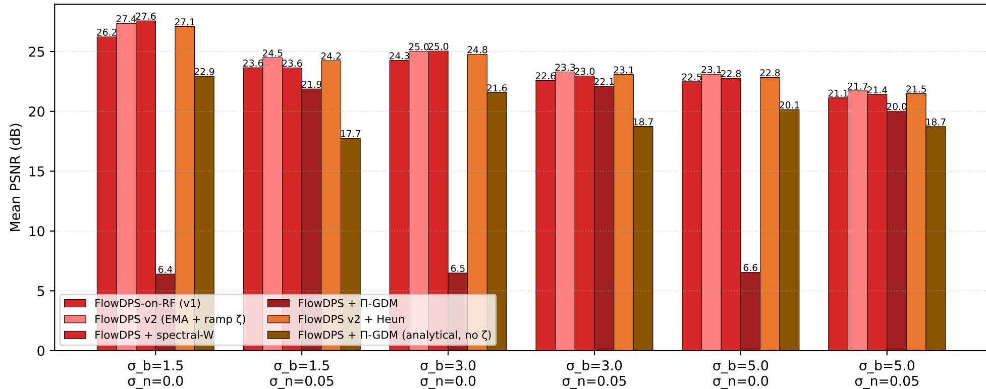
FlowDPS-on-RF family — tier ablation at NFE=100
