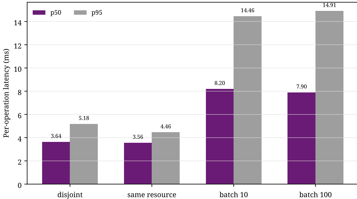
ECTC workload and batching measurements
