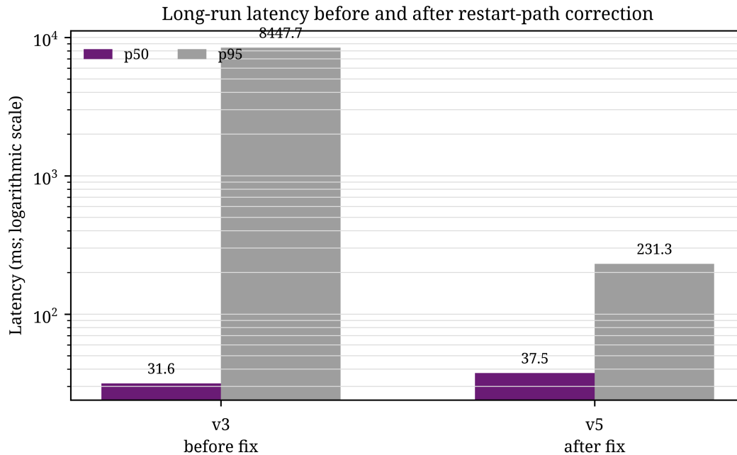
Fig. 8. p50 and p95 latency before and after the restart-path correction in the local long-run artifacts. The logarithmic scale exposes the former recovery tail. with a closure proof and successor seal, while Conflict and Abandoned remain independently inspectable artifacts.
