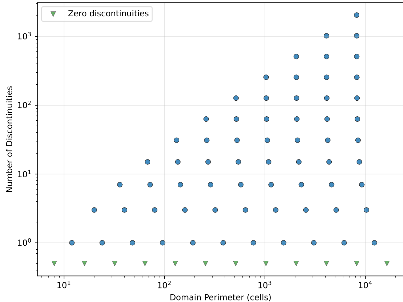
Hamilton CHI Discontinuities vs Domain Perimeter (2D)
