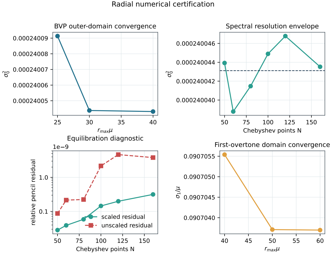
Figure 5. Numerical certification of the low radial modes. The panels show ground-mode BVP outer-domain convergence, the broad N = 50 –160 spectral envelope, scaled and unscaled pencil residuals, and first-overtone domain convergence. Spectral drift is oscillatory rather than monotonic, motivating an envelope instead of a formal extrapolation.
