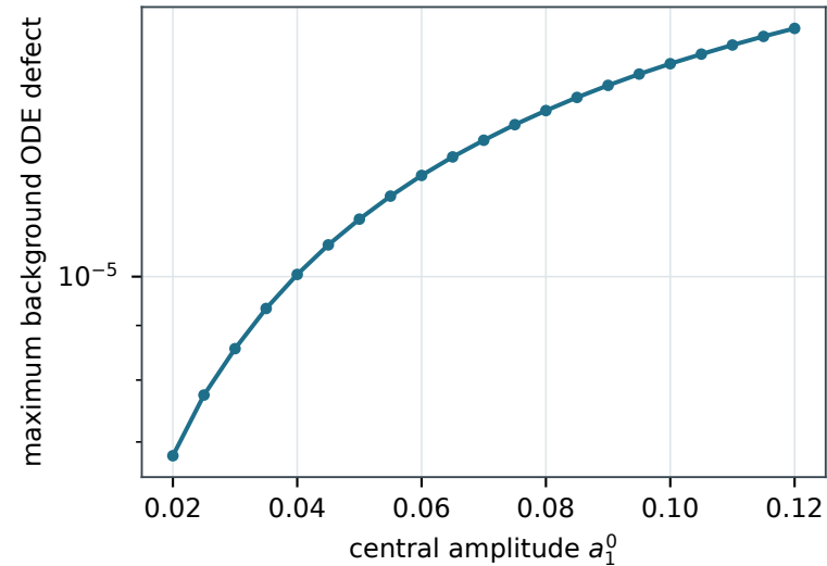
Dense first-order residual
