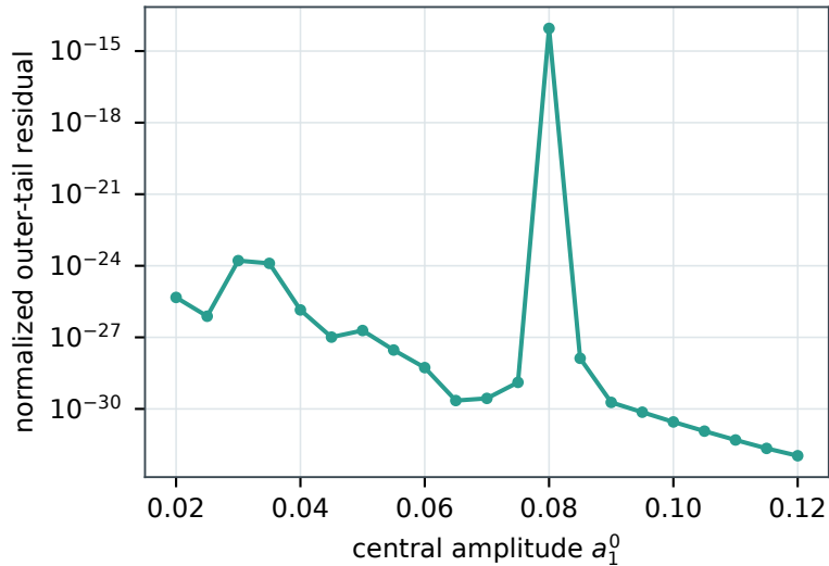
Massive-field Robin condition
