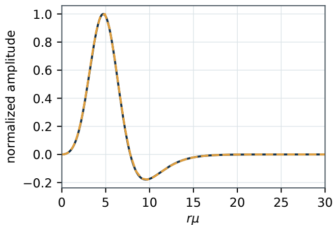
Overtone: metric field
