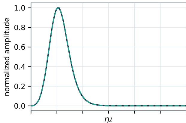
Overtone: metric field
