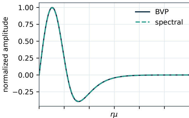
Overtone: scalar field (one node)
