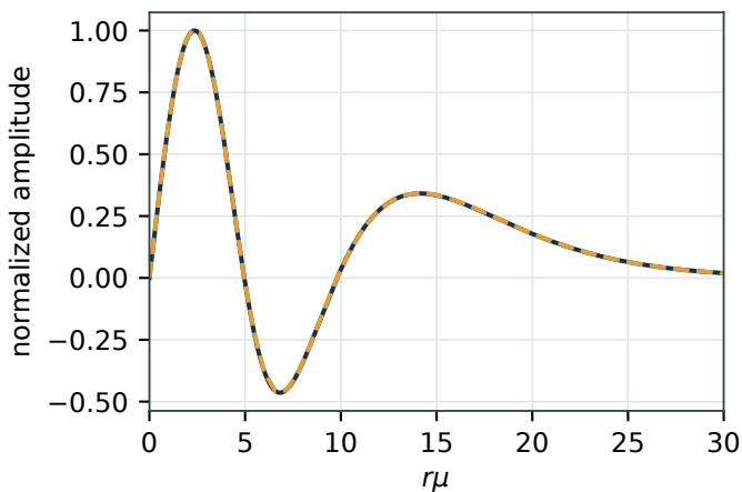
Overtone: scalar field (one node)
