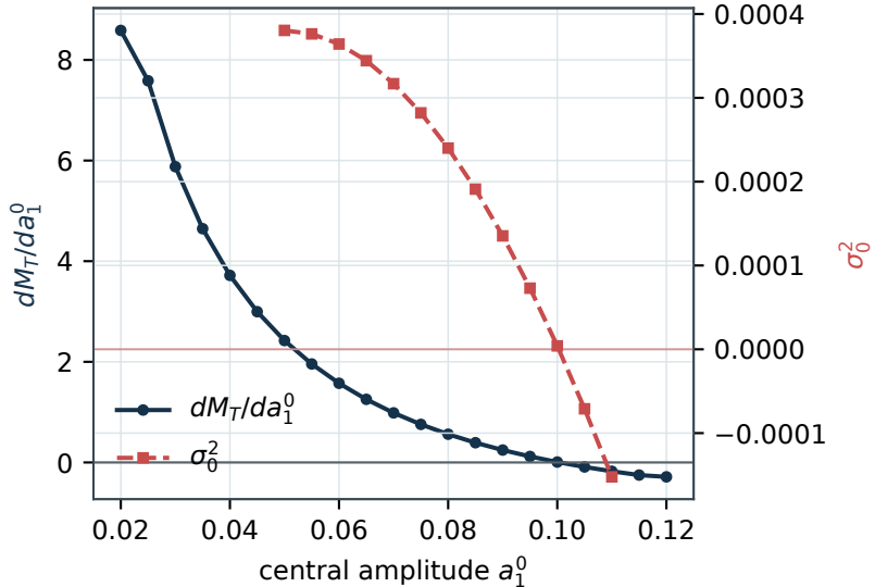
Turning point and radial eigenvalue
