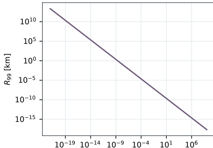
Quantum-gravity and charge scales
