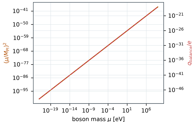
Quantum-gravity and charge scales
