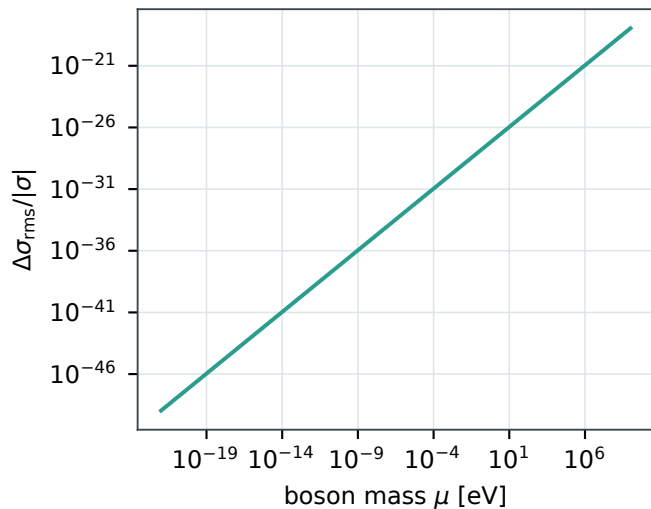
Coherent occupation dispersion
