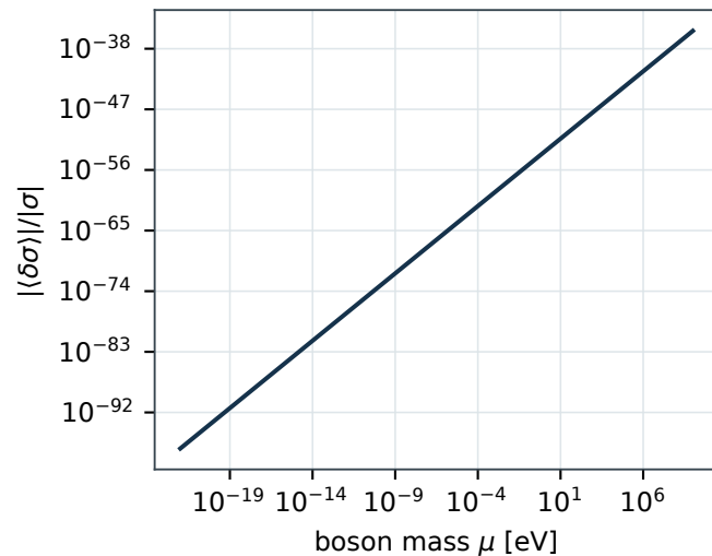
Mean occupation-noise bias
