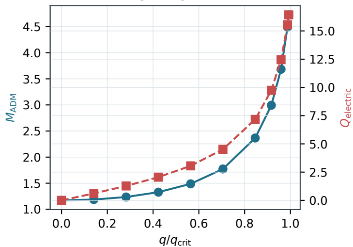
Backreacting charged continuation
