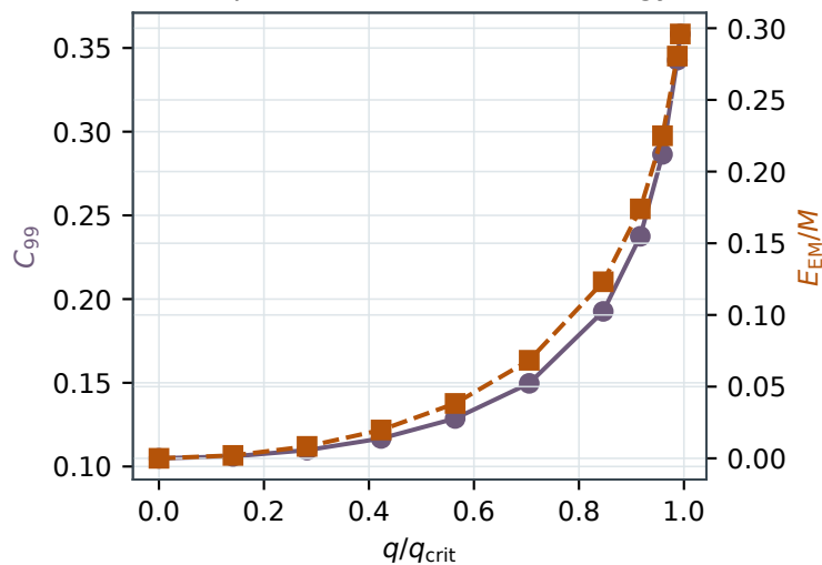
Compactness and Maxwell energy
