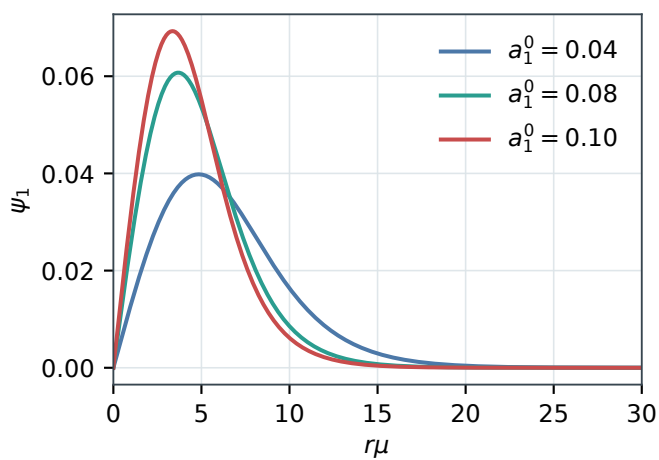
Representative relativistic \ell = 1 boson-star backgrounds
