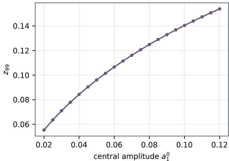
Redshift at the 99% mass radius
