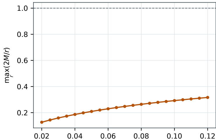
Exterior curvature proxy
