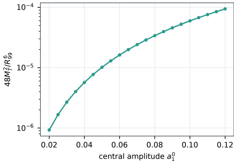
Exterior curvature proxy
