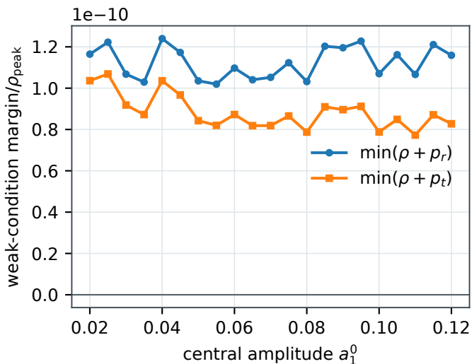
Weak energy-condition margins
