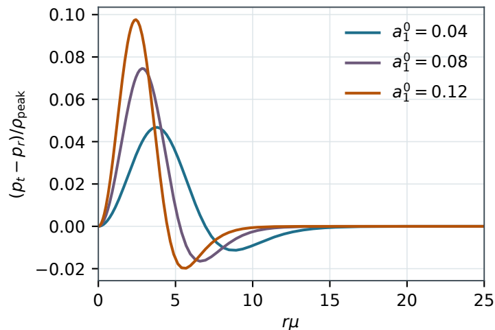
Pressure anisotropy
