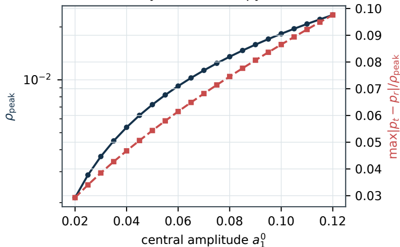
Density and anisotropy scale
