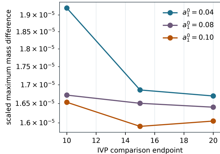
Independent integration: metric sector
