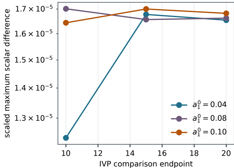
Independent integration: scalar sector
