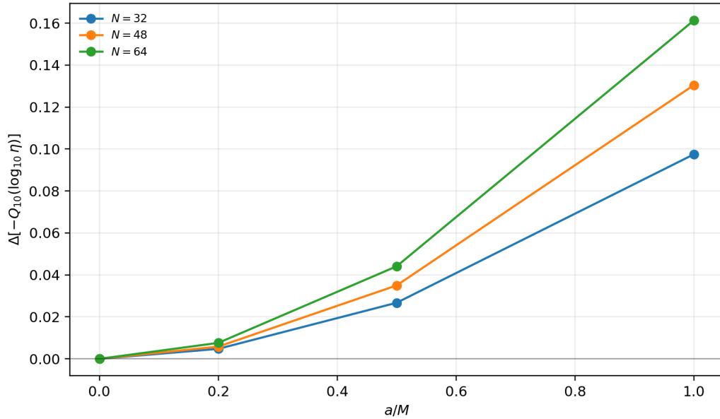
Fig. 7 Finite- N check for the scalar \ell = 2, n = 0 singular-value pseudospectral trend. The plotted quantity is the increase in -Q_{10}(\log_{10} \eta_N) relative to the Schwarzschild value at the same N . The monotonic increase with a/M is stable for N = 32, 48, 64 , although the absolute contour levels remain resolution dependent.
