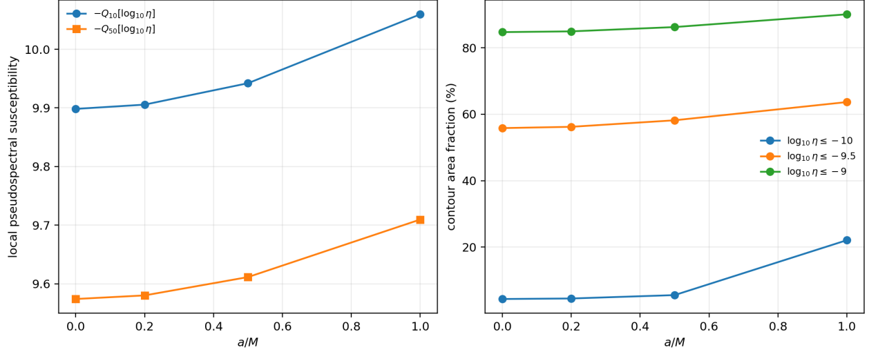
Fig. 6 Scalar \ell = 2, n = 0 singular-value pseudospectral sensitivity diagnostics at N = 64 . Left: quantile-based susceptibility measures increase with a/M . Right: fixed-threshold contour area fractions also grow; the deepest endpoint contour is window-limited and is used only as a local diagnostic.
