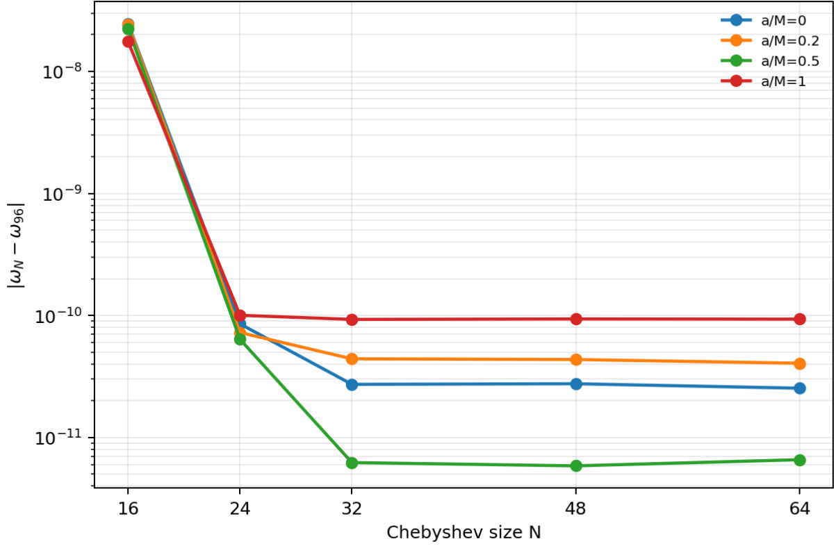
Fig. 1 Chebyshev convergence of the direct spectral fundamental branches. The vertical axis shows |\omega_N - \omega_{96}| for N = 16, 24, 32, 48, 64 , using the N = 96 value at the same a/M as the reference. The error drops rapidly between N = 16 and N = 24 and then reaches a high- N plateau, consistent with the large condition numbers reported in Table 5.
