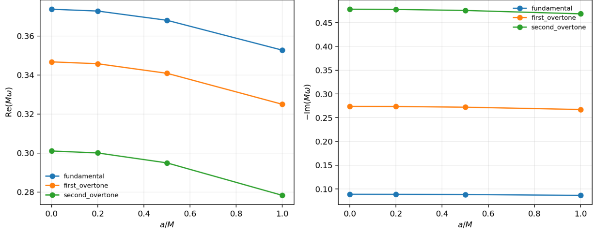
Fig. 2 Representative lapse-deformed axial-gravitational \ell = 2 mode trajectories versus a/M . These curves are trend diagnostics for the phenomenological axial model.
