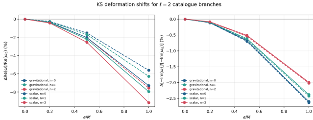
Fig. 3 Schwarzschild-relative endpoint trends for the \ell = 2 catalogue branches. Solid curves show scalar modes and dashed curves show the lapse-deformed axial gravitational model. The real-frequency shifts dominate the damping shifts, and all branches move downward over the sampled deformation range.
