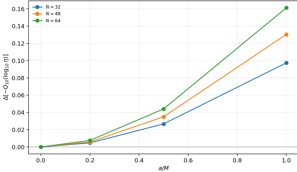
Figure 7 Finite- N check for the scalar \ell = 2, n = 0 singular-value pseudospectral trend. The plotted quantity is the increase in -Q_{10}(\log_{10} \eta_N) relative to the Schwarzschild value at the same N . The monotonic increase with a/M is stable for N = 32, 48, 64 , although the absolute contour levels remain resolution dependent.
