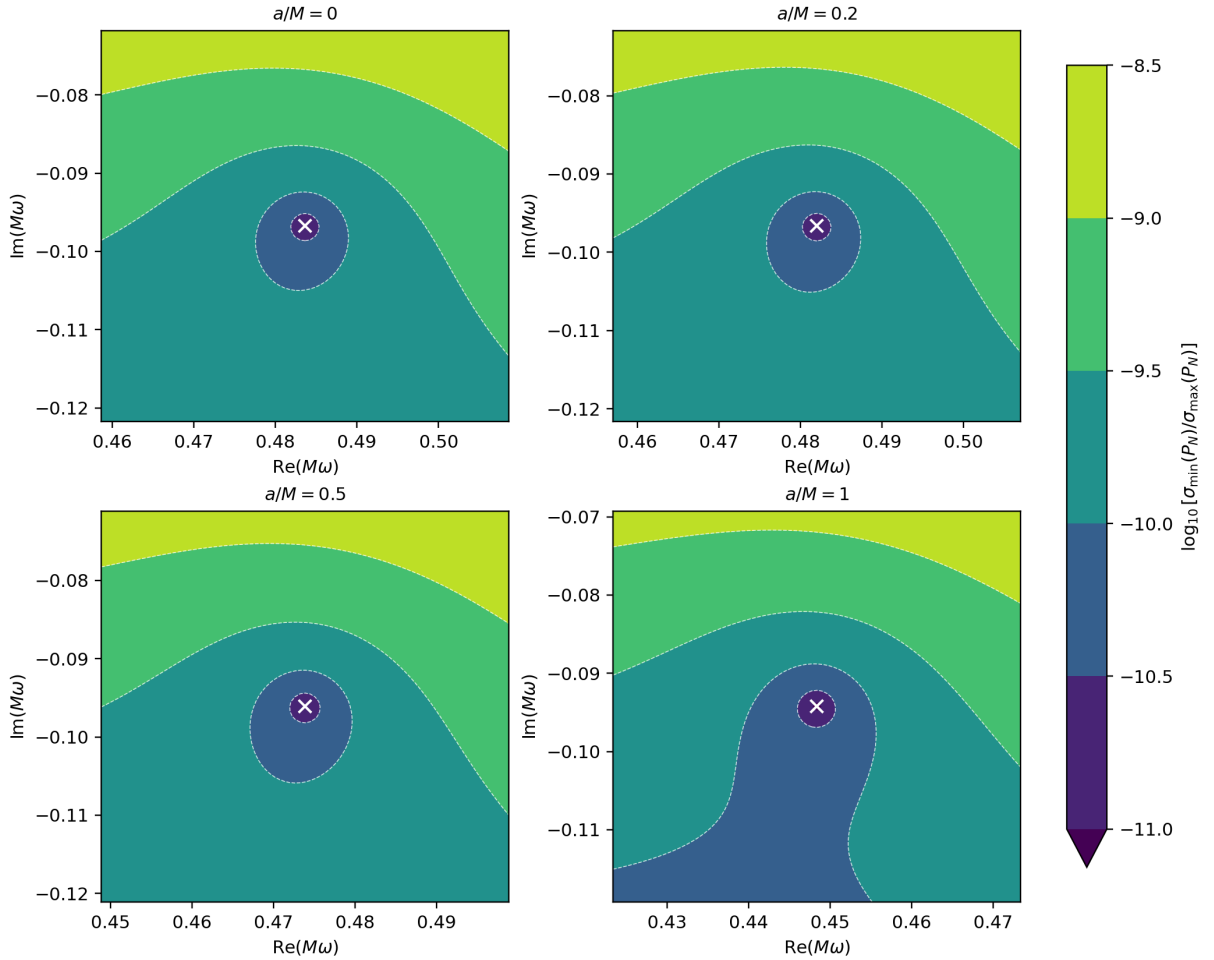
Figure 5 Finite-dimensional scalar \ell = 2, n = 0 singular-value pseudospectral contours for the relative residual \eta_N = \sigma_{\min}(P_N)/\sigma_{\max}(P_N) at N = 64 . White crosses mark the residual-minimized QNM locations. The panels show that the local small- \eta_N basin broadens as a/M increases.
