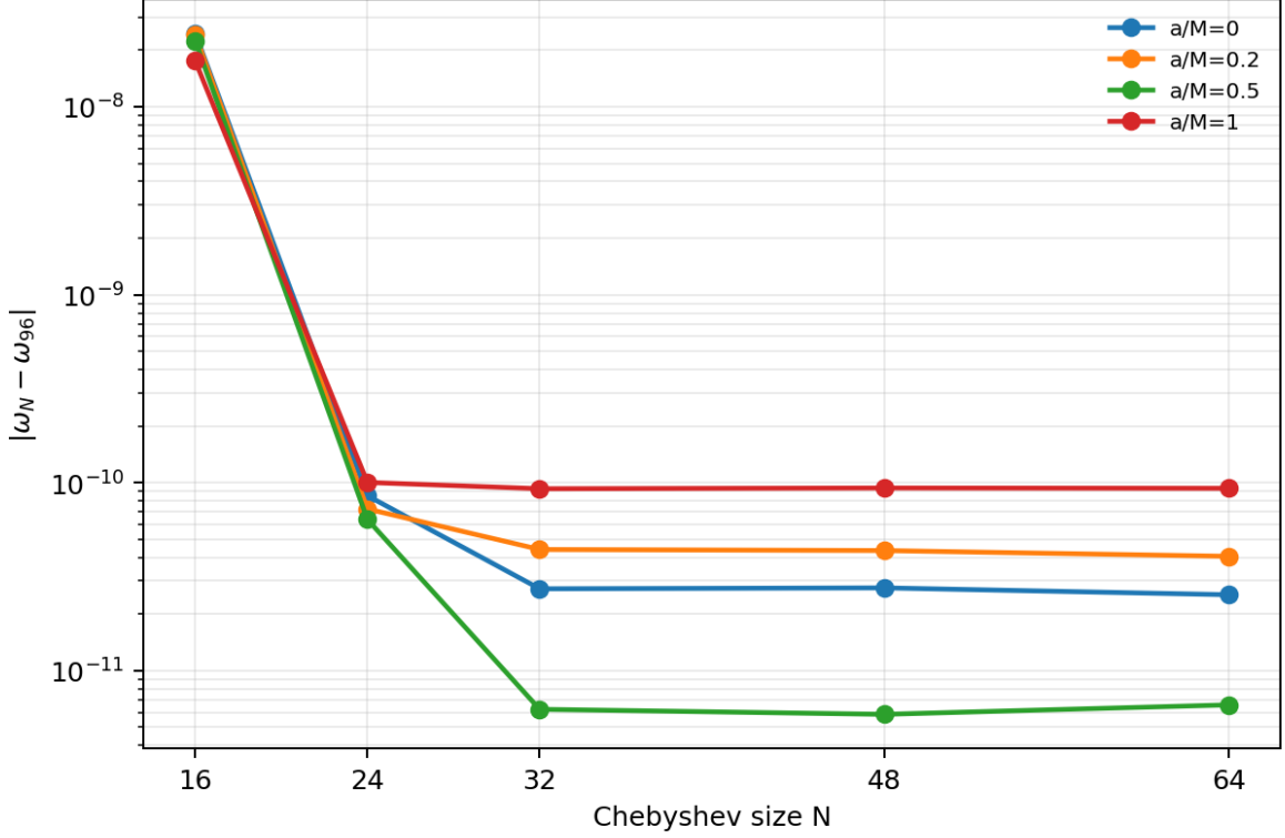
Figure 1 Chebyshev convergence of the direct spectral fundamental branches. The vertical axis shows |\omega_N - \omega_{96}| for N = 16, 24, 32, 48, 64 , using the N = 96 value at the same a/M as the reference. The error drops rapidly between N = 16 and N = 24 and then reaches a high- N plateau, consistent with the large condition numbers reported in Table 5.
