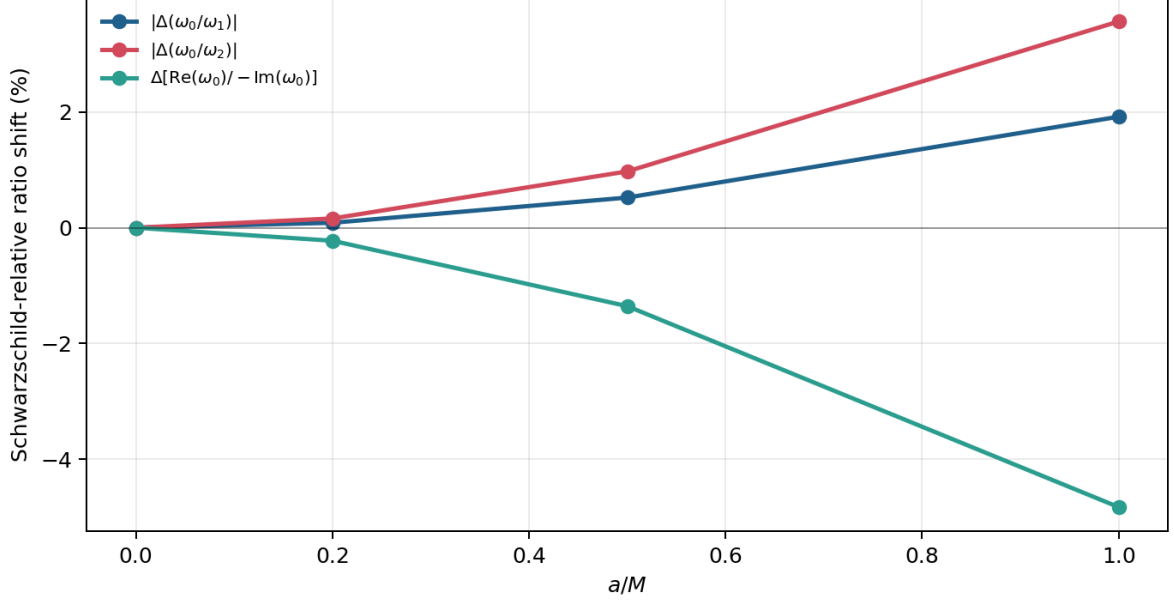
Figure 4 Scalar \ell = 2 dimensionless spectroscopy diagnostics. The plot shows Schwarzschild-relative changes in \omega_0/\omega_1 , \omega_0/\omega_2 , and \text{Re}(\omega_0)/[-\text{Im}(\omega_0)] . These ratios do not by themselves constitute an observational forecast, but they are closer to spectroscopy observables than individual mode frequencies because they reduce simple mass-scaling degeneracy.
