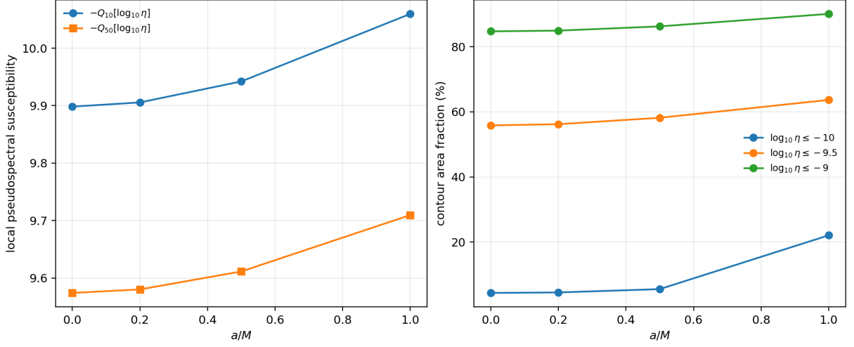
Figure 6 Scalar \ell = 2, n = 0 singular-value pseudospectral sensitivity diagnostics at N = 64 . Left: quantile-based susceptibility measures increase with a/M . Right: fixed-threshold contour area fractions also grow; the deepest endpoint contour is window-limited and is used only as a local diagnostic.
