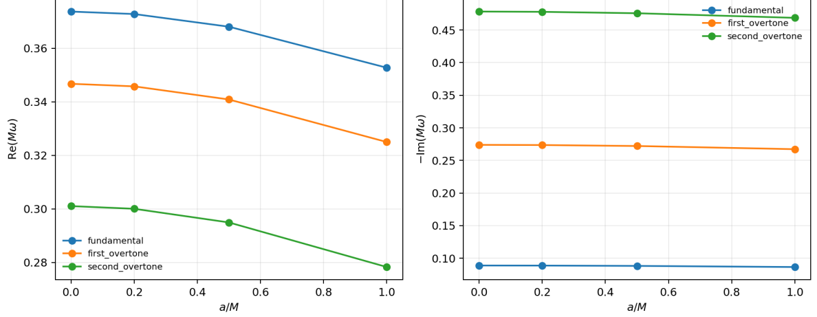
Figure 2 Representative lapse-deformed axial-gravitational \ell = 2 mode trajectories versus a/M . These curves are trend diagnostics for the phenomenological axial model.
