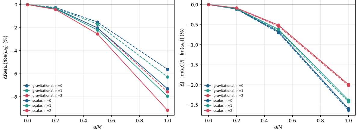
Figure 3 Schwarzschild-relative endpoint trends for the \ell = 2 catalogue branches. Solid curves show scalar modes and dashed curves show the lapse-deformed axial gravitational model. The real-frequency shifts dominate the damping shifts, and all branches move downward over the sampled deformation range.
