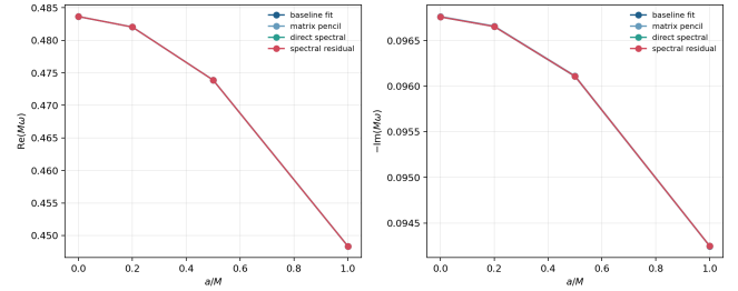
Fig. 5 Baseline and direct spectral deformation trends for the scalar \ell = 2 fundamental mode. The spectral operator reproduces the same qualitative decrease in oscillation frequency with increasing a/M , while avoiding the waveform-derived matrix surrogate.
