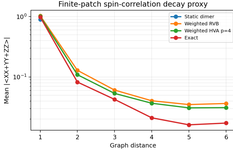
Figure 5: Finite-patch spin-correlation decay proxy. Correlations are averaged by graph distance because reliable physical coordinates for the extracted 19-site patch are not part of the input data. The static dimer has only nearest-neighbor singlet correlations, while the weighted-RVB and HVA-refined states show distributed short-range correlations closer to the exact-state pattern.
