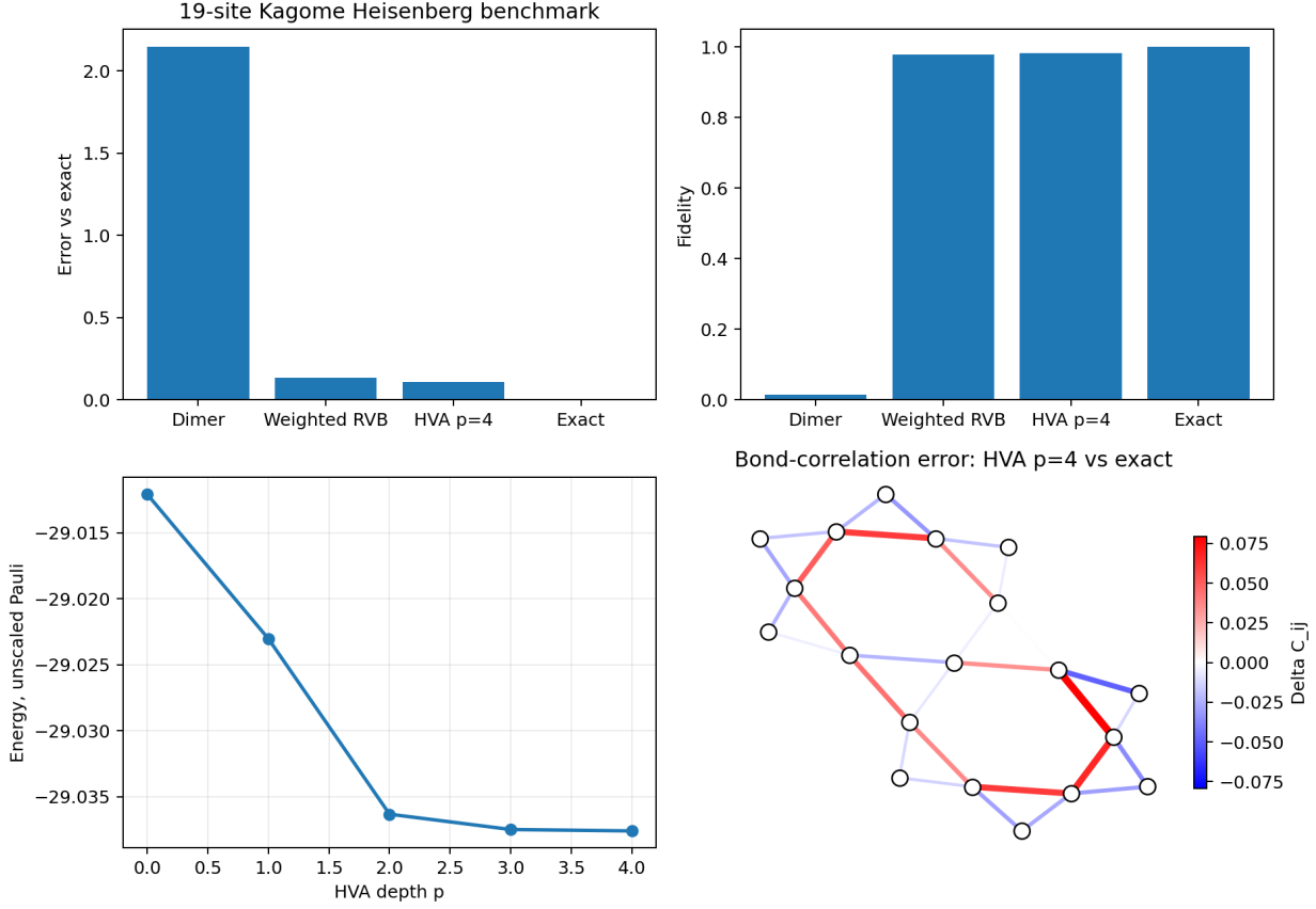
Figure 2: One-page summary of the 19-site benchmark. The weighted-RVB initializer dramatically improves on the static dimer product state, and Heisenberg-HVA refinement gives a smaller but consistent no-calibration improvement through p = 4 .
