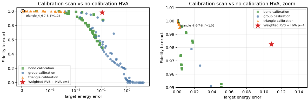
Figure 9: Calibration scan landscape. Left means lower target-energy error and up means higher exact-state fidelity, so the upper-left corner is best. The colored points are exact ground states of modified Hamiltonians; the red star is the present no-calibration weighted-RVB + HVA p = 4 result. The figure motivates calibration-informed ansatz design, not a claim that the current HVA already outperforms calibrated reference states.
