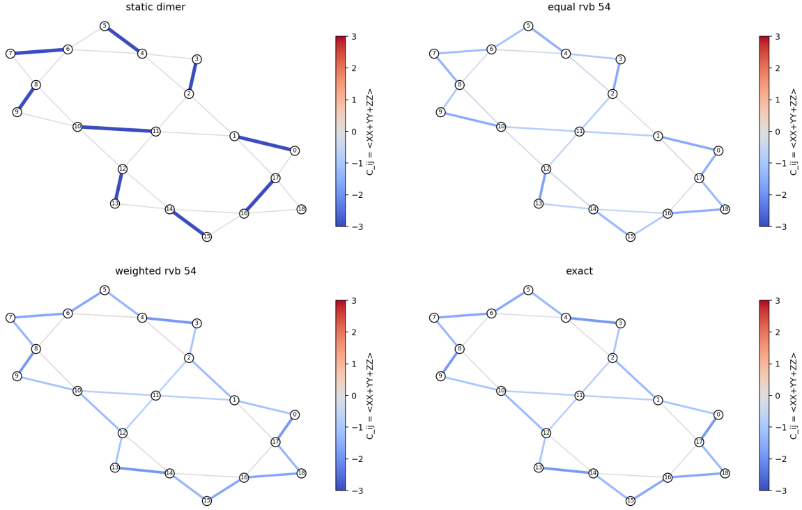
Figure 6: Bond correlations for the static dimer baseline, equal RVB, weighted RVB, and exact state. The weighted-RVB state captures the exact correlation pattern much better than either the static product state or equal positive RVB.
