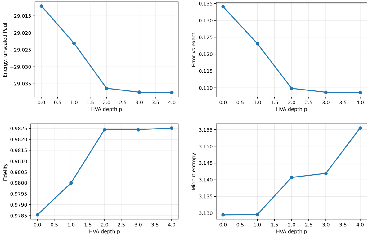
Figure 3: Depth dependence of energy, error, fidelity, and entropy. The largest improvement comes from weighted-RVB initialization; HVA layers provide a smaller additional circuit-compatible refinement.
