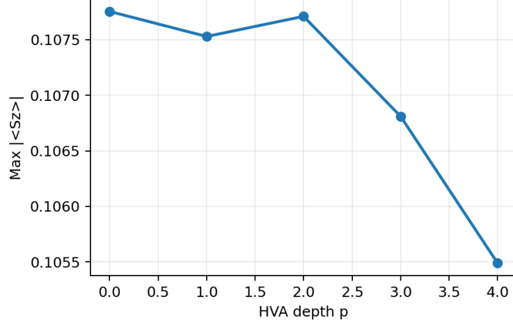
Figure 4: Maximum site magnetization versus HVA depth. The weighted RVB and HVA-refined states remain much closer to the low-magnetization exact state than the static dimer baseline.
