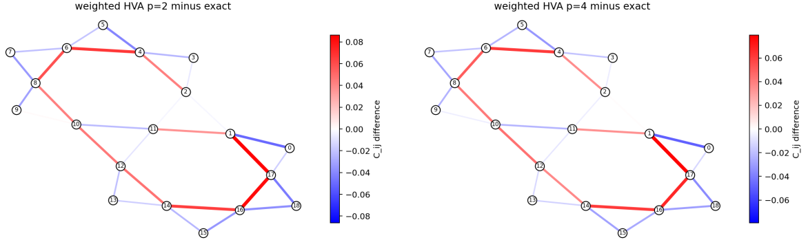
Figure 8: Bond-correlation error maps relative to the exact state. Left: earlier p = 2 HVA reference. Right: best current no-calibration HVA, p = 4 .
