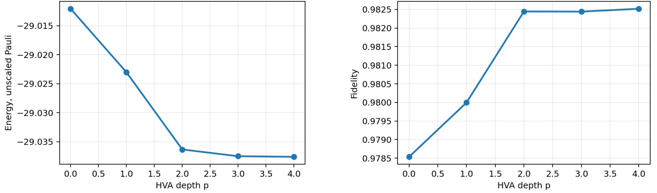
Figure 3: Energy and fidelity versus HVA depth after weighted-RVB initialization. Energy improves most through p = 2 and then begins to saturate, while fidelity remains high.
