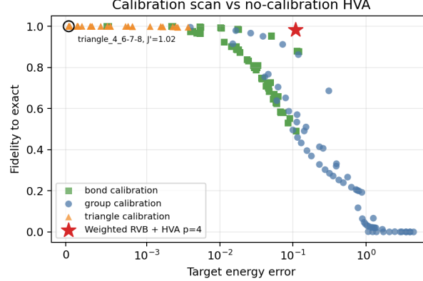
Figure 4: Calibration scan landscape compared with the no-calibration HVA baseline. These exact reference states are interpreted here as guidance for future ansatz design, not as a replacement for the no-calibration circuit workflow.
