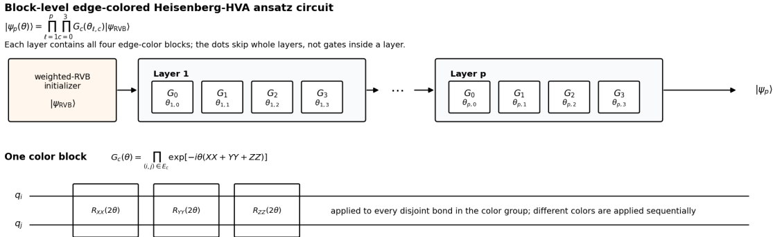
Figure 2: Block-level edge-colored Heisenberg-HVA ansatz circuit. The weighted-RVB initializer is followed by repeated color blocks G_c(\theta_{\ell,c}) . Each G_c block represents several parallel two-qubit Heisenberg interactions on disjoint bonds, decomposed into Qiskit Pauli rotation gates R_{XX}(2\theta) , R_{YY}(2\theta) , and R_{ZZ}(2\theta) . A full 19-qubit gate-level circuit would contain 120 Heisenberg bond gates, or 360 R_{XX}/R_{YY}/R_{ZZ} rotations, for the p = 4 run, so the full gate-level diagram is omitted for readability.
