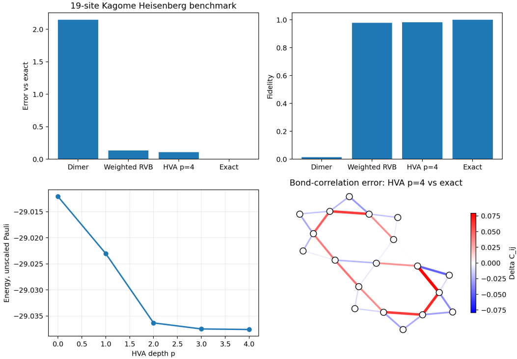
Figure 2: Compact summary of the current finite-size proof-of-concept. Weighted-RVB gives the main jump in quality; shallow Heisenberg-HVA layers add no-calibration refinement.
