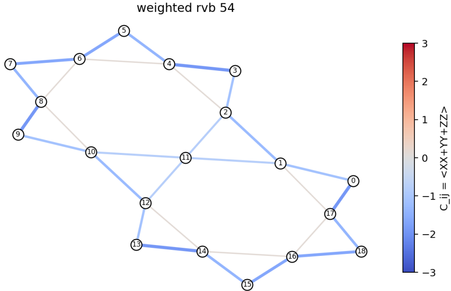
Figure 1: Bond-correlation map for the weighted-RVB initializer. This finite-patch diagnostic shows that antiferromagnetic correlations are distributed over the graph rather than frozen onto one dimer covering.
