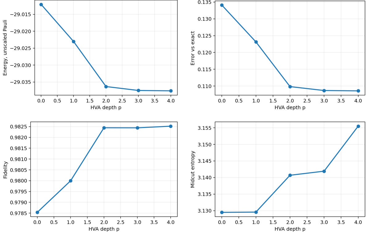
Figure 4: Depth dependence of energy, error, fidelity, and entropy. The largest improvement comes from weighted-RVB initialization; HVA layers provide a smaller additional circuit-compatible refinement.
