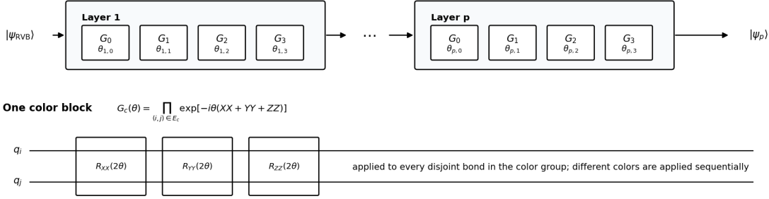
Figure 2: Edge-colored Heisenberg-HVA ansatz circuit. The weighted-RVB initializer is followed by repeated color blocks G_c(\theta_{\ell,c}) . Each color block is a product of disjoint two-qubit Heisenberg interactions, decomposed into Qiskit Pauli rotation gates R_{XX}(2\theta) , R_{YY}(2\theta) , and R_{ZZ}(2\theta) .
