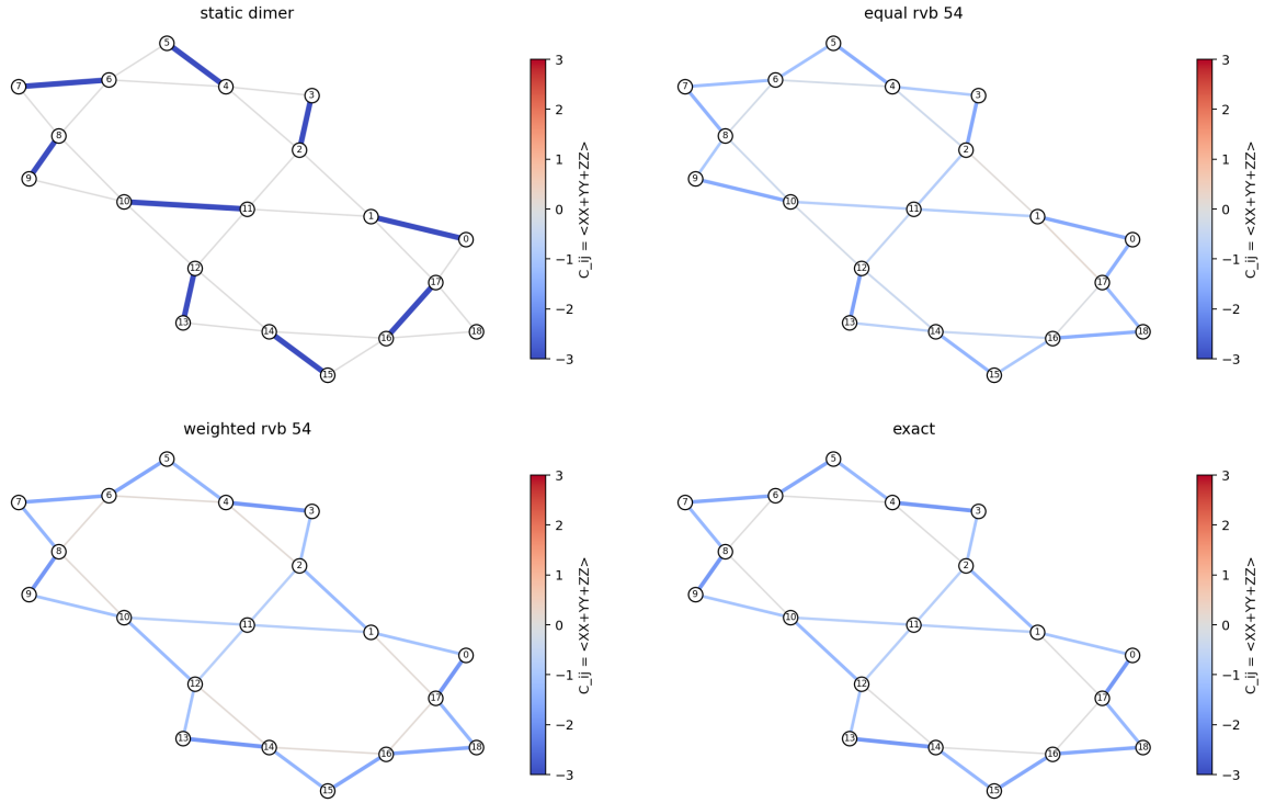
Figure 7: Bond correlations for the static dimer baseline, equal RVB, weighted RVB, and exact state. The weighted-RVB state captures the exact correlation pattern much better than either the static product state or equal positive RVB.
