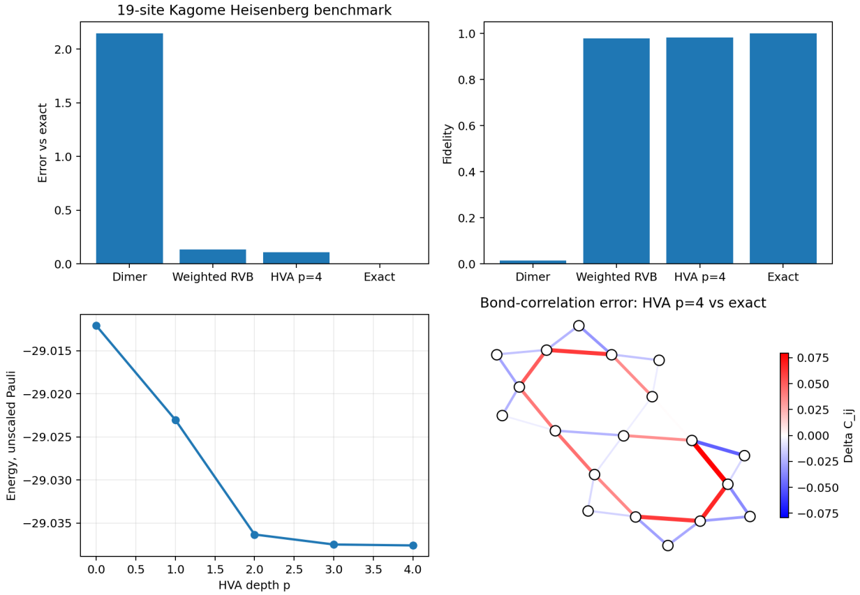
Figure 3: One-page summary of the 19-site benchmark. The weighted-RVB initializer dramatically improves on the static dimer product state, and Heisenberg-HVA refinement gives a smaller but consistent no-calibration improvement through p = 4 .
