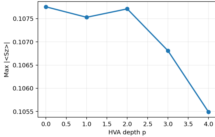
Figure 5: Maximum site magnetization versus HVA depth. The weighted RVB and HVA-refined states remain much closer to the low-magnetization exact state than the static dimer baseline.
