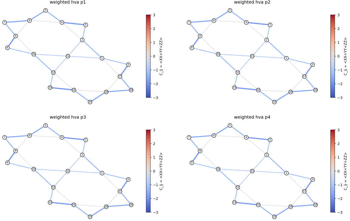
Figure 8: Bond-correlation maps after HVA refinement at p = 1, 2, 3, 4 . Refinement is incremental but consistently preserves the distributed antiferromagnetic structure of the weighted-RVB initializer.
