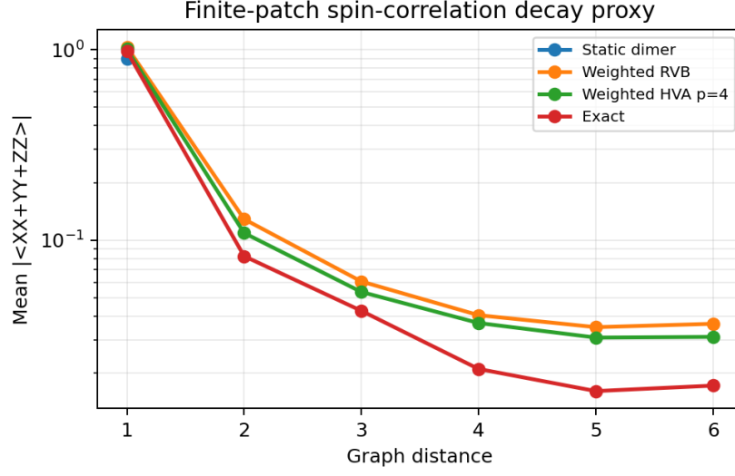
Figure 6: Finite-patch spin-correlation decay proxy. Correlations are averaged by graph distance because reliable physical coordinates for the extracted 19-site patch are not part of the input data. The static dimer has only nearest-neighbor singlet correlations, while the weighted-RVB and HVA-refined states show distributed short-range correlations closer to the exact-state pattern.
