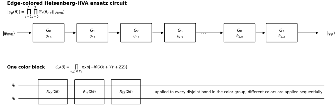
Figure 2: Edge-colored Heisenberg-HVA ansatz circuit. The weighted-RVB initializer is followed by repeated color blocks G_c(\theta_{\ell,c}) . Each color block is a product of disjoint two-qubit Heisenberg interactions, decomposed into Qiskit Pauli rotation gates R_{XX}(2\theta) , R_{YY}(2\theta) , and R_{ZZ}(2\theta) .
