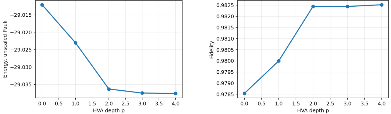
Figure 5: Energy and fidelity versus HVA depth after weighted-RVB initialization. Energy improves most through p = 2 and then begins to saturate, while fidelity remains high.
