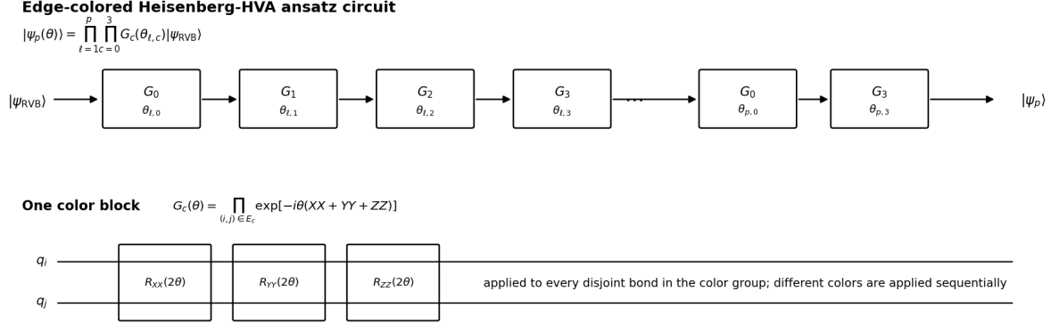
Figure 3: Ansatz circuit used after weighted-RVB initialization. A depth- p HVA applies four edge-color blocks per layer. Each block uses one shared parameter and applies Qiskit two-qubit Pauli rotations on every disjoint bond in that color group.
