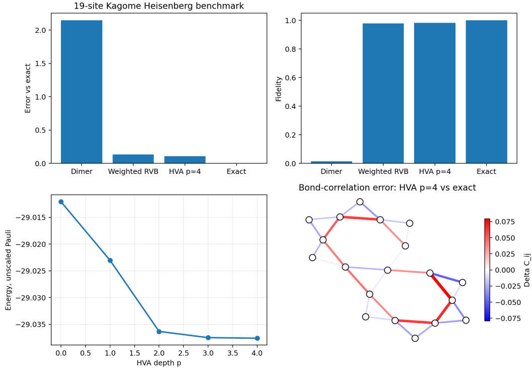
Figure 4: Compact summary of the current finite-size proof-of-concept. Weighted-RVB gives the main jump in quality; shallow Heisenberg-HVA layers add no-calibration refinement.
