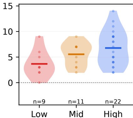
Mistral-7B-Instruct-v0.3
