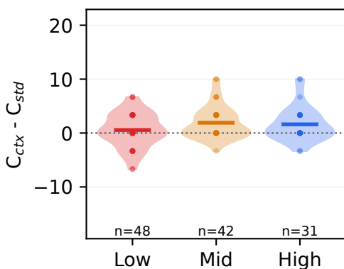
Llama-3.1-8B-Instruct
