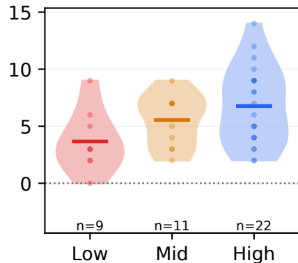
Mistral-7B-Instruct-v0.3
