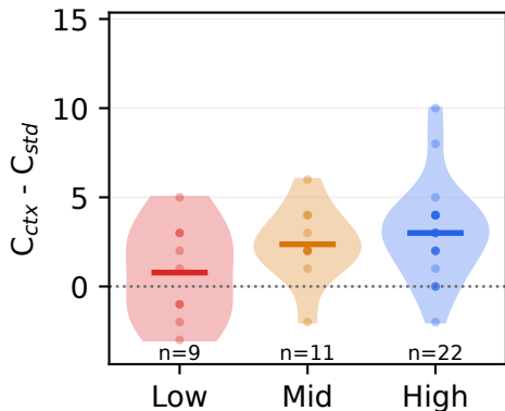
Llama-3.1-8B-Instruct
