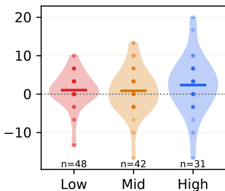
Mistral-7B-Instruct-v0.3
