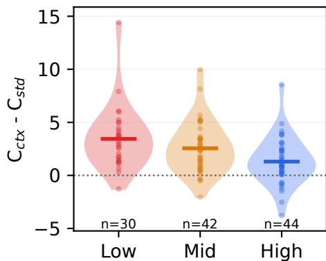
Llama-3.1-8B-Instruct
