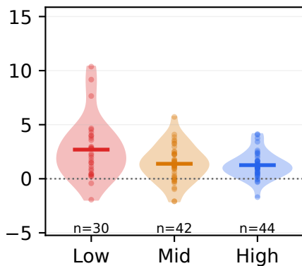
Mistral-7B-Instruct-v0.3
