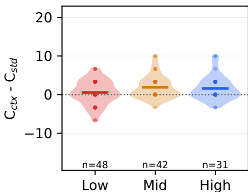
Llama-3.1-8B-Instruct
