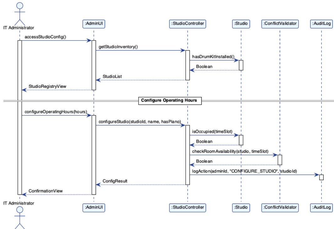
Figure 4.16: SSD-15 Configure Studio & Instrument Setup
