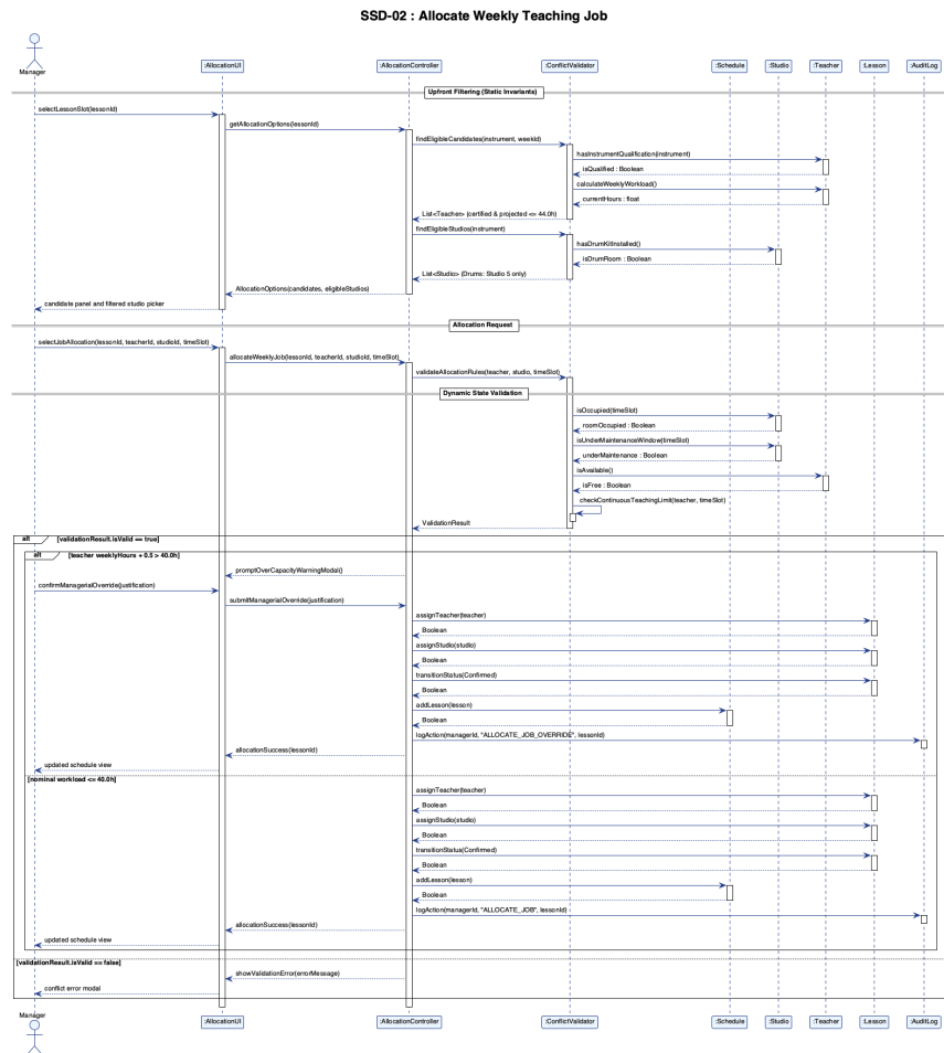
Figure 4.4: SSD-02 Allocate Weekly Teaching Job
