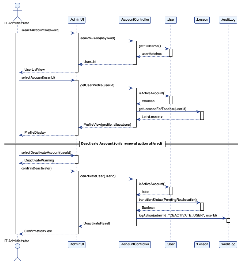
Figure 4.15: SSD-14 Manage User Account Status & Access
