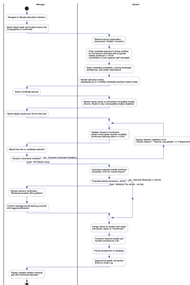
Figure 3.2: Activity Diagram for Weekly Job Allocation Workflow
