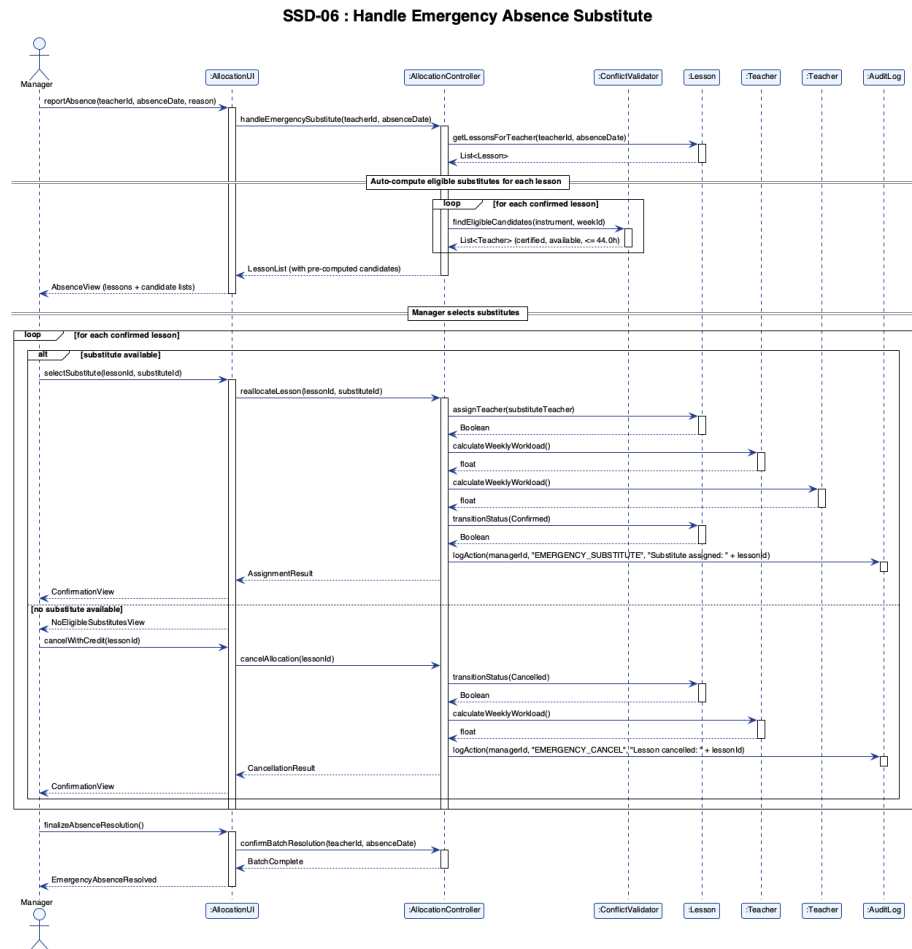
Figure 4.8: SSD-06 Handle Emergency Absence Substitute
