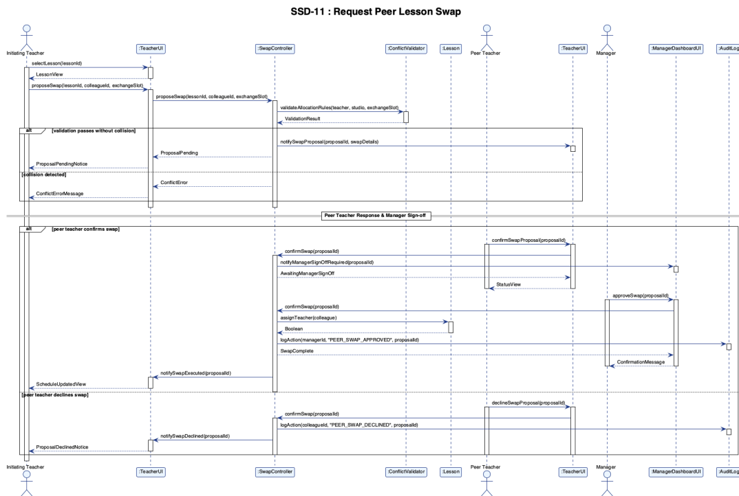
Figure 4.13: SSD-11 Request Peer Lesson Swap
