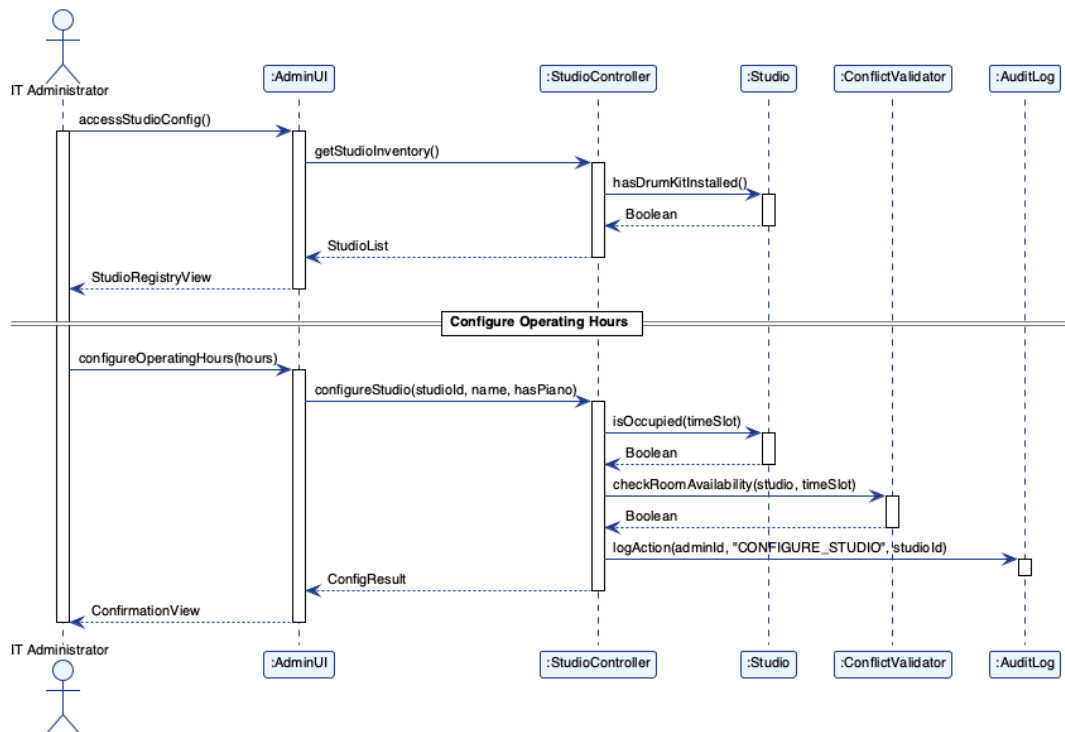
Figure 4.16: SSD-14 Configure Studio & Instrument Setup
