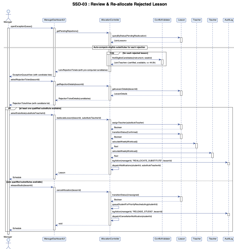
Figure 4.5: SSD-03 Review & Re-allocate Rejected Lesson
