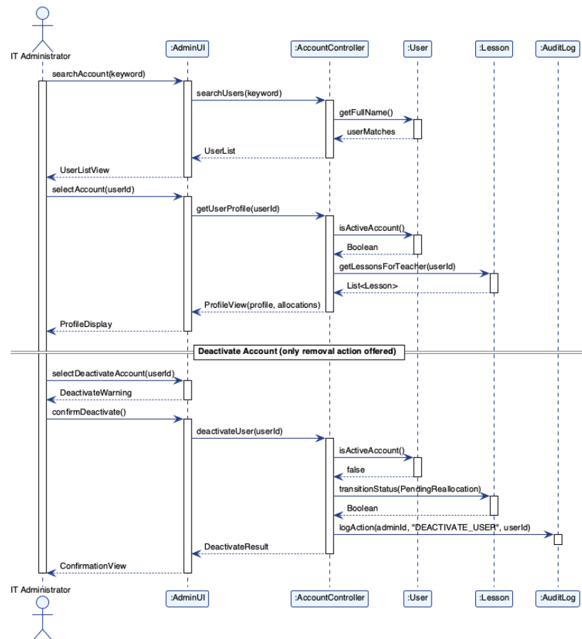
Figure 4.15: SSD-13 Manage User Account Status & Access
