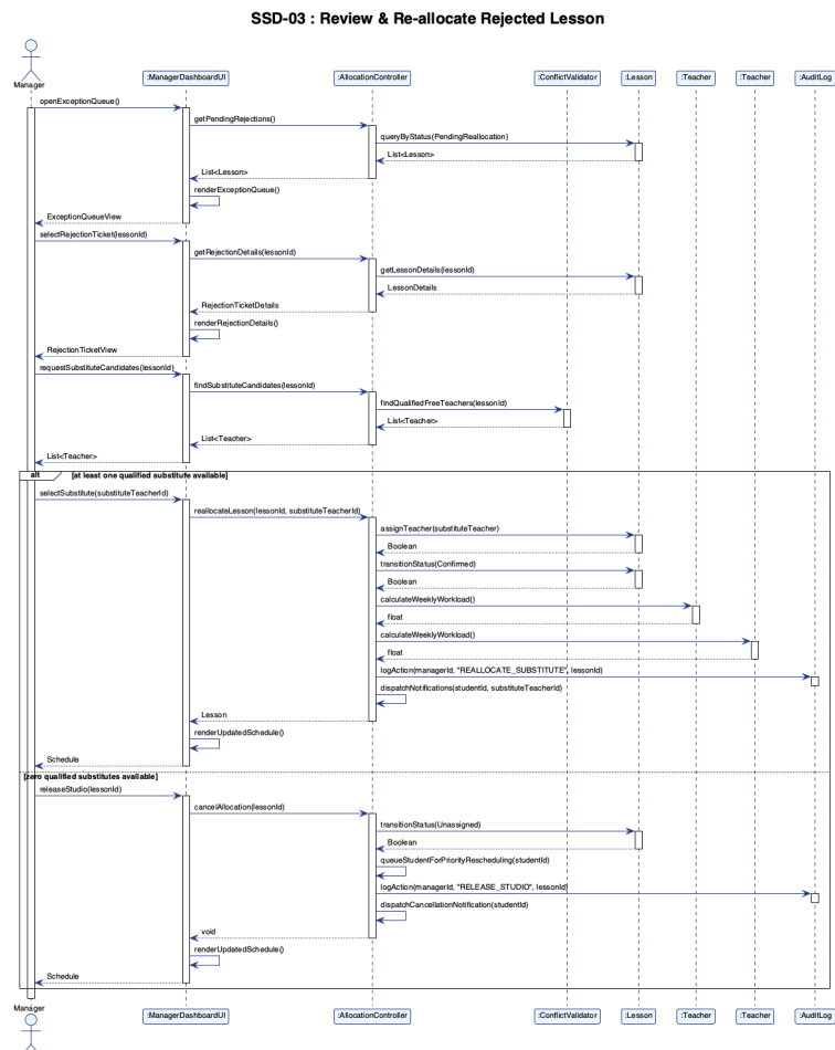
Figure 4.5: SSD-03 Review & Re-allocate Rejected Lesson
