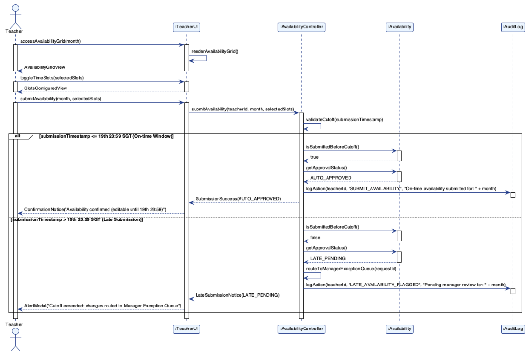
Figure 4.9: SSD-08 Submit Monthly Availability Window
