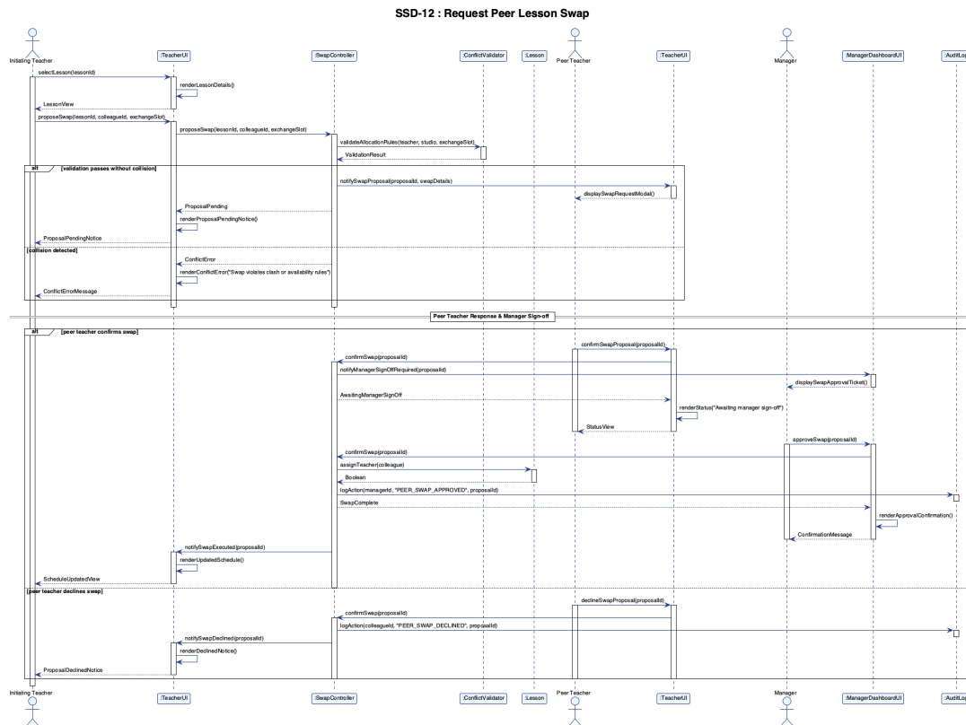
Figure 4.13: SSD-12 Request Peer Lesson Swap
