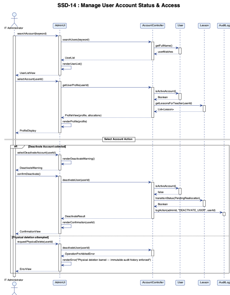
Figure 4.15: SSD-14 Manage User Account Status & Access
