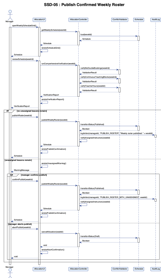
Figure 4.7: SSD-05 Publish Confirmed Weekly Roster
