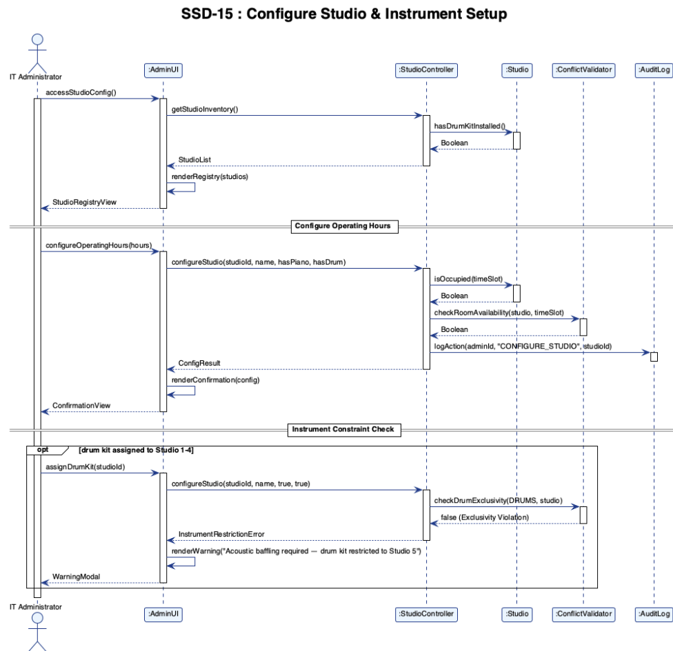
Figure 4.16: SSD-15 Configure Studio & Instrument Setup
