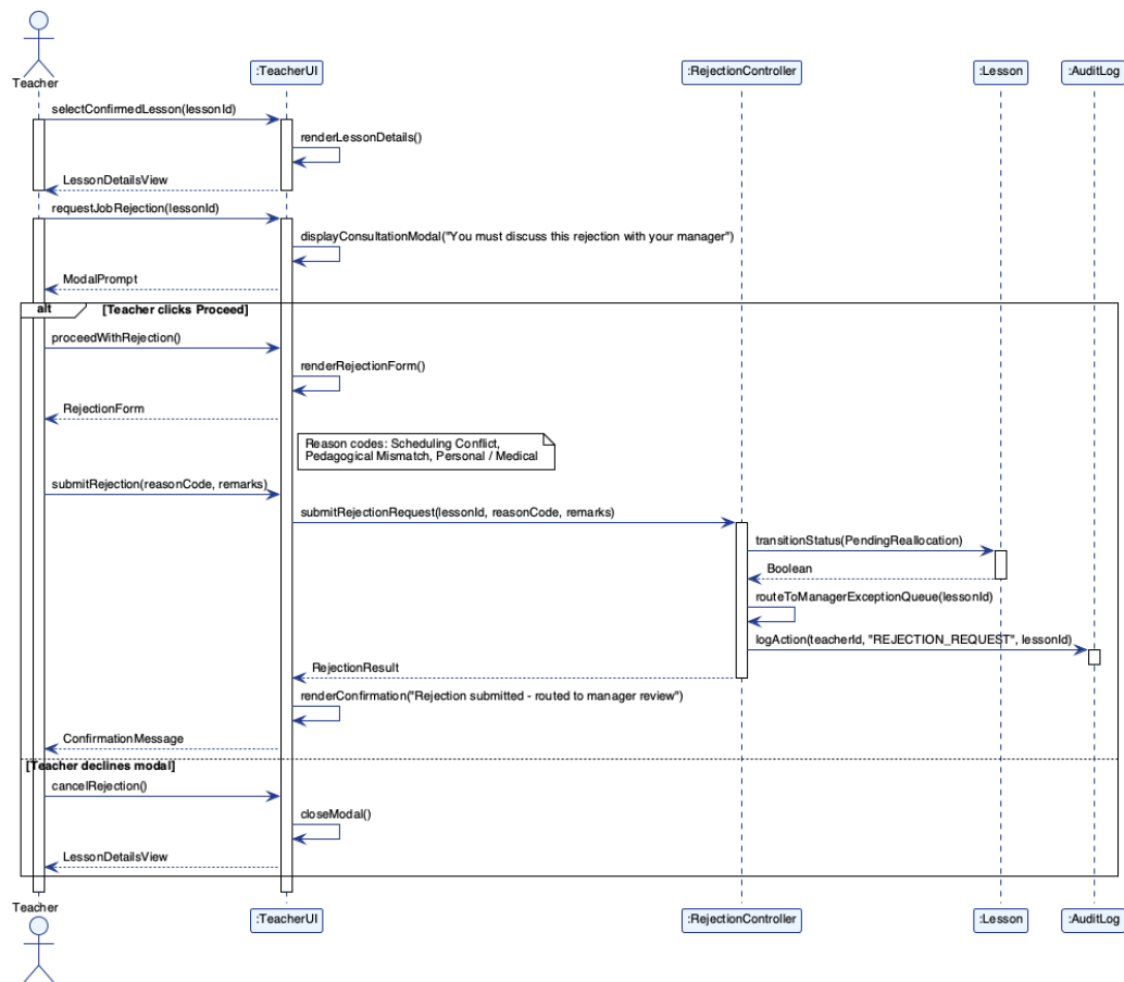
Figure 4.12: SSD-11 Submit Job Rejection Request
