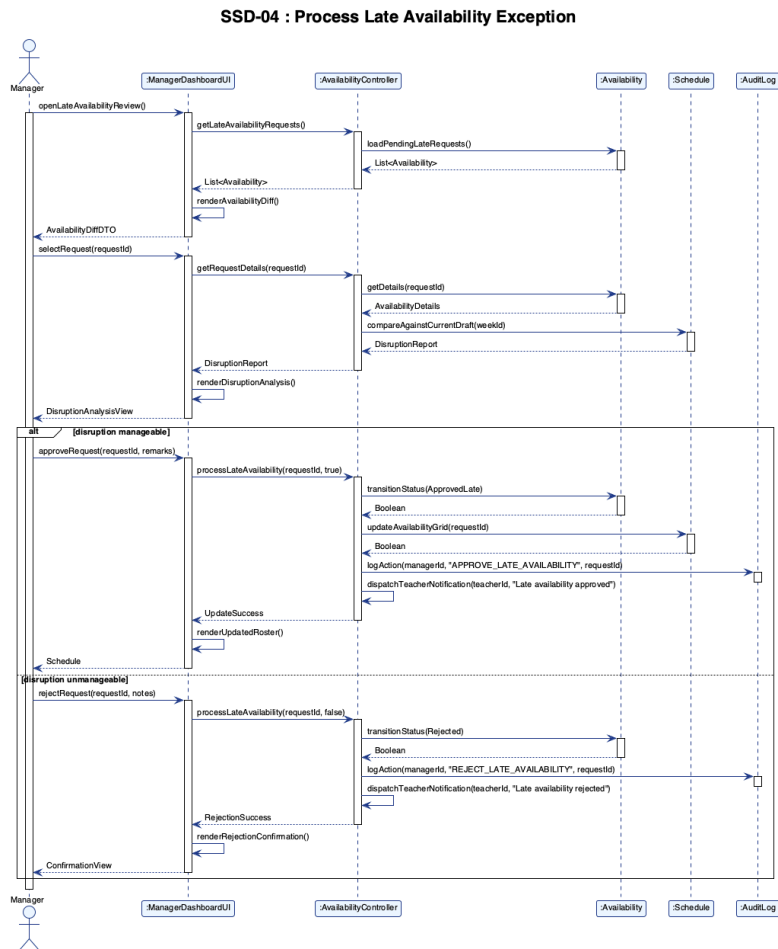
Figure 4.6: SSD-04 Process Late Availability Exception
