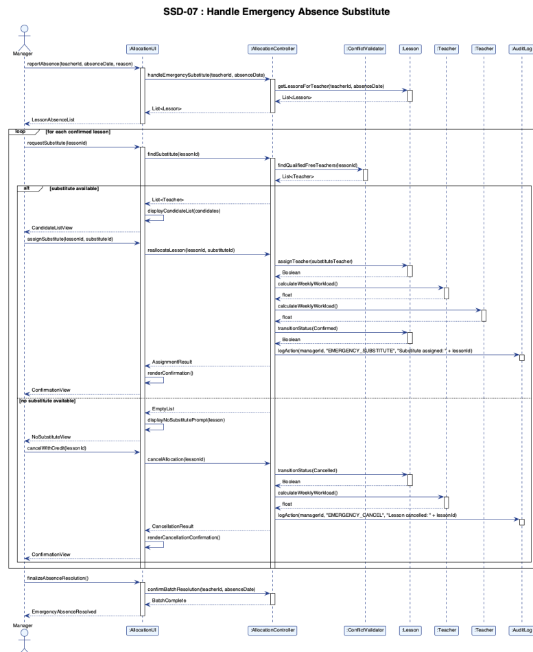
Figure 4.8: SSD-07 Handle Emergency Absence Substitute
