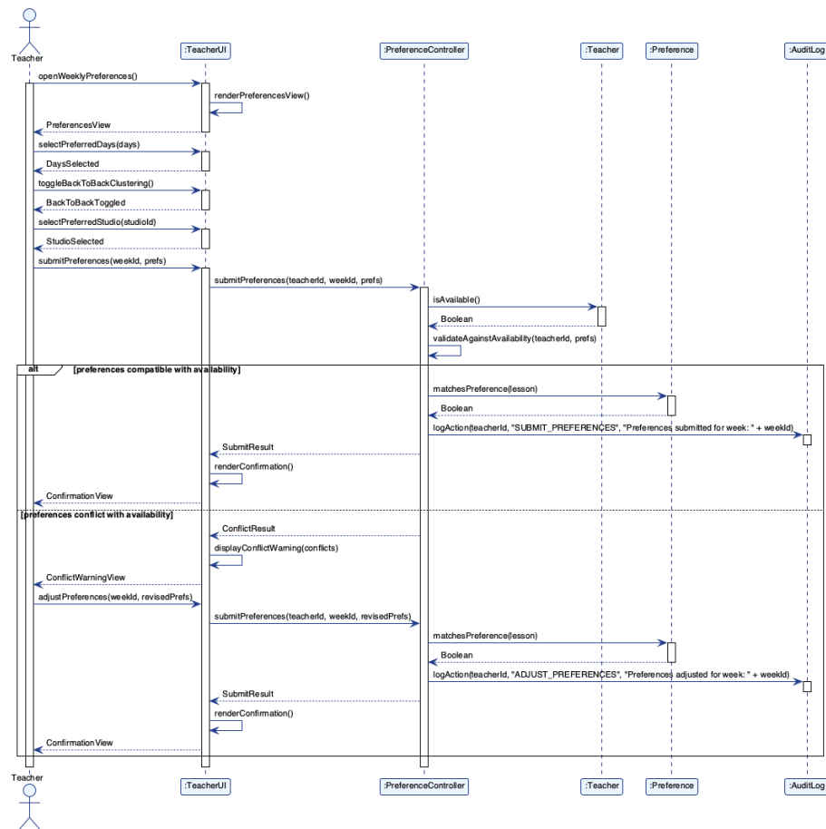
Figure 4.10: SSD-09 Submit Weekly Job Preferences
