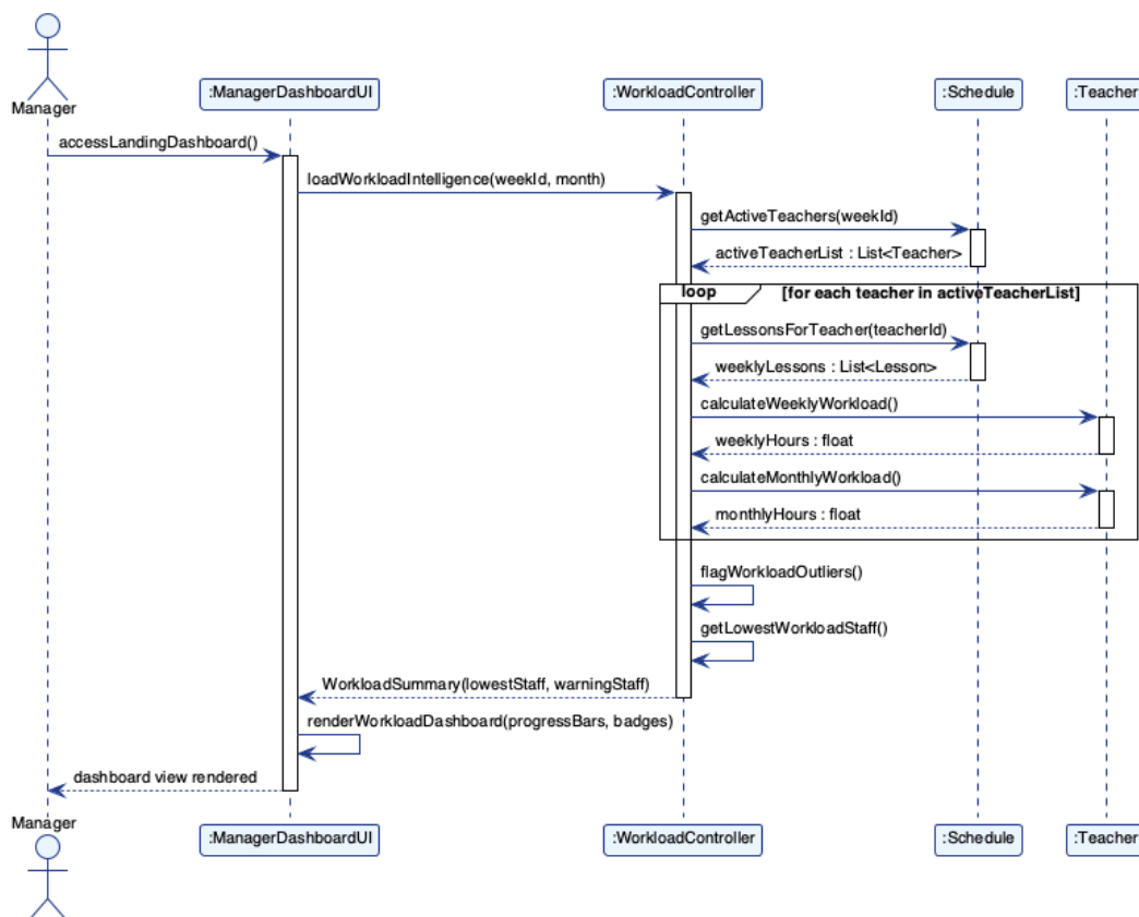
Figure 4.3: SSD-01 View Workload Dashboard & Outliers
