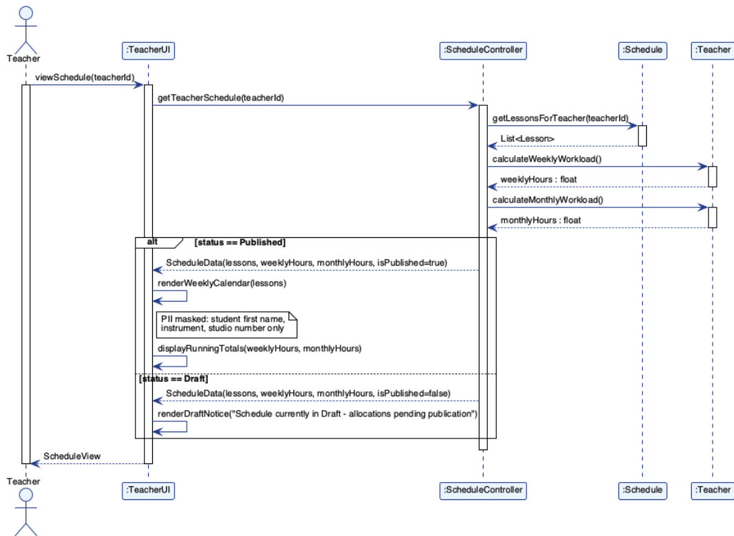
Figure 4.11: SSD-10 View Confirmed Schedule & Workload
