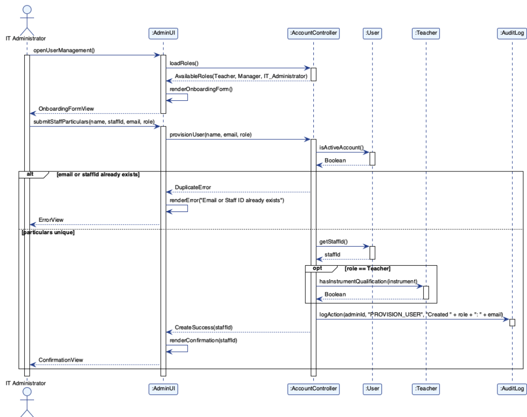
Figure 4.14: SSD-13 Onboard New Staff & Manager Accounts
