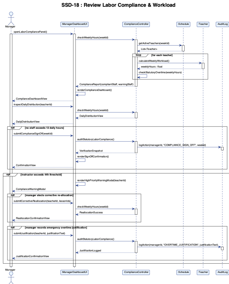
Figure 4.19: SSD-18 Review Labor Compliance & Workload
