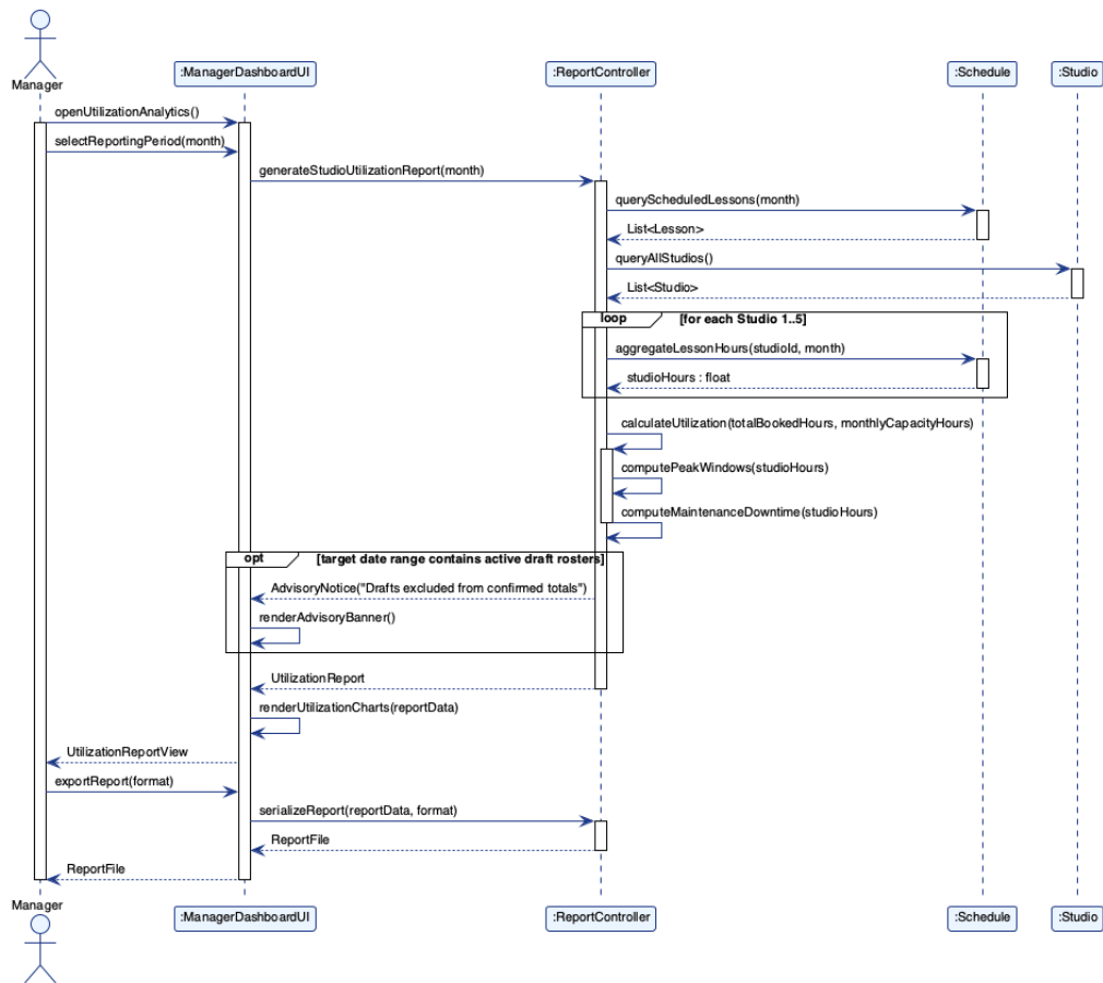
Figure 4.18: SSD-17 Generate Studio Utilization Report
